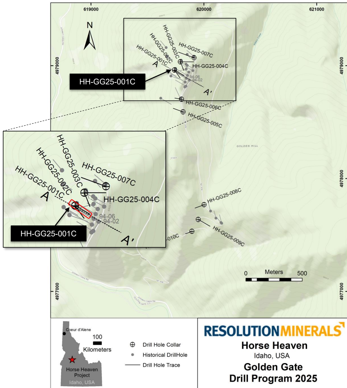
Figure 2: Drill hole location map of the Phase 1 Golden Gate drill program. HH-GG25-001C is located in the central northern part of the Golden Gate Target. INSERT: Enlarged part of the plan, included to show the details of the drill hole configuration in the vicinity of HH-GG25-001C. HH-GG25-001C is the first hole at Horse Heaven to properly test un-oxidised mineralisation. Shallow, pre-RML RC drill holes (grey hole traces) are also shown, including 94-02 and 94-06, which both appear in Figure 3. The drill hole parameters and summary mineralised interval of the pre-RML RC drill holes were provided to the market in ASX announcement dated 11 June 2025.
