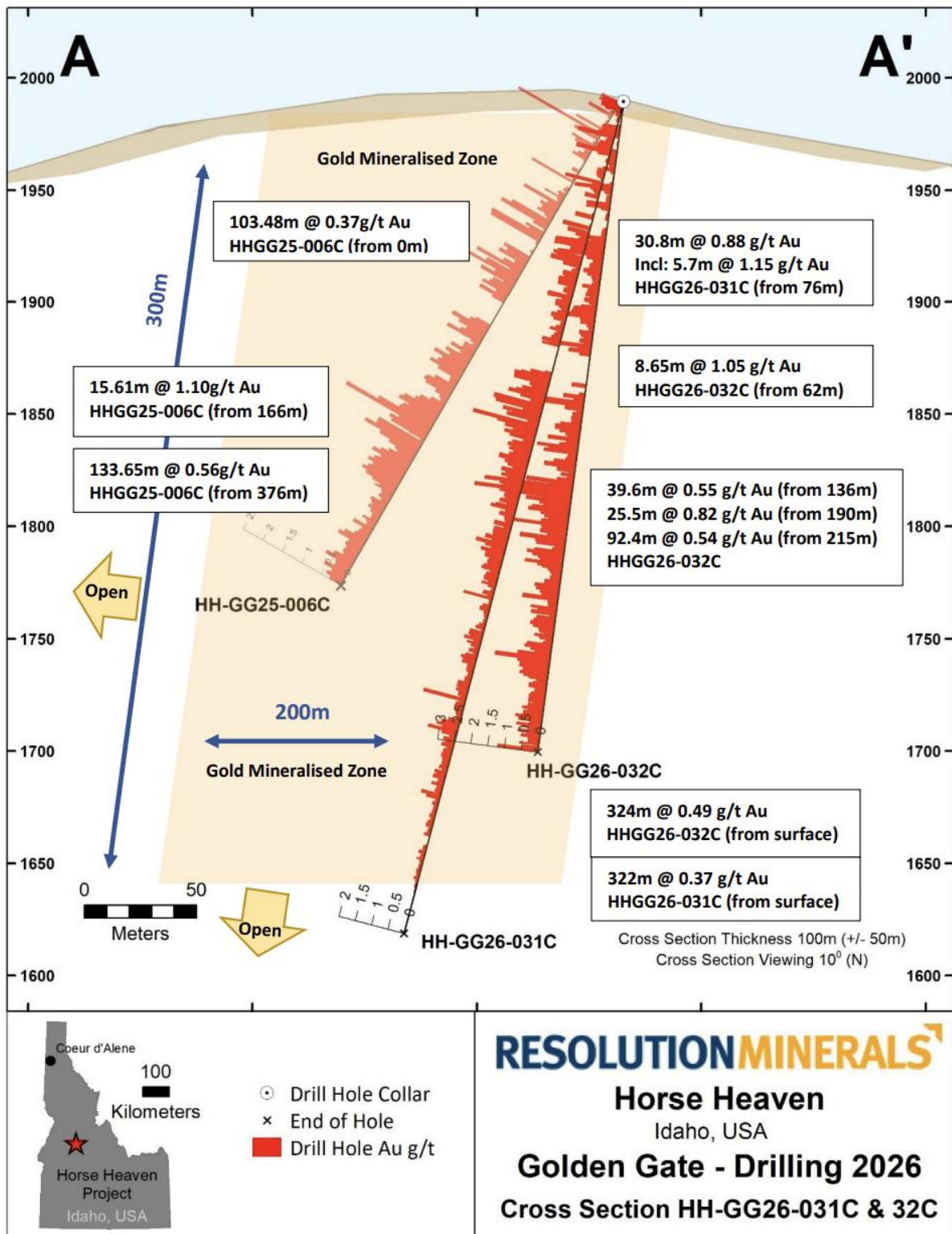
Figure 4: Resolution's Golden Gate North – Cross section of two reported drill holes with gold assays as histograms in red, overlain on 2025 drillhole HHGG25-006, with significant gold intervals and interpreted gold mineralised zone.
