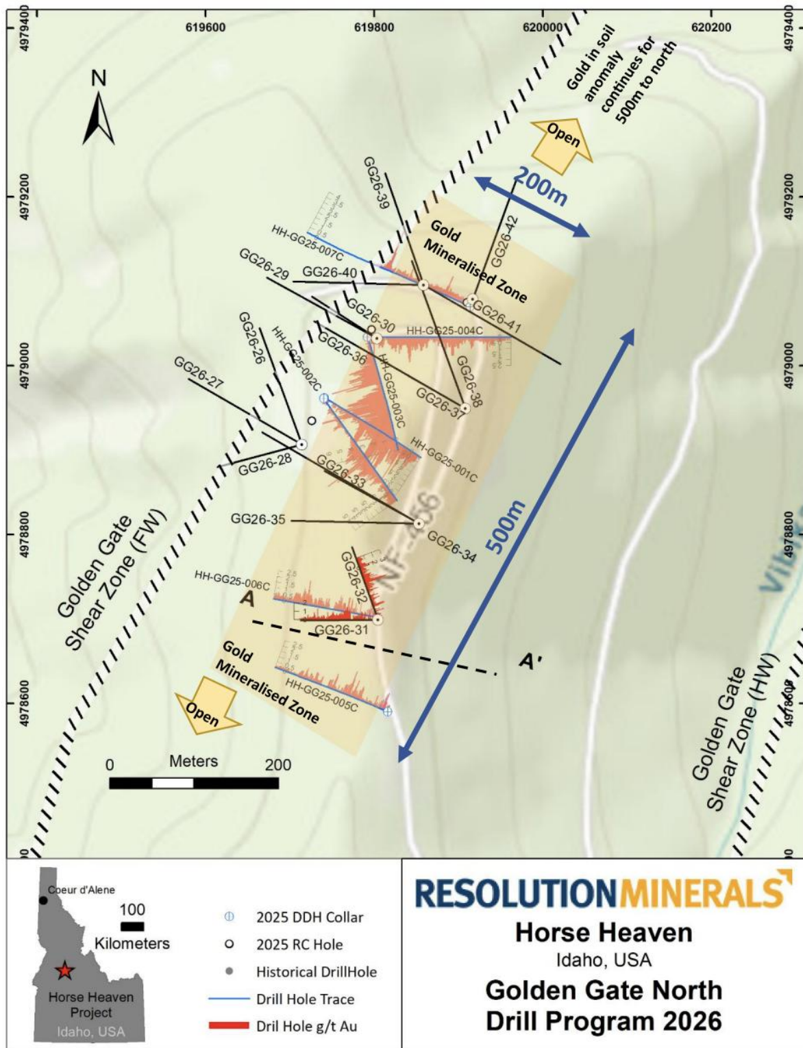
Figure 3: Resolution's Golden Gate North – Location of drill holes 2026 and 2025 with reported drill hole gold assays for drill holes in 2026 and 2025 as histograms (red) and location of Cross section in Figure 2, with interpreted gold mineralised zone (Pale yellow) and interpreted fault/shear zones. Note the zone is open ended to NE and SW, with a gold-in-soil anomaly extending a further 500m to the north (see Figure 5).
