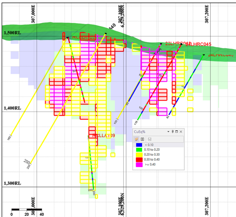
Figure 2: Drill AA48 200m+, Drill AA47 150m+ (oxide copper at surface). 2025 published resource block model shown in section. NB: Section width is 50m
