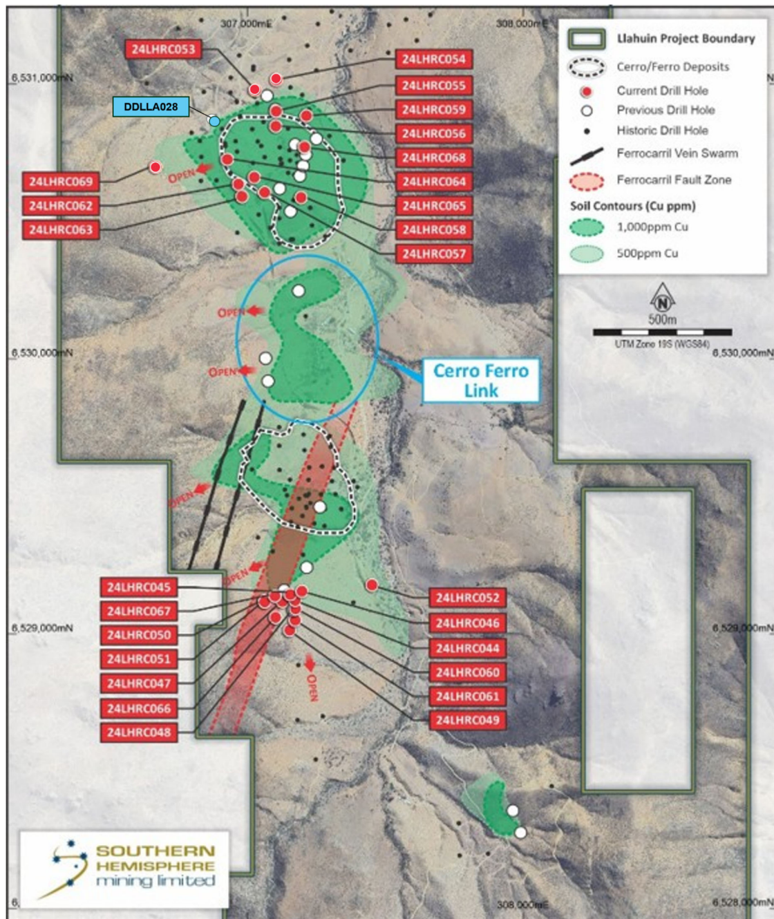
Figure 4: Plan view of the Cerro-Ferro and Ferro South zones showing current and previous drill holes
