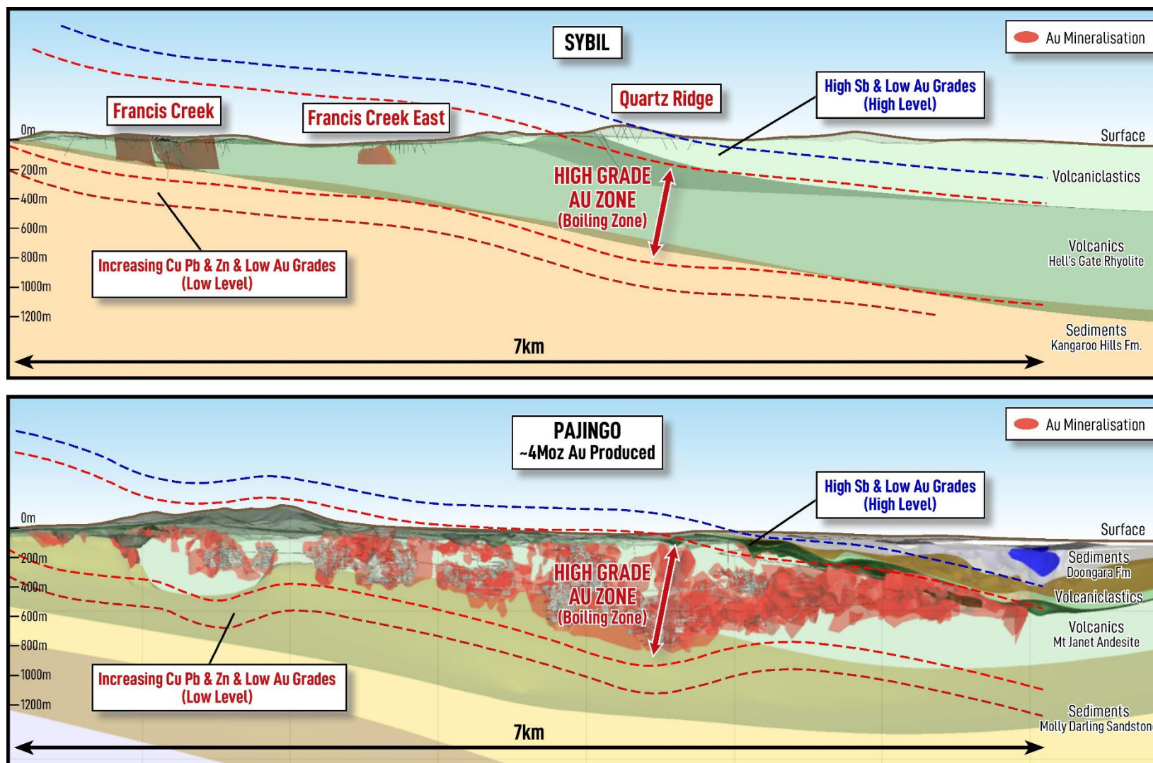
Figure 8: Schematic long section comparison of the Sybil and Pajingo epithermal systems (both long sections are looking north). Figure modified from AIG NEQ Minerals Workshop Presentation, "Pajingo – exploring undercover", March 2022.
