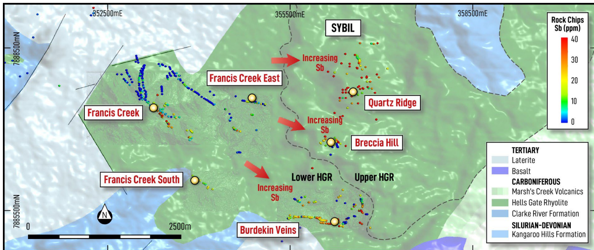
Figure 7: Antimony distribution (in rock chip sampling) increasing east and south-east of Francis Creek. Targets at Francis Creek East, Burdekin Veins, Breccia Hill and Quartz Ridge are interpreted to sit immediately above the prospective boiling zone window (Figure 5).
