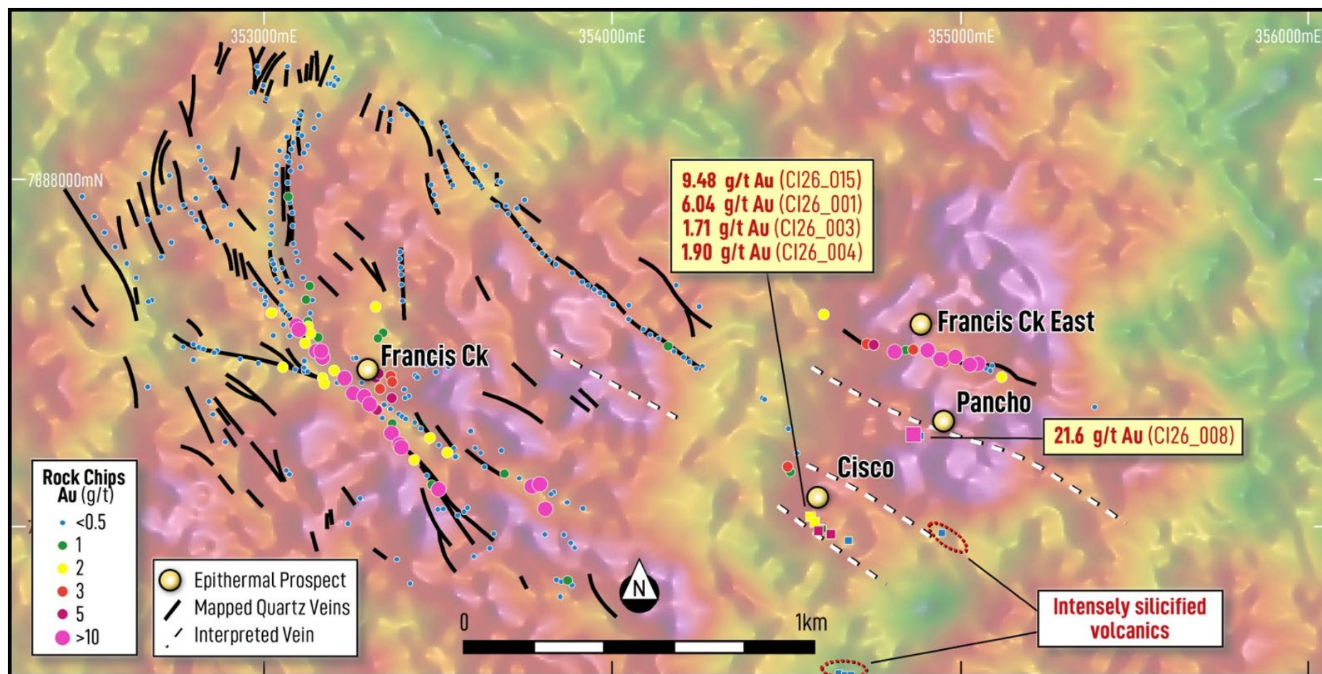
Figure 7: Radiometric image with zones of potassium depletion correlating to mapped quartz veins (black) in the Francis Creek to Francis Creek East area. Interpreted and now ground truthed, veins (white) including Cisco and Pancho veins show elevated Au in rock chip sampling.
