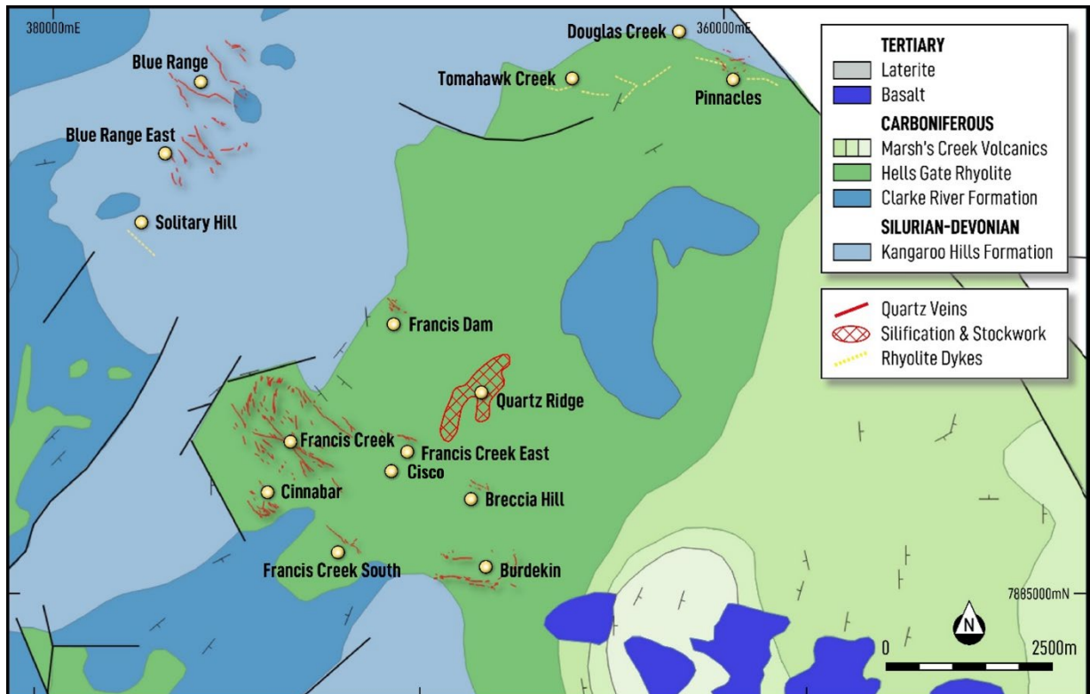
Figure 2: RC drilling tested the Francis Creek, Francis Creek East and Blue Range targets at Sybil. Next phase drilling, to commence in mid-October 2026, will also test the Burdekin Veins and Cisco targets.
