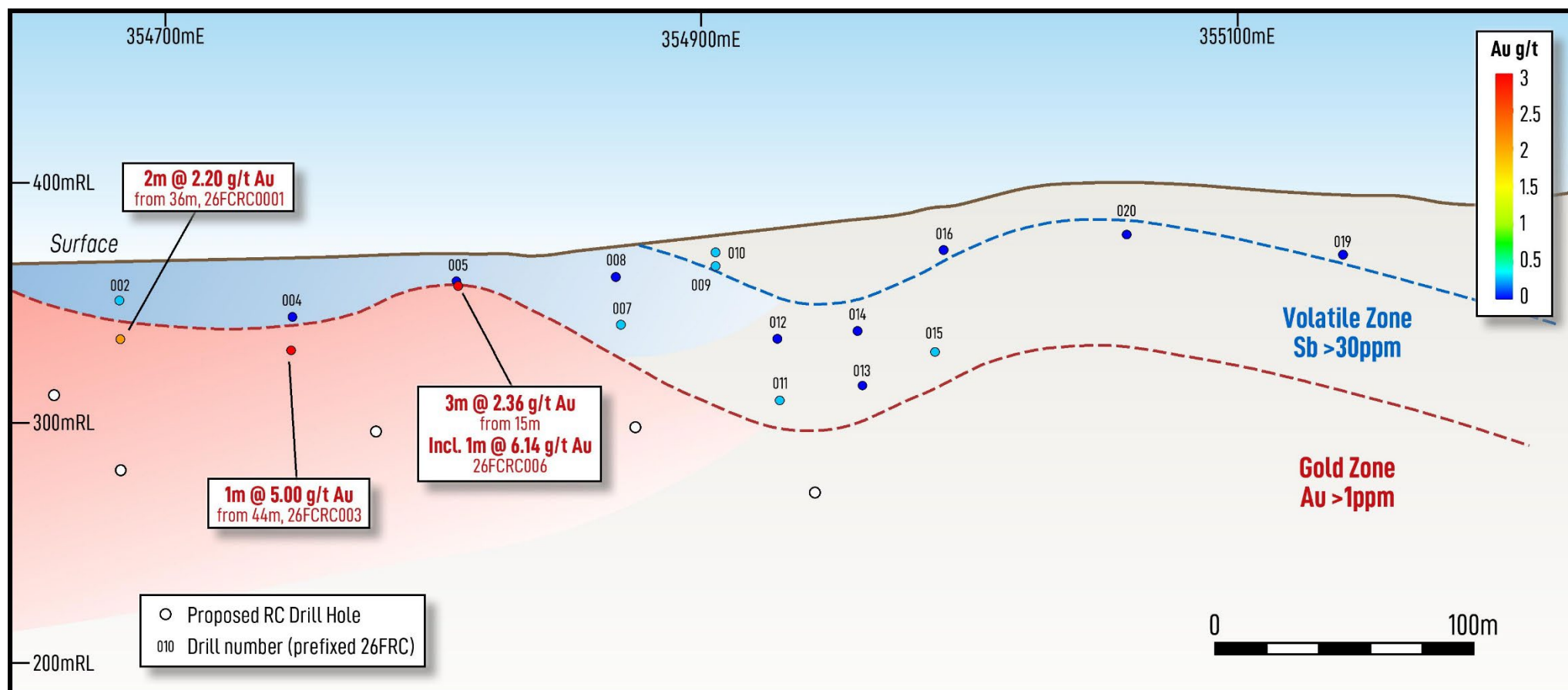
Figure 6: Long section of Francis Creek East drilling. Antimony is seen to be elevated in the east of the prospect, while all significant gold intercepts appear in the west of the prospect.
