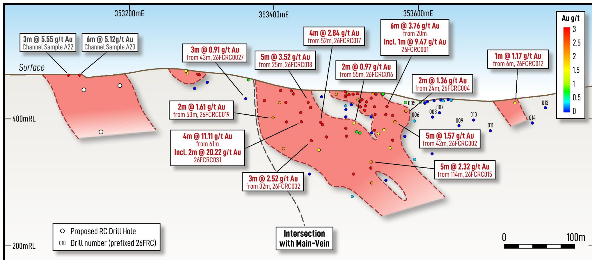
Figure 4. Long section across the Francis Creek A Vein drilling, showing the results from the A Vein east of the Main Vein and limited testing of the A Vein West area.
