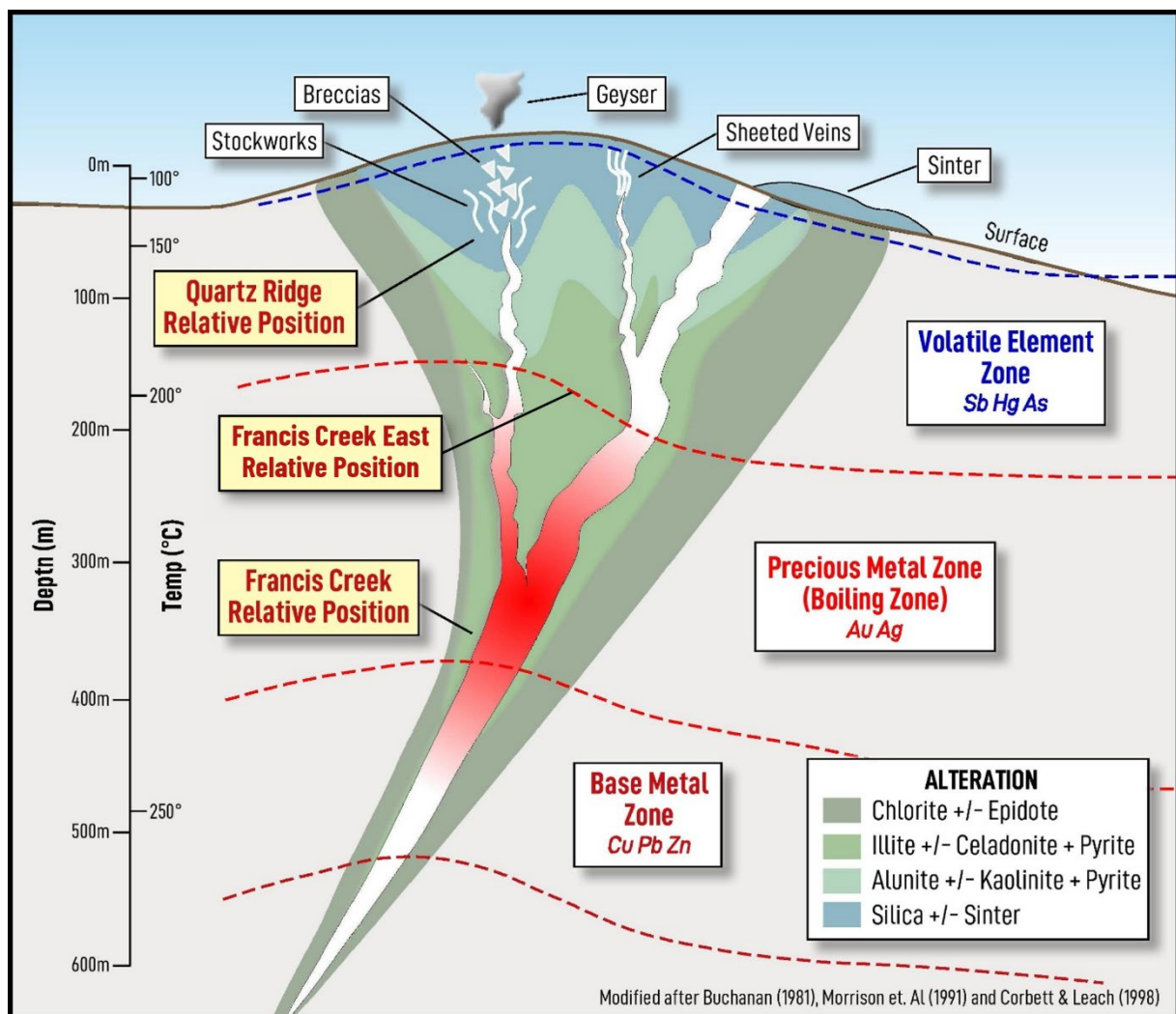
Figure 5: Geochemical zonation in low-sulphidation, epithermal deposits.
