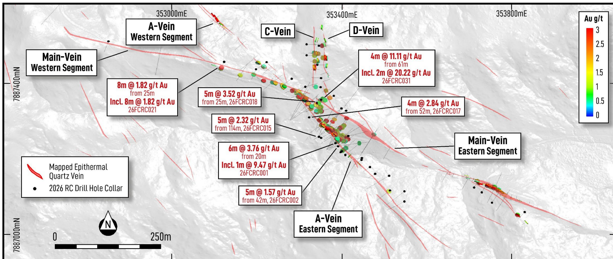
Figure 3: Plan view of Francis Creek showing drill collars and significant intersections from RC drilling completed.
