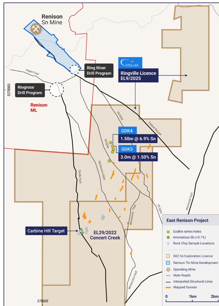
Figure 8: SRZ's Concert Creek EL, Ringville EL licence areas, historic drilling & SRZ rock chip sampling locations, major structures and location of Renison Tin Mine and Renison Mining Lease area (including Renison Tin Mine Development projection and recent drill program locations 12 )
