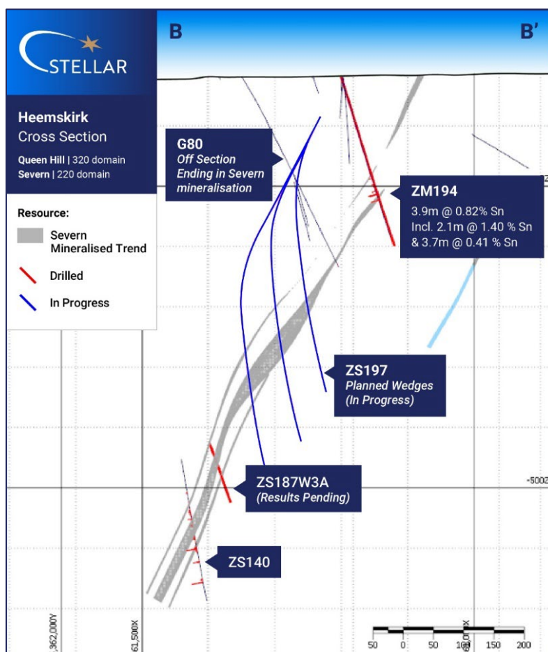
Figure 7: Drillhole Cross Section B-B' (Location on Figure 6), drillhole ZM194.
