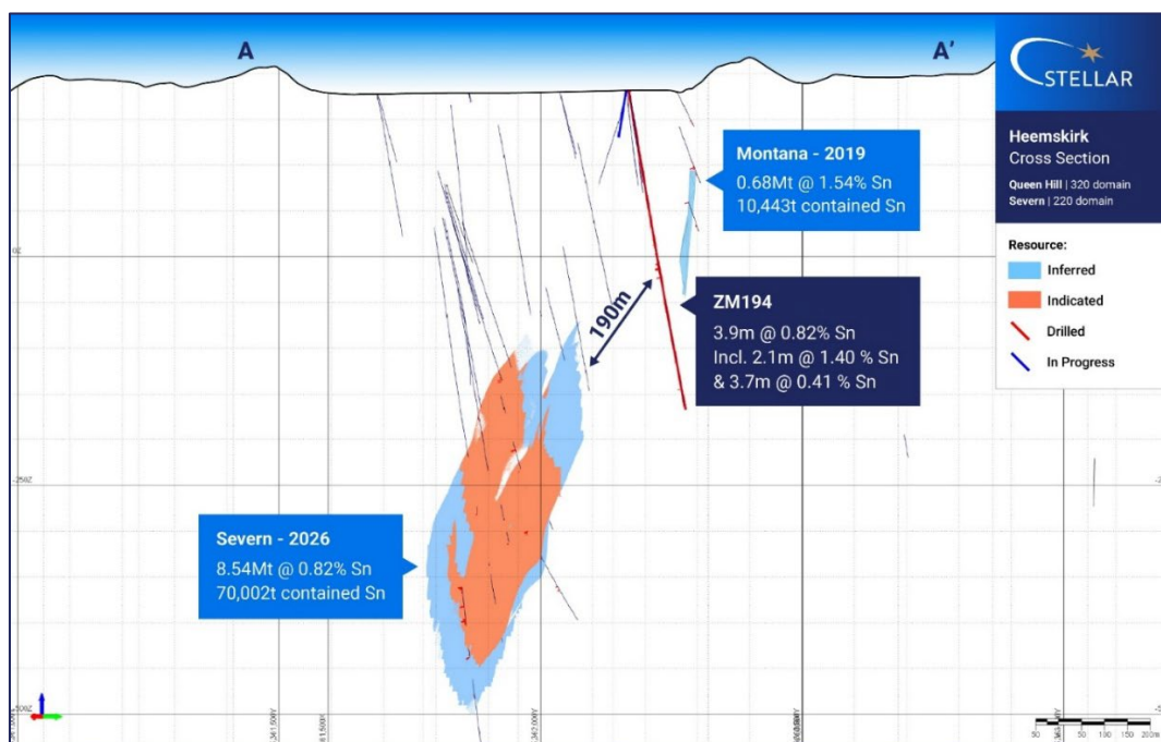
Figure 5: Drillhole Cross Section A-A' (Location on Figure 6), drillhole ZM194. Indicated and Inferred Resource blocks from the 2026 MRE 1 at Severn.
