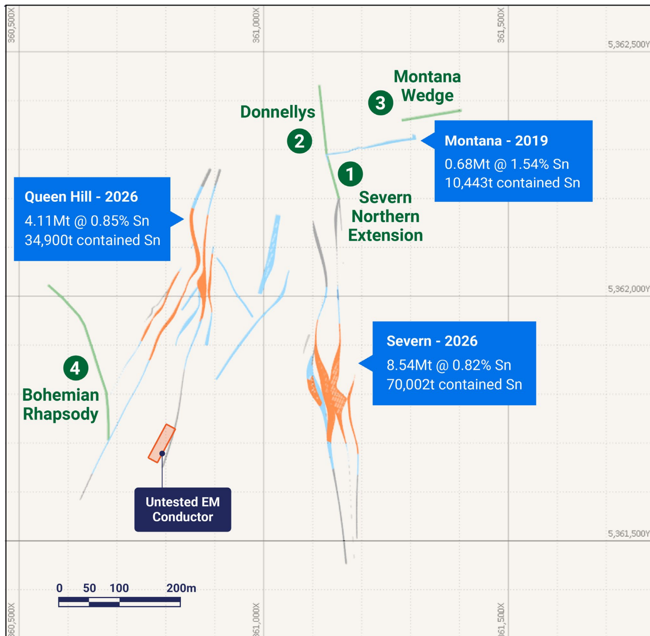
Figure 3: Heemskirk Tin Project, showing Queen Hill, Severn and Montana locations and targets (1-4) for drill testing outside of the Resource Models.
