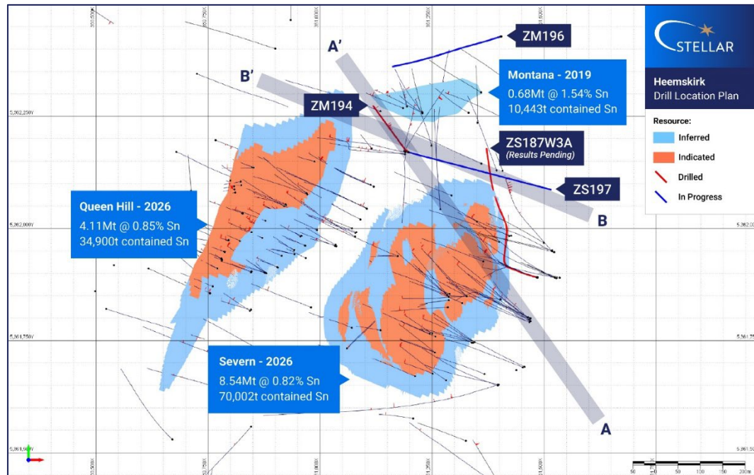
Figure 6: Drill hole location plan, location of cross sections A-A' (Figure 5) and B-B' (Figure 7). Grey boxes indicate section line and width of sectional view. Montana Inferred Resource block from 2019 MRE 2 and Queen Hill 8 and Severn 1 Indicated and Inferred Resource blocks from 2026 MRE 1 .
