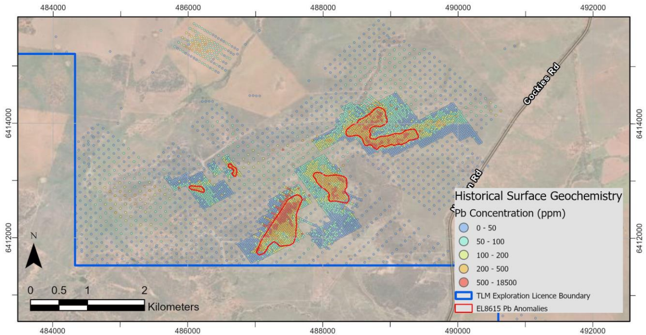
Figure d - EL8615 Lead geochemistry - Rip N Tear Prospect.
