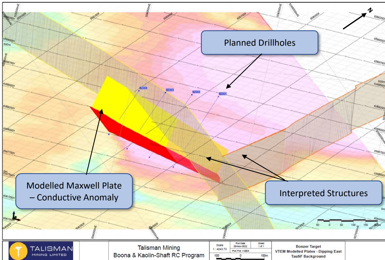
Figure b – Modelled Maxwell Plate, interpreted structures and planned drilling at the Bonzer Target, Kaolin Shaft Prospect Area.
