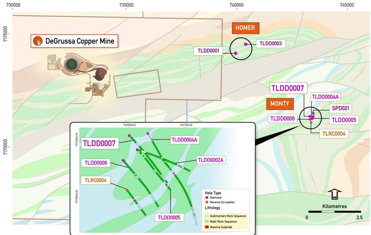
Figure 2 – Plan view showing location of recent exploration drilling relative to the DeGrussa Copper Mine.
