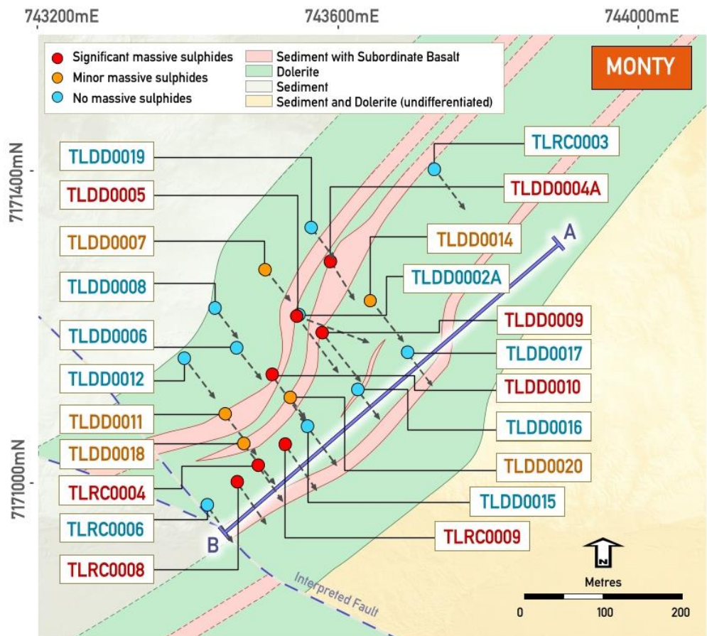
Figure 1 – Plan view of Monty showing drill-hole collar locations and interpreted schematic geology
