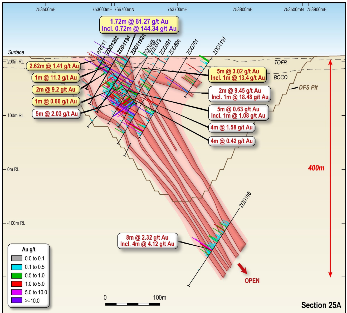
Figure 4: Oblique cross section showing latest drill results at AG Core (section 25A +/-12.5m)
