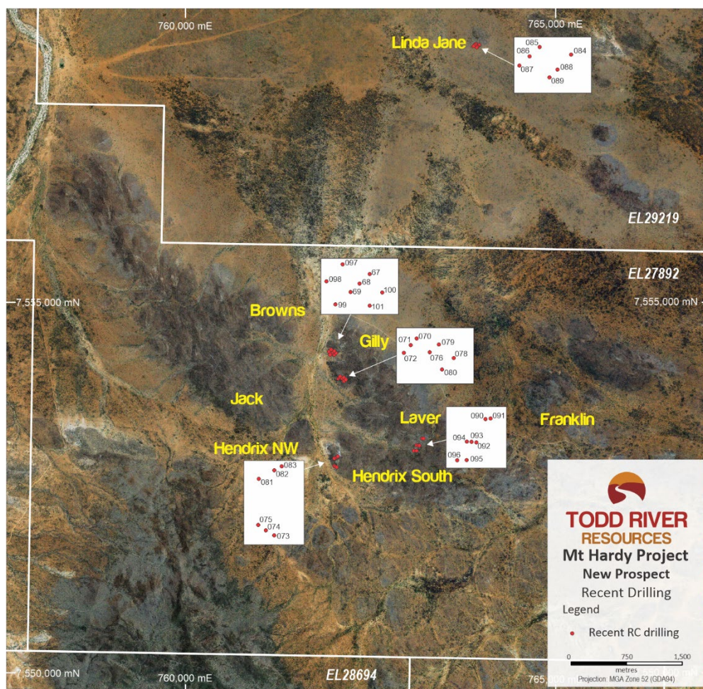
Figure 4. Mt Hardy Project showing the collar locations for the holes drilled during the recently completed reconnaissance RC drilling program.
