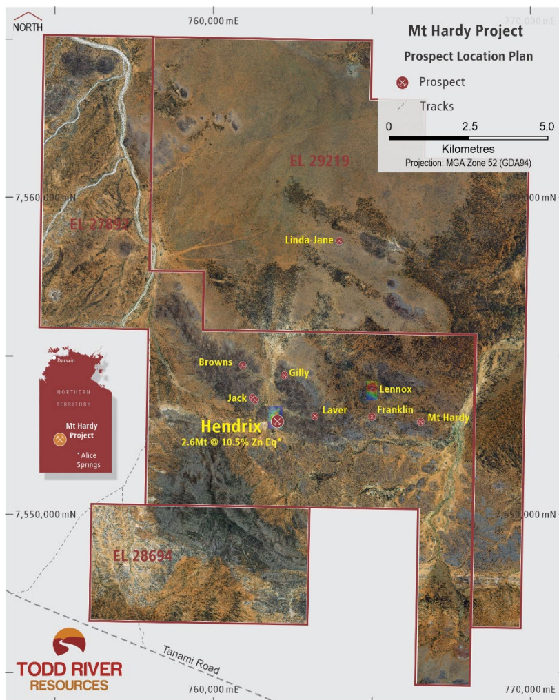
Figure 3. Mt Hardy Project showing new Prospect Locations
