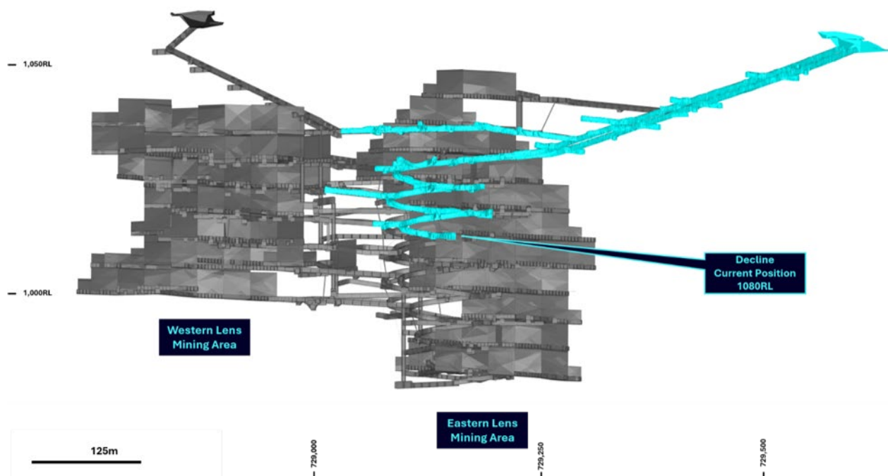
Figure 5: Yitirrti Mine as-built September-26 with LOM planned development (current development in blue).
