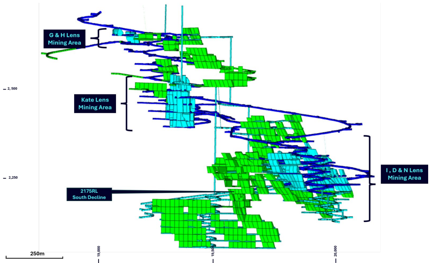
Figure 1: Woodlawn Mine as-built with current development and active mining areas (light blue) and planned LOM stopes (green).
