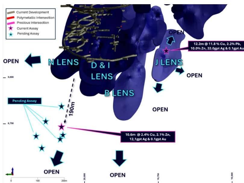
Figure 3: Woodlawn Project DM15 significant intersections N & J Lens (oblique long-section +/-1000m).
