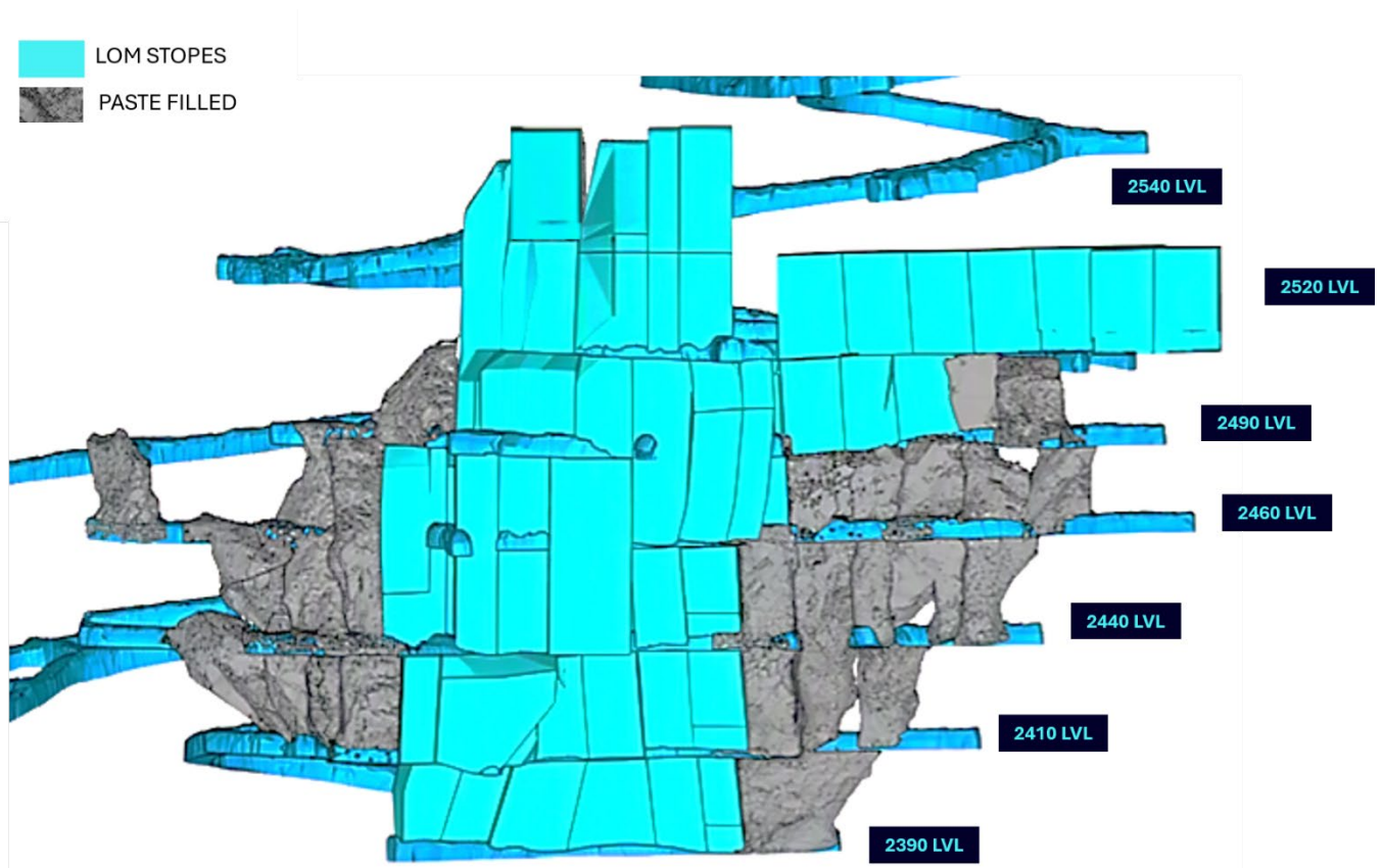
Figure 2: Kate Lens stope status. High-grade central corridor scheduled for the coming quarters.
