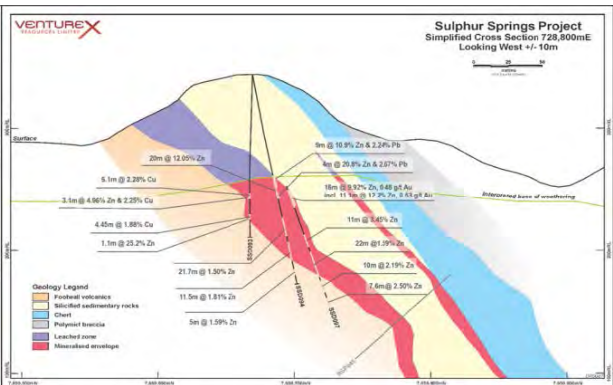
Figure 6: Sulphur Springs cross section on 728,800mE
