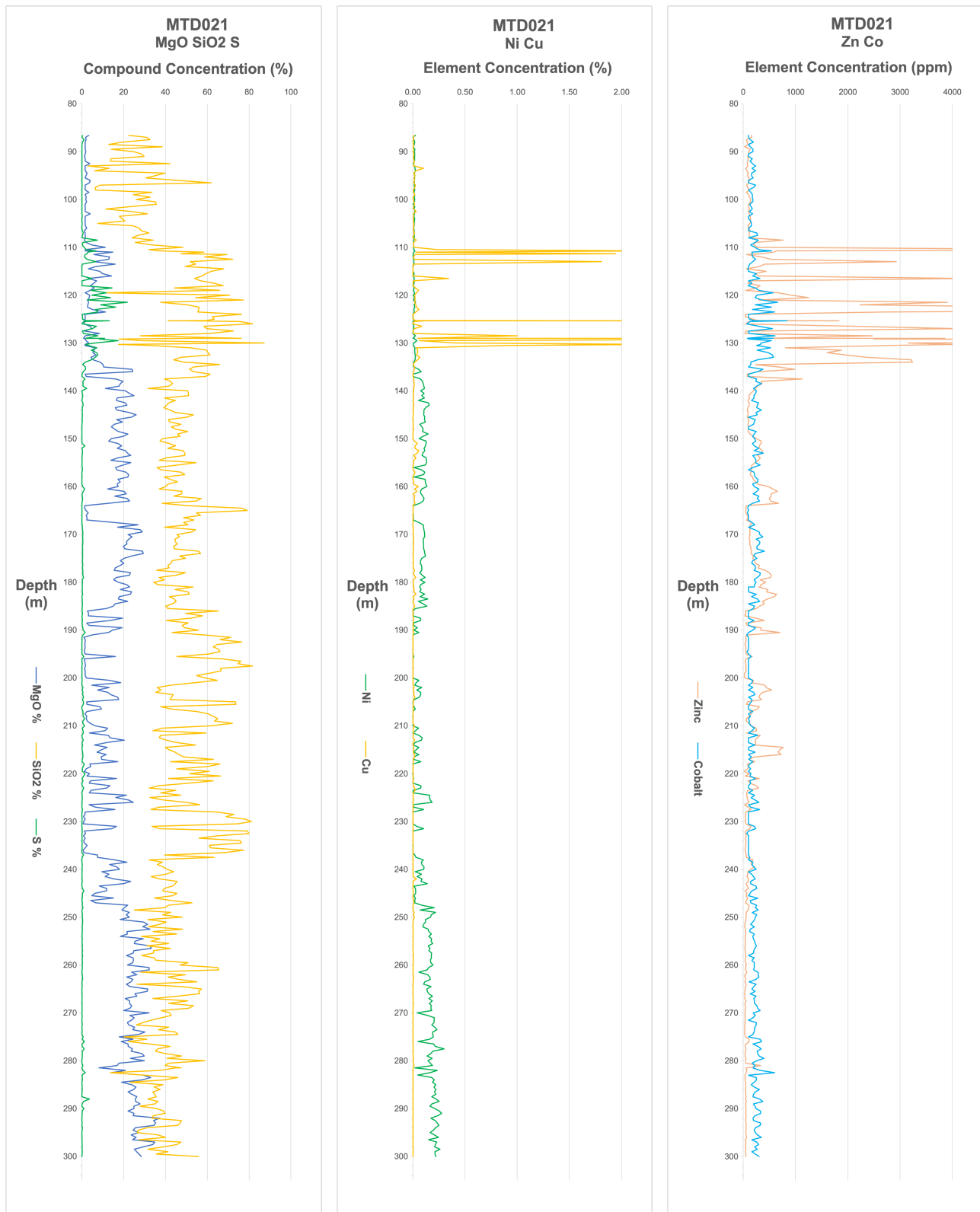
Figure 3: Processed pXRF data for hole MTD021
