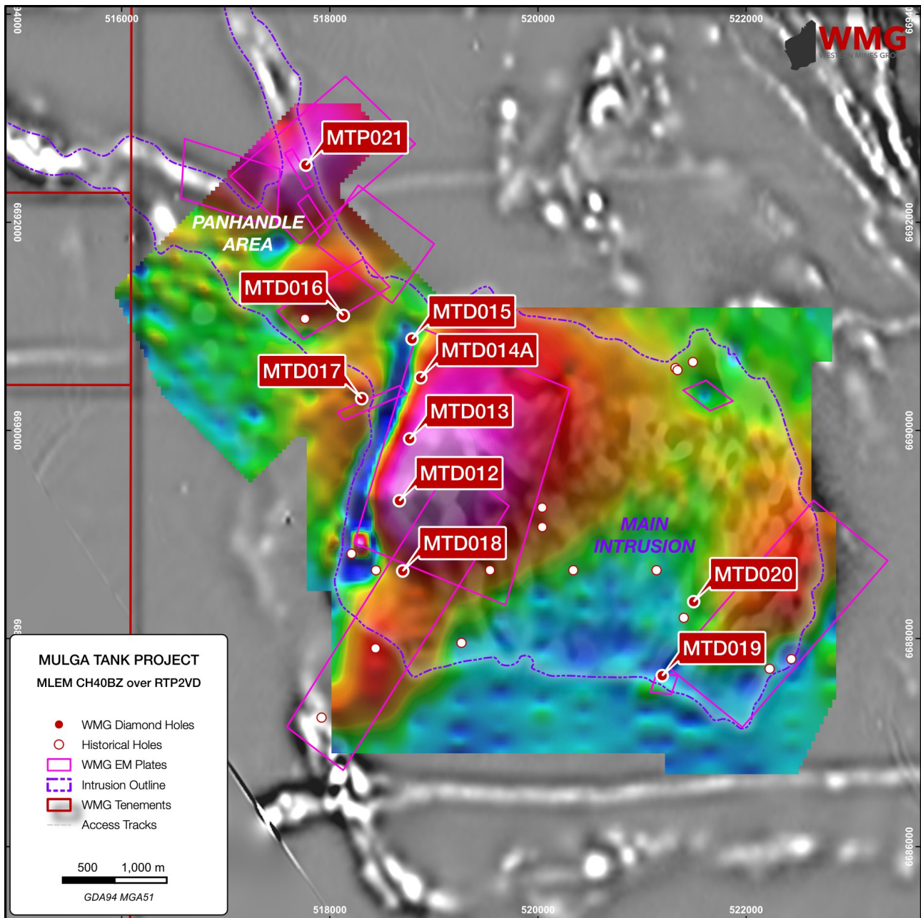
Figure 4: Mulga Tank MLEM late channel CH40BZ image showing EM plates and WMG's completed drill holes
