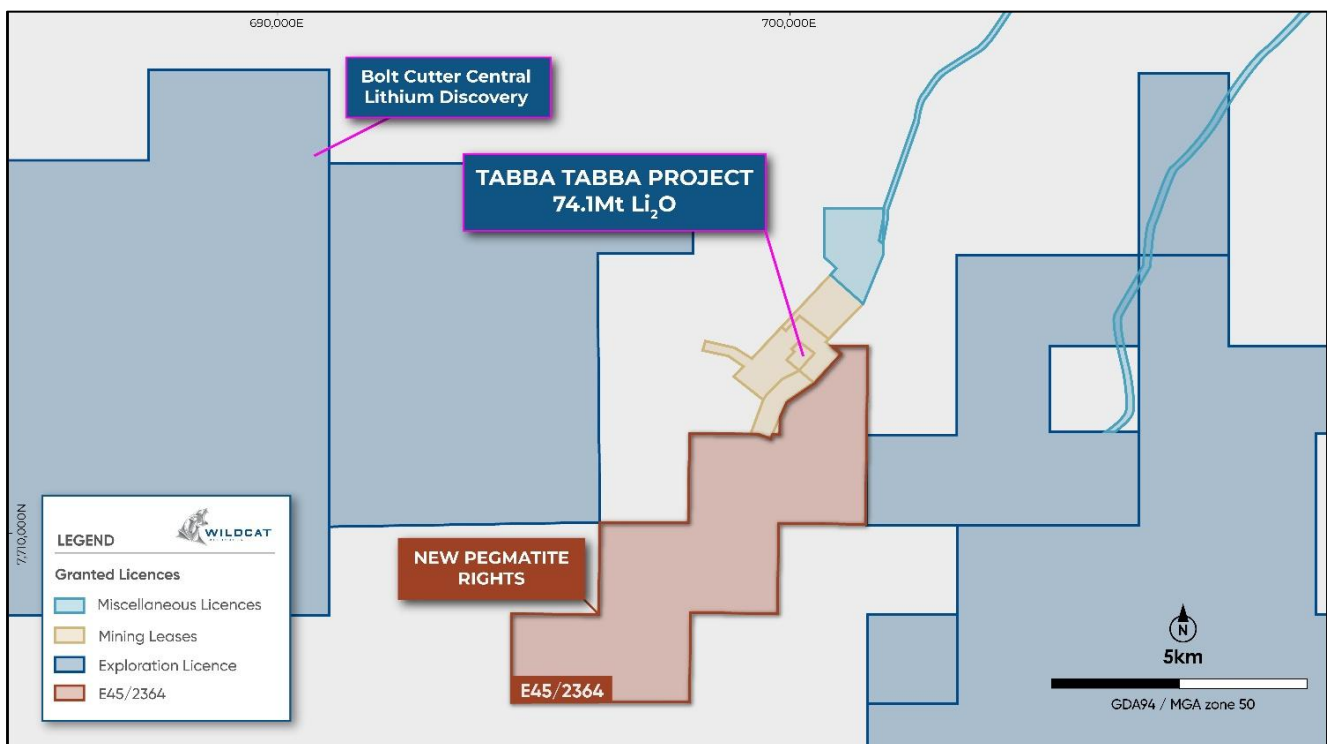
Figure 1: Tabba Tabba Project tenements and the location of E45/2364 (only relevant WC8 project tenements shown)
