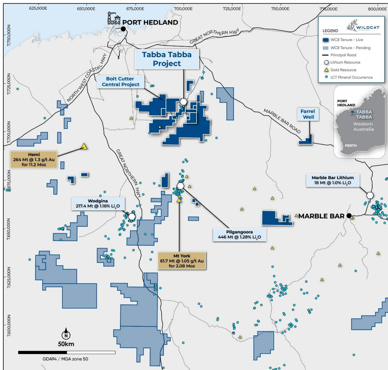
Figure 3: Location of Tabbatabba and the surrounding exploration tenements at quarter end. Pending Miscellaneous Leases or second-in-time applications are not displayed. Exploration rights may vary, with full details of tenure status and changes found in Appendix 1.
