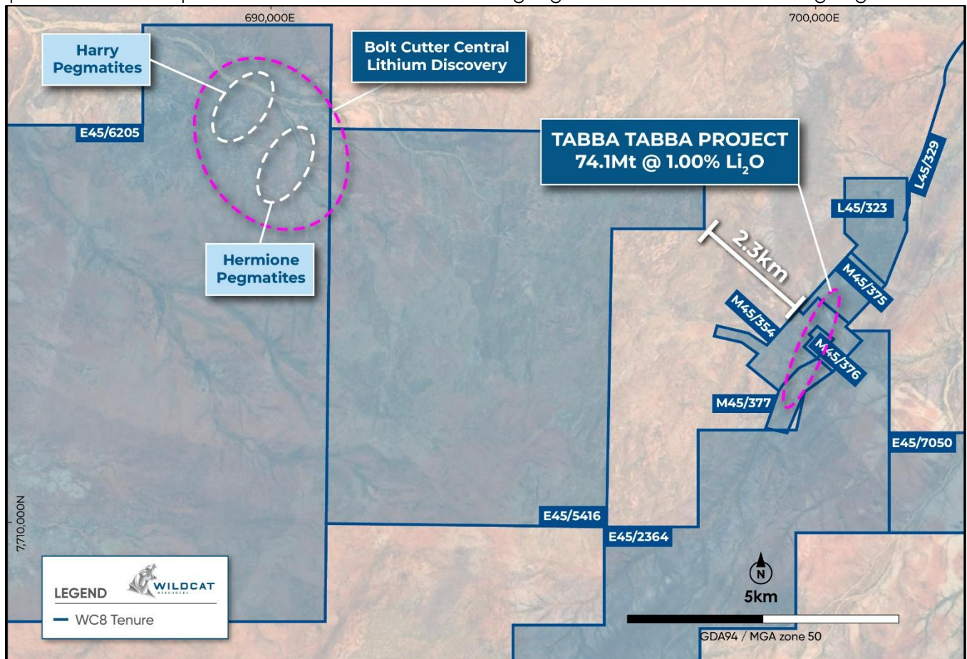
Figure 4: Location of the Bolt Cutter Central discovery relative to the Tabbatabba Project, WA. Mineral and exploration rights may across vary across tenements.
