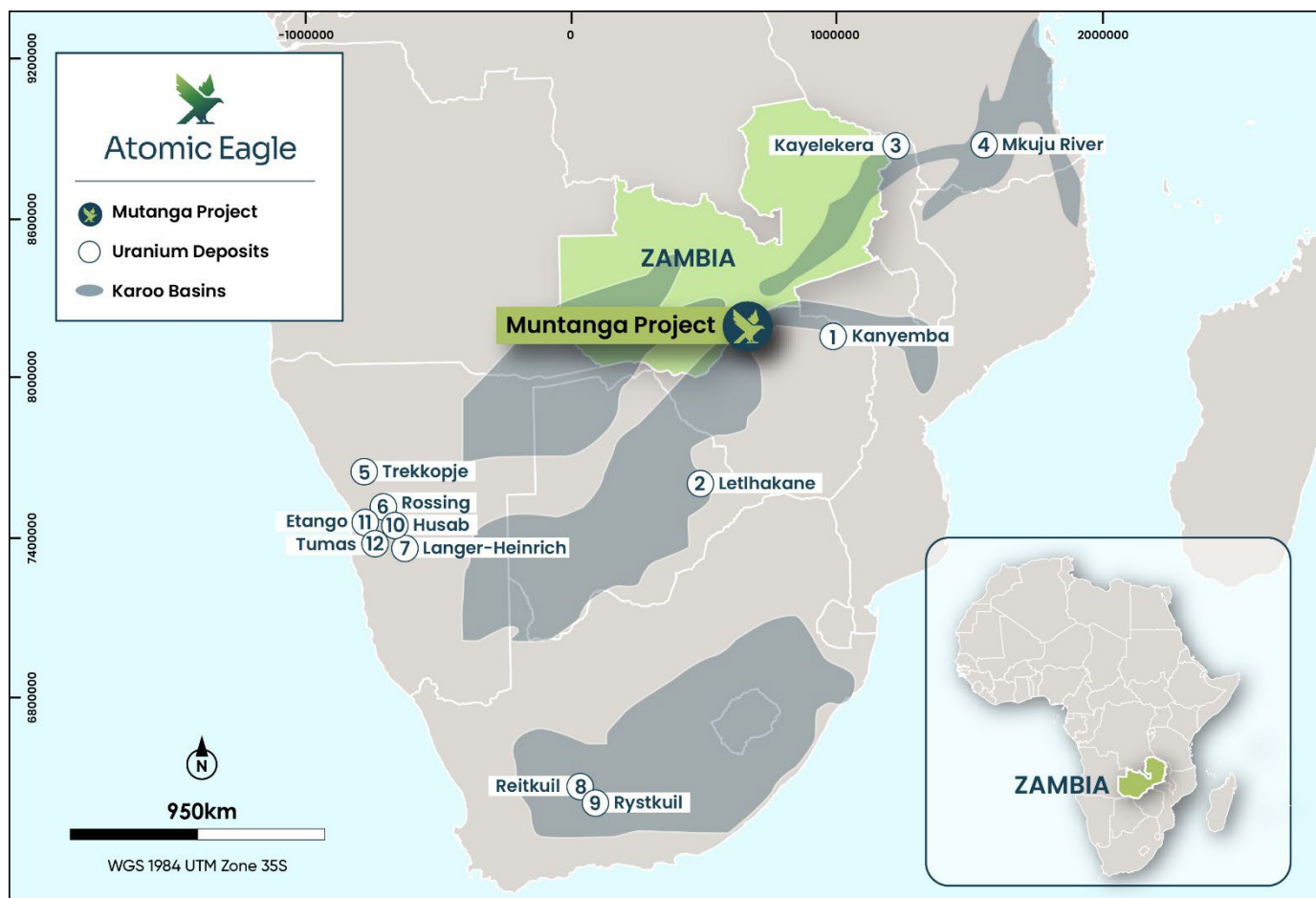
Figure 3: Major African uranium deposits and location of the Karoo Basins of southern Africa
