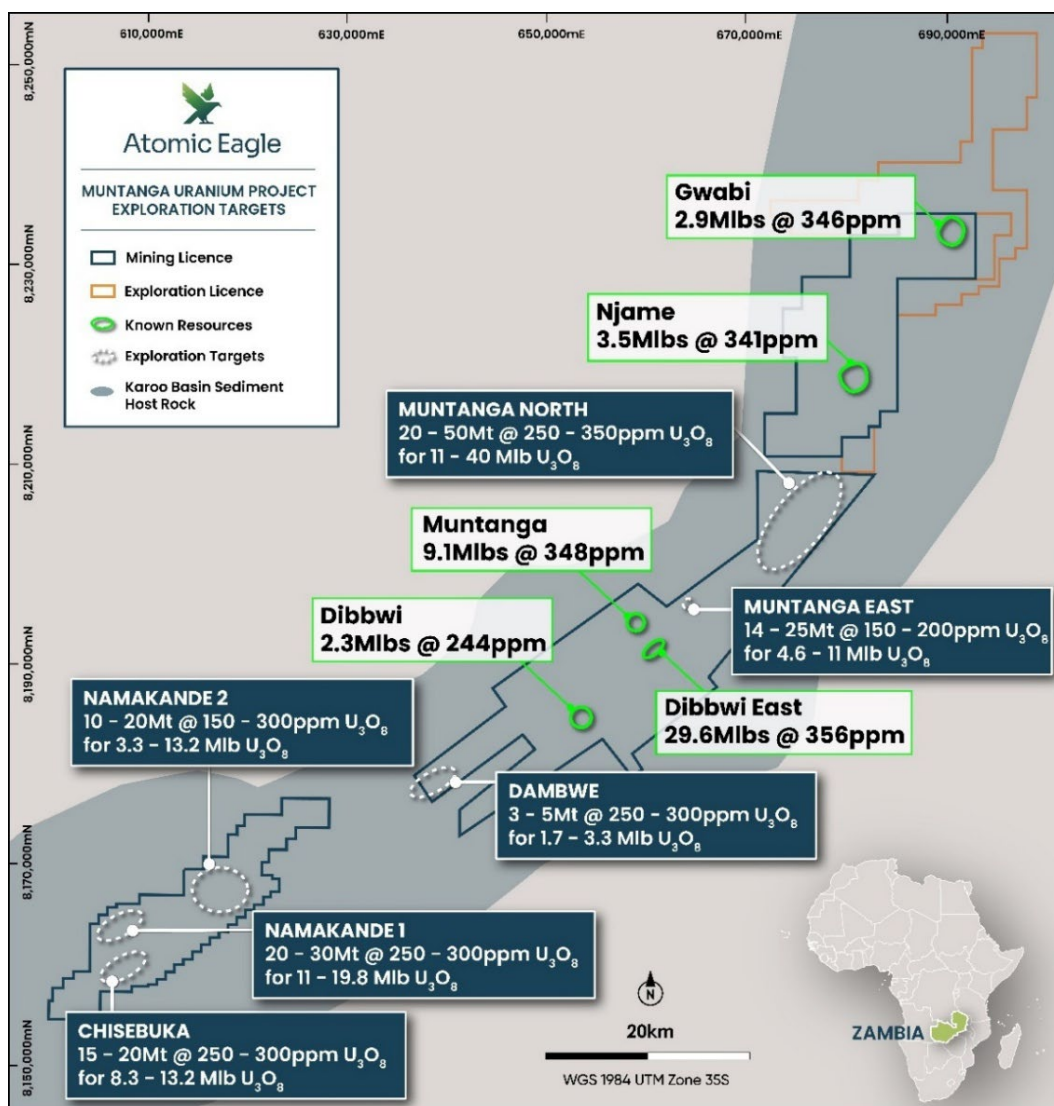
Figure 2: Location of Exploration Target areas
