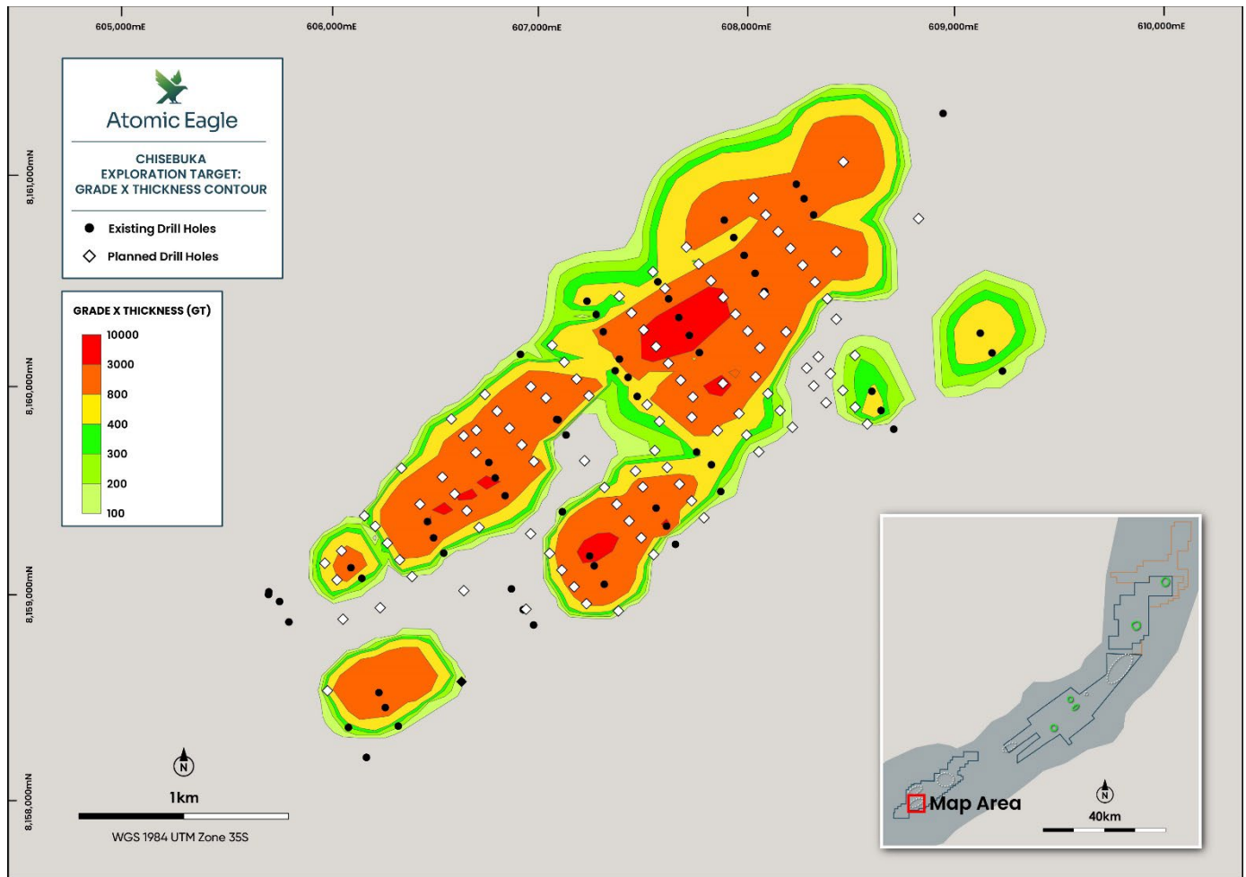
Figure 10: Chisebuka Exploration Target: ‘Grade x Thickness’ contours from historical drilling and proposed drilling
