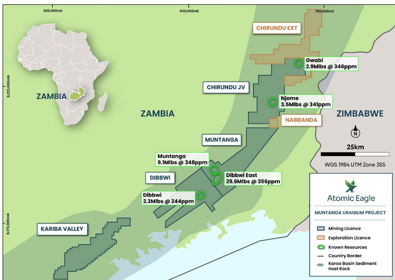
Figure 1: Location of Mineral Resources within the broader Muntanga Project licence area
