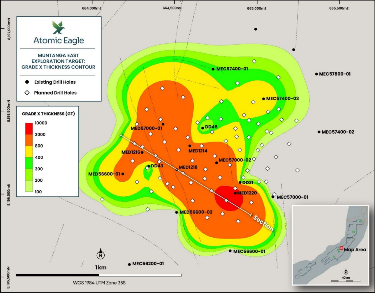
Figure 6: Muntanga East Exploration Target: Historical and planned drilling over ‘Grade x Thickness’ contours
