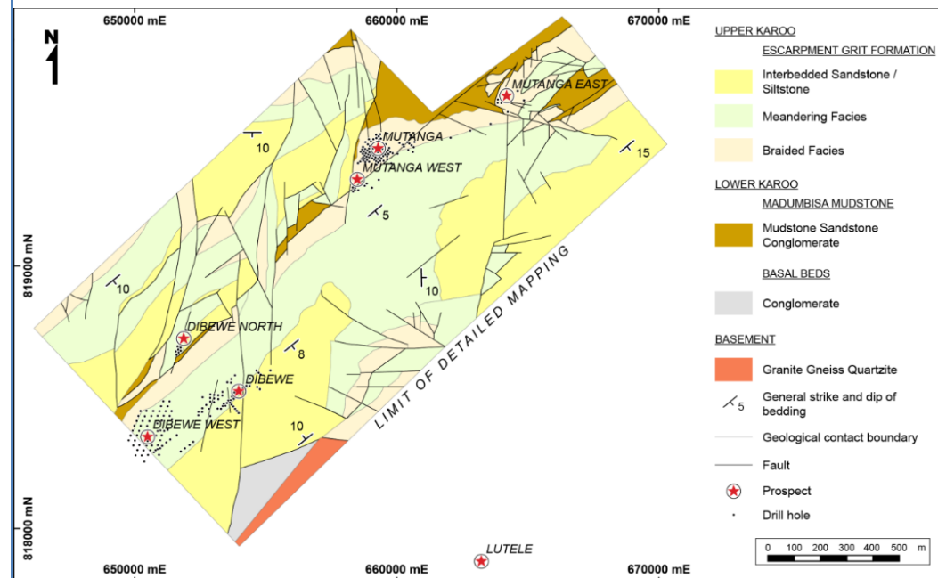
Regional Geology Map
