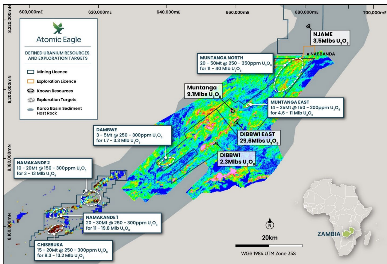
Figure 4: Muntanga Uranium Project: Map showing defined Uranium Resources and Exploration Targets overlaid on radiometrics
