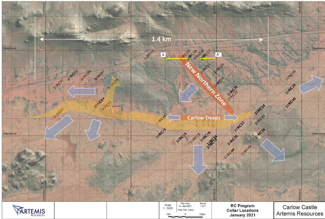
Figure 1: Carlow Castle current drilling programme map showing current reverse circulation (RC) hole locations, with previous drilling and 2019 inferred Mineral Resource Estimate (MRE) schematic outline (as released to the ASX on 20 November 2019 1 ), with the location of interpretive drill cross section (A – A') 7,698,980mN +/-10m shown as yellow line, and as cross sections in Figures 2 below. Blue arrows indicate interpreted directions of current and future drill plans.
