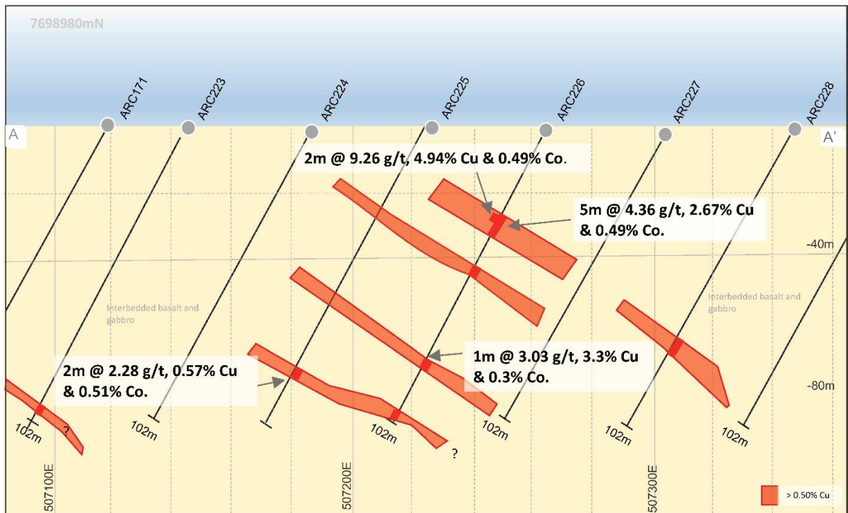
Figure 2: Carlow Castle current programme interpretive drill section 7,698,980mN +/-10m showing shallow RC hole intersections in the Northern Discovery zone.
