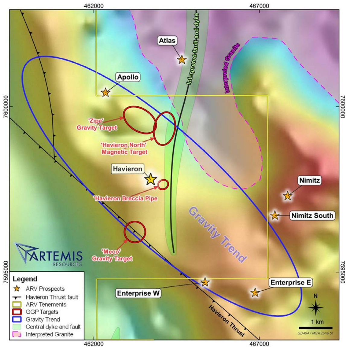
Figure 5: Central and Southern Artemis priority targets (yellow stars) over gravity Image and interpreted geology also highlighting NCM/GGP JV published regional targets (red).
