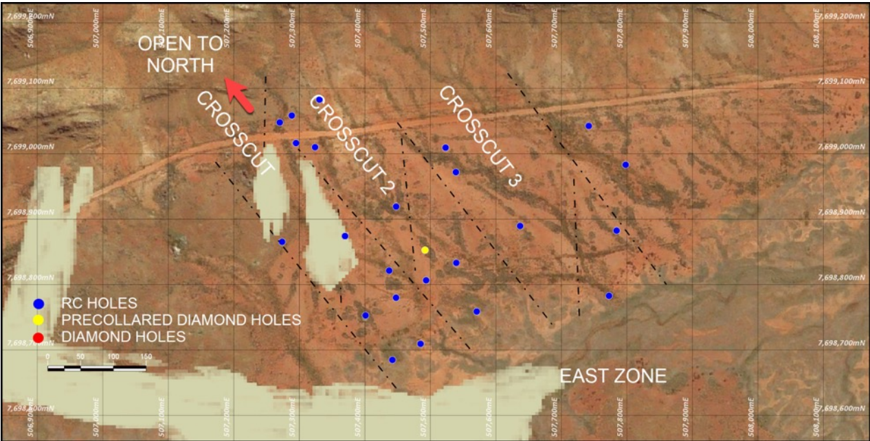
Figure 3: Details of the Crosscut Prospect illustrating the inferred bounding structures oriented to the northwest, forming 'corridors' labelled as Crosscut, Crosscut 2 and Crosscut 3.
