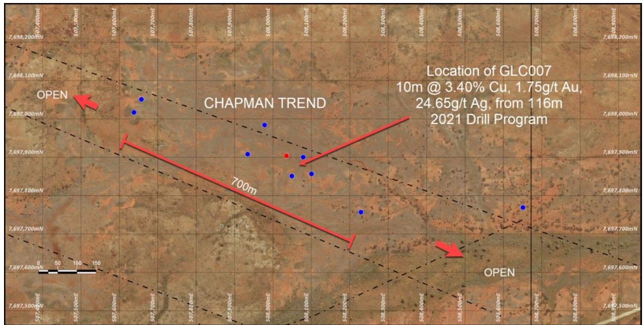
Figure 4: Chapman trend as defined by large west-northwest structures, has revealed significant sulphide mineralisation associated with coarse grained gabbro and basalts. Chapman is defined by magnetic trends and coincident VTEM signatures.
