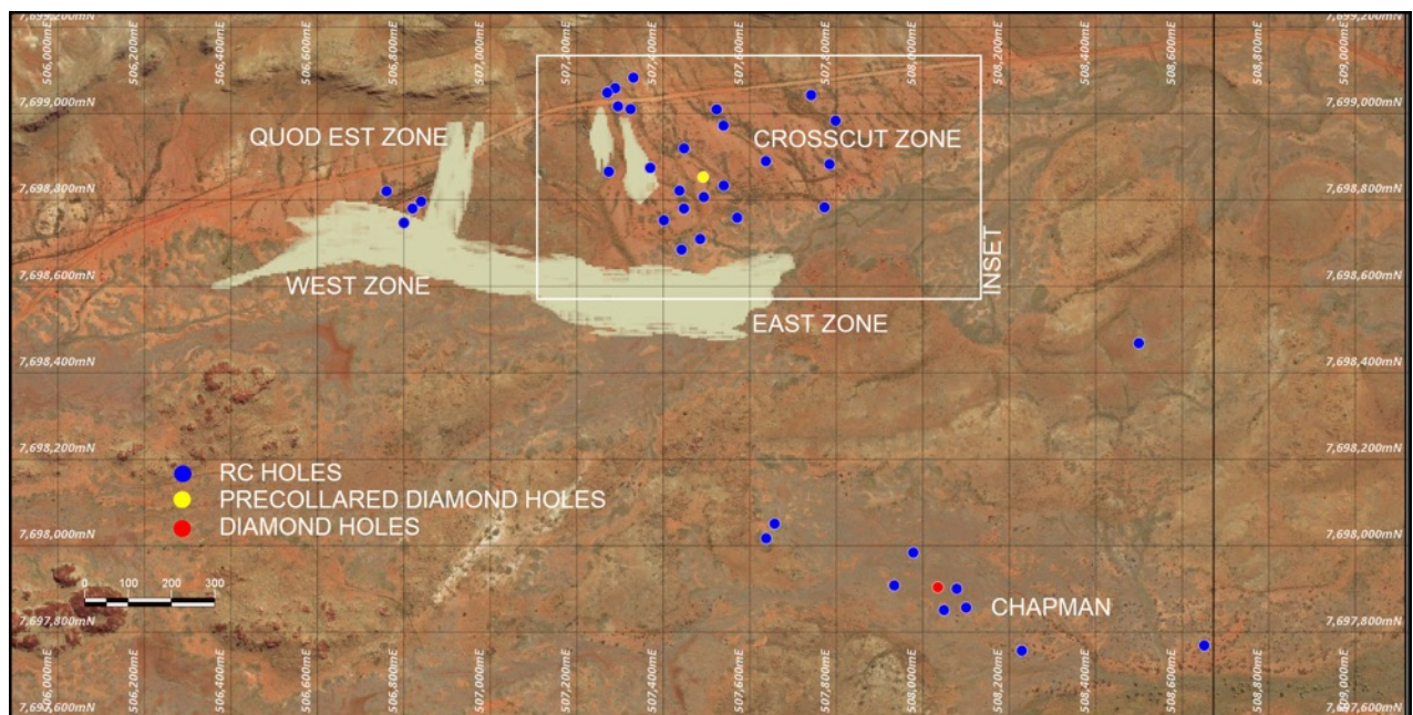
Figure 2: Location of Prospects at Carlow showing the current planned program drill collars. Carlow 2021 BM shown in pale yellow highlighting the potential of upscaling the mineralised envelope. Refer to Figure 3 for details of inset.
