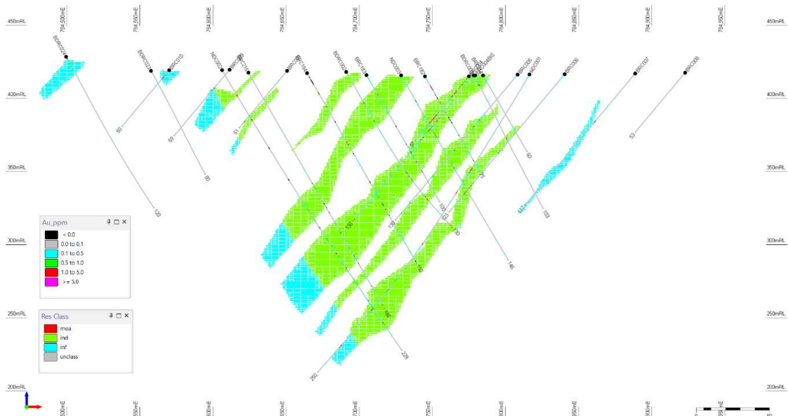
Figure 13: Example Cross Section BST Showing Resource Classification and Drill Data (Looking North +/-25m)
