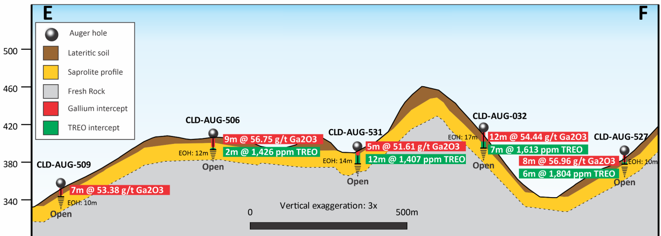
Figure 7. Cross section of auger drillholes on Area B Eastern portion.
