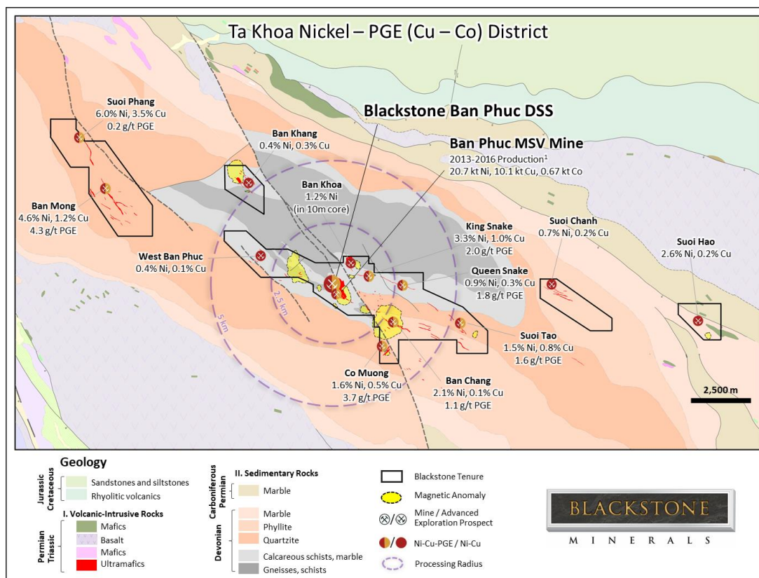
Figure 8: Ta Khoa dome geology prospective for multiple magmatic nickel sulfide deposits
