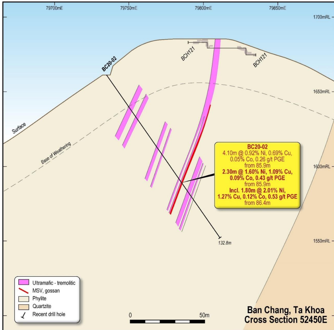
Figure 3: Ban Chang Cross Section 52450E showing maiden drill hole BC20-02 (refer to tables 1&2)
