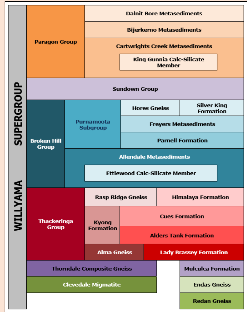
Figure C-3: Regional Stratigraphy
