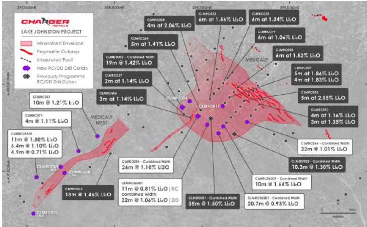
Figure 7. Medcalf Spodumene Deposit Plan showing new RC and diamond drilling results relative to the spodumene-bearing pegmatite swarm from surface and previous diamond and RC drill results at Medcalf MRE and Medcalf West Exploration Target.
