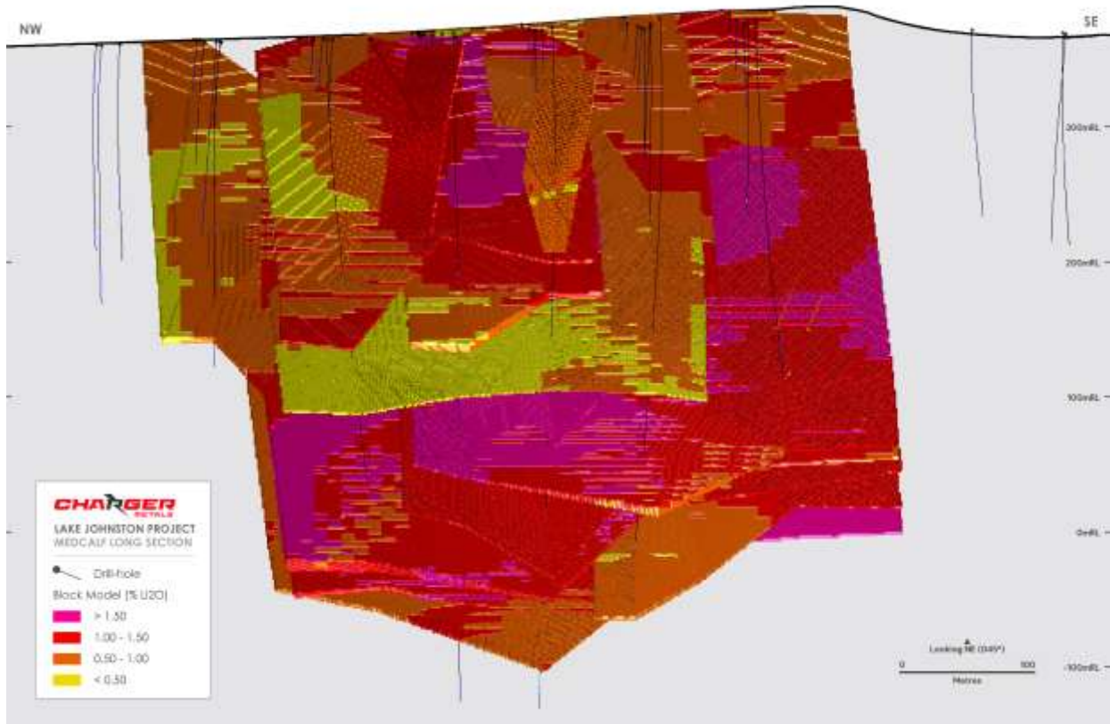
Figure 1. Long sectional view looking northeast of the Medcalf Lithium Mineral Resource.
