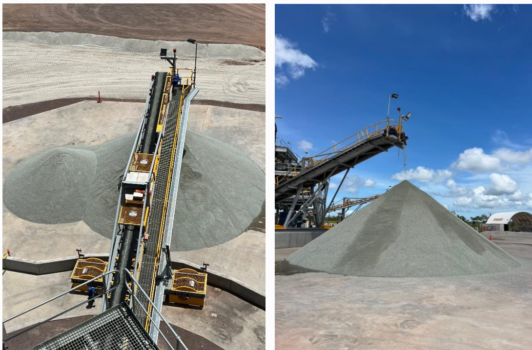
First Concentrate from the Finniss Lithium Mine
