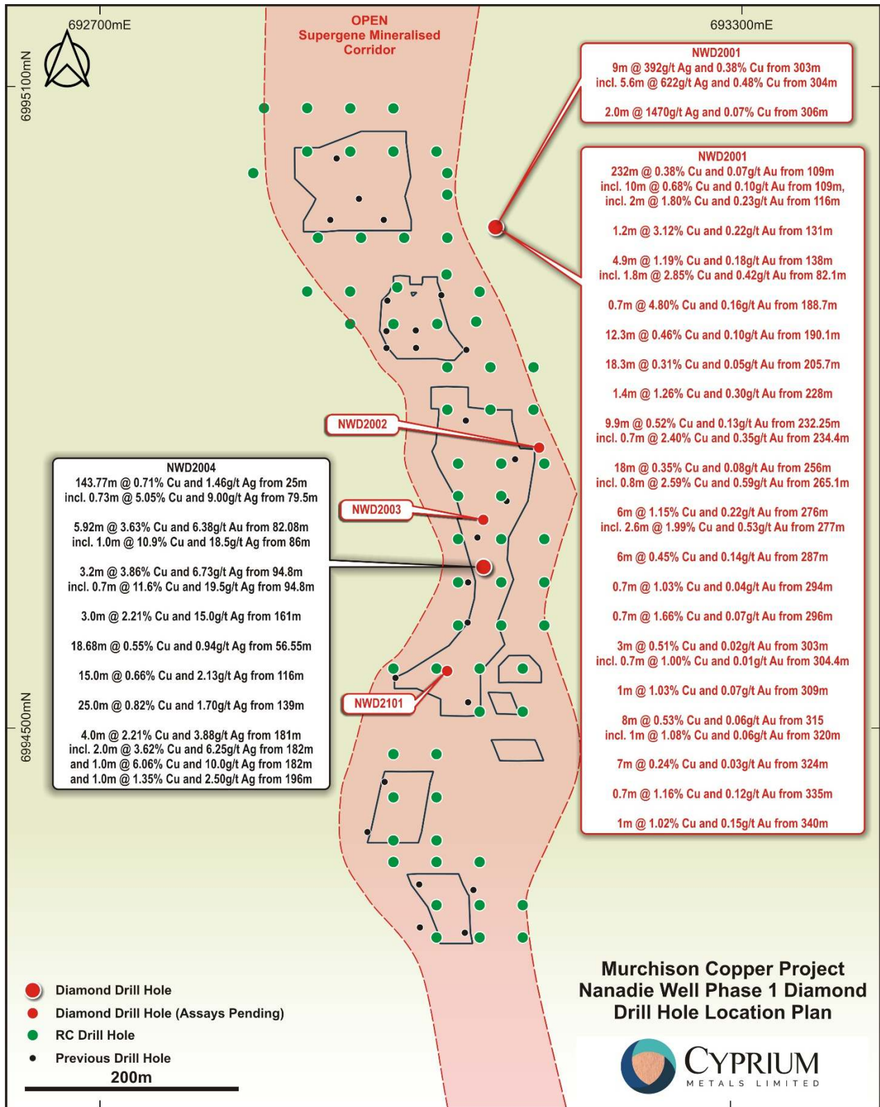
Figure 2 / Nanadie Well Phase 1 drill hole collar locations and diamond drill hole intercept highlights
