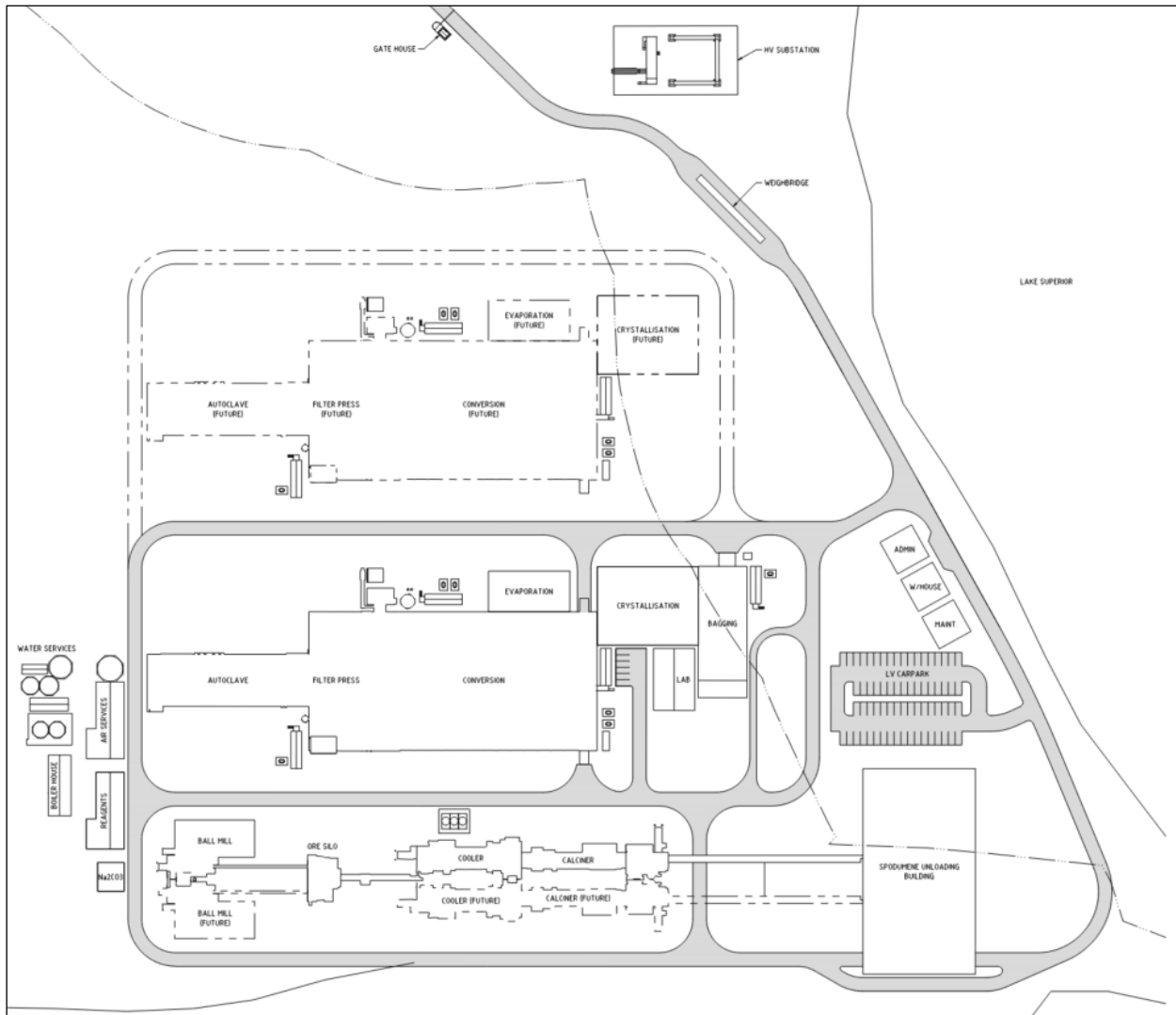
Figure 35: Lithium Hydroxide Conversion Plant Layout
