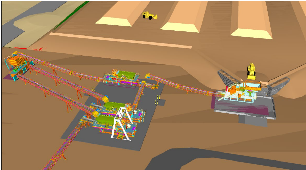
Figure 33: Seymour Crushing 3D Snapshot (Cladding Removed)
