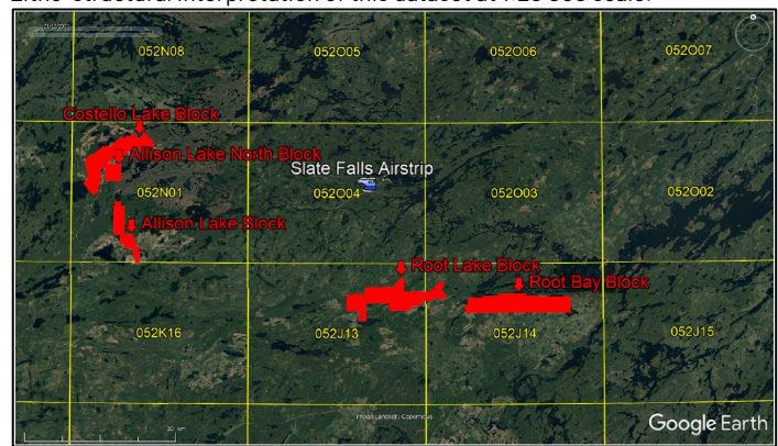
Figure 9 1 – Area covered by Aeromagnetic Surveys (Root, Root Bay and Allison)
