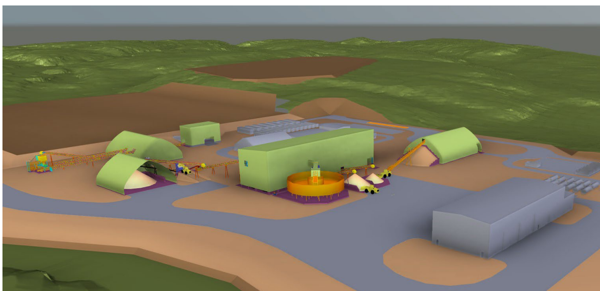
Figure 32: Seymour Concentrator & Mine Services Area
