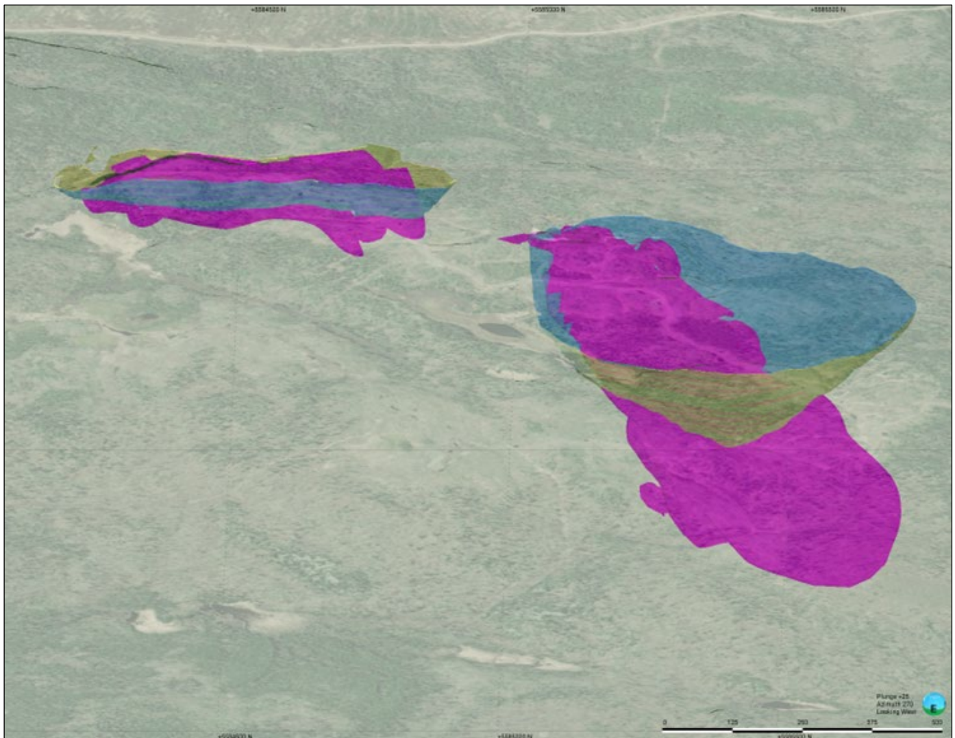
Figure 3: Aubry Interpreted Pegmatites with Overlaid Pit Designs
