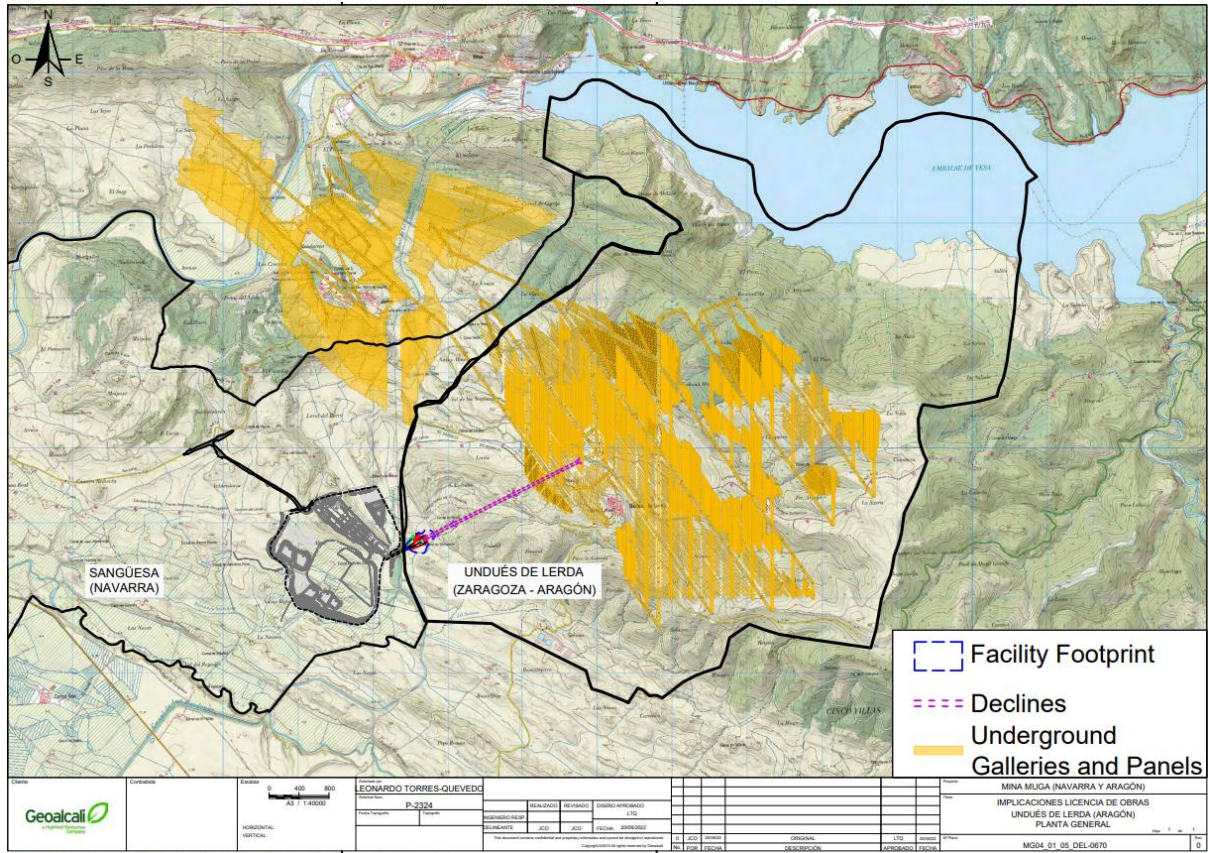
FIGURE 1: LOCATION OF THE MUGA PROJECT'S LICENCES IN UNDUE'S AND SANGÜESA
