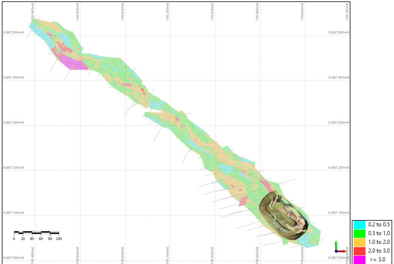
Figure 13: Shiraz drill hole plan showing mined open pit and OK resource block model coloured by Au (g/t)
