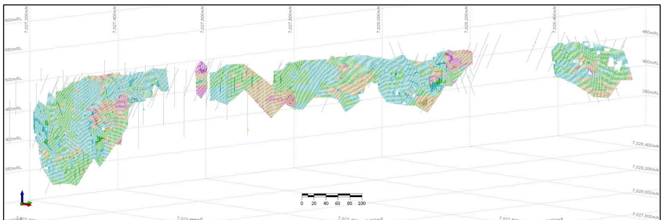
Figure 22: Specimen Well 3D looking down to the north-west showing drill holes and OK block model coloured by Au (g/t)
