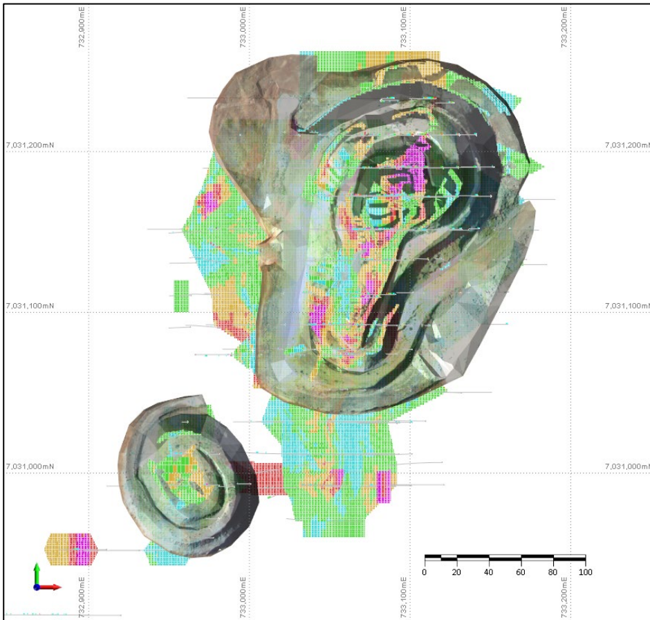
Figure 17: Toedter drill hole plan showing mined open pit and OK resource block model coloured by Au (g/t)
