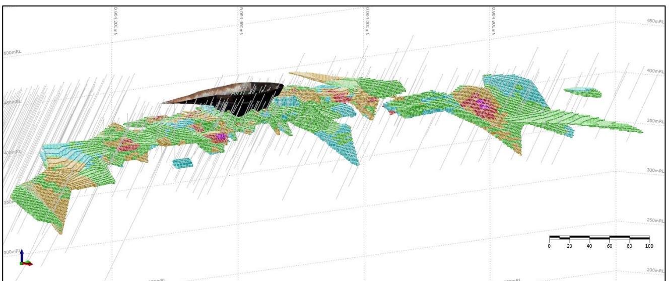
Figure 16: Think Big 3D view looking down to the north-west showing drill holes, mined open pits, and OK block model coloured by Au (g/t)
