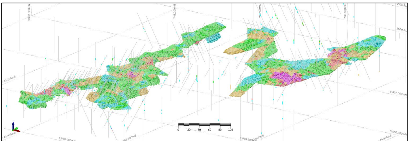
Figure 28: Hyperno-Reliance 3D view looking down to the north-west showing drill holes and OK block model coloured by Au (g/t)
