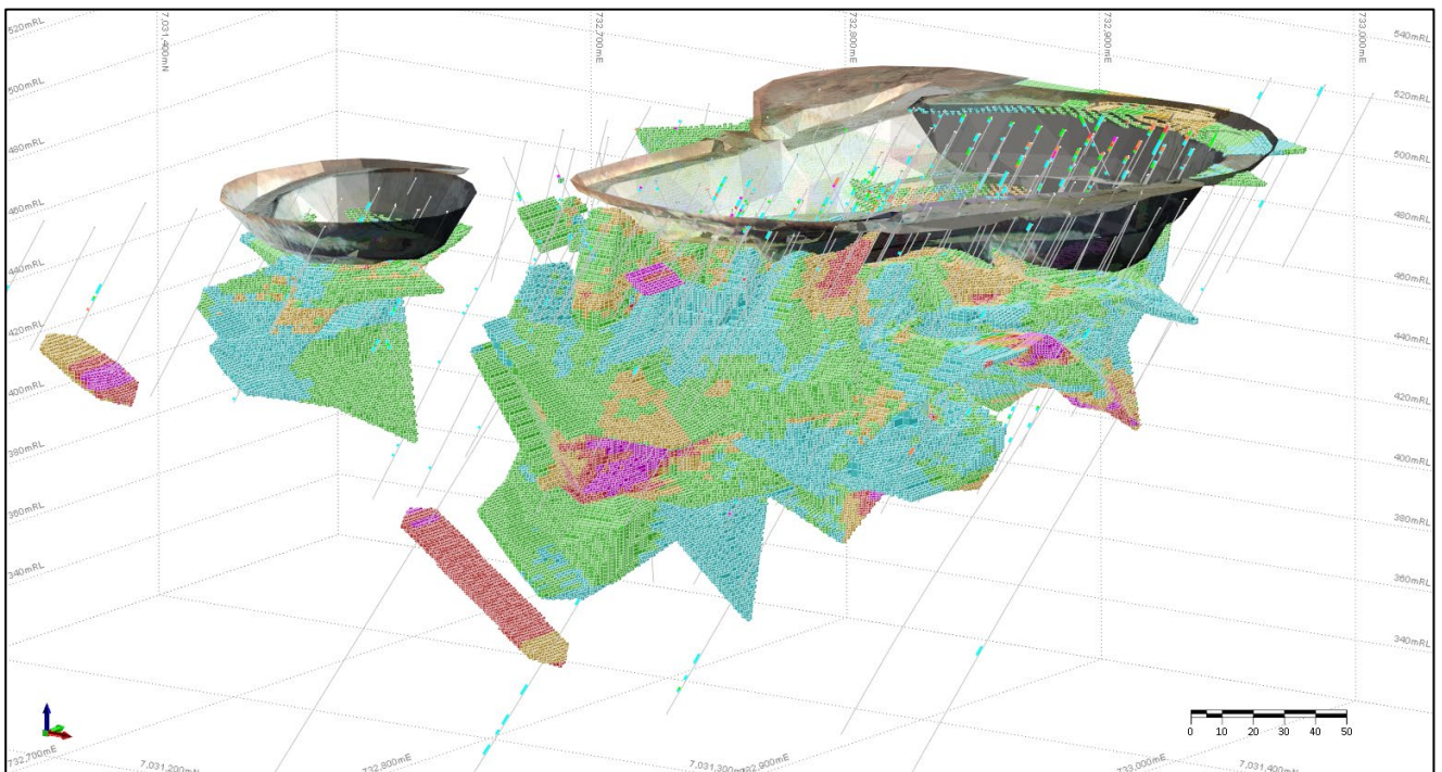
Figure 18: Toedter 3D view looking down to the north-west showing drill holes, mined open pits, and OK block model coloured by Au (g/t)
