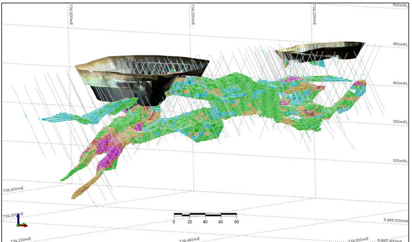
Figure 24: Wedge 3D view looking down to the north-west showing drill holes, mined open pits, and OK block model coloured by Au (g/t)
