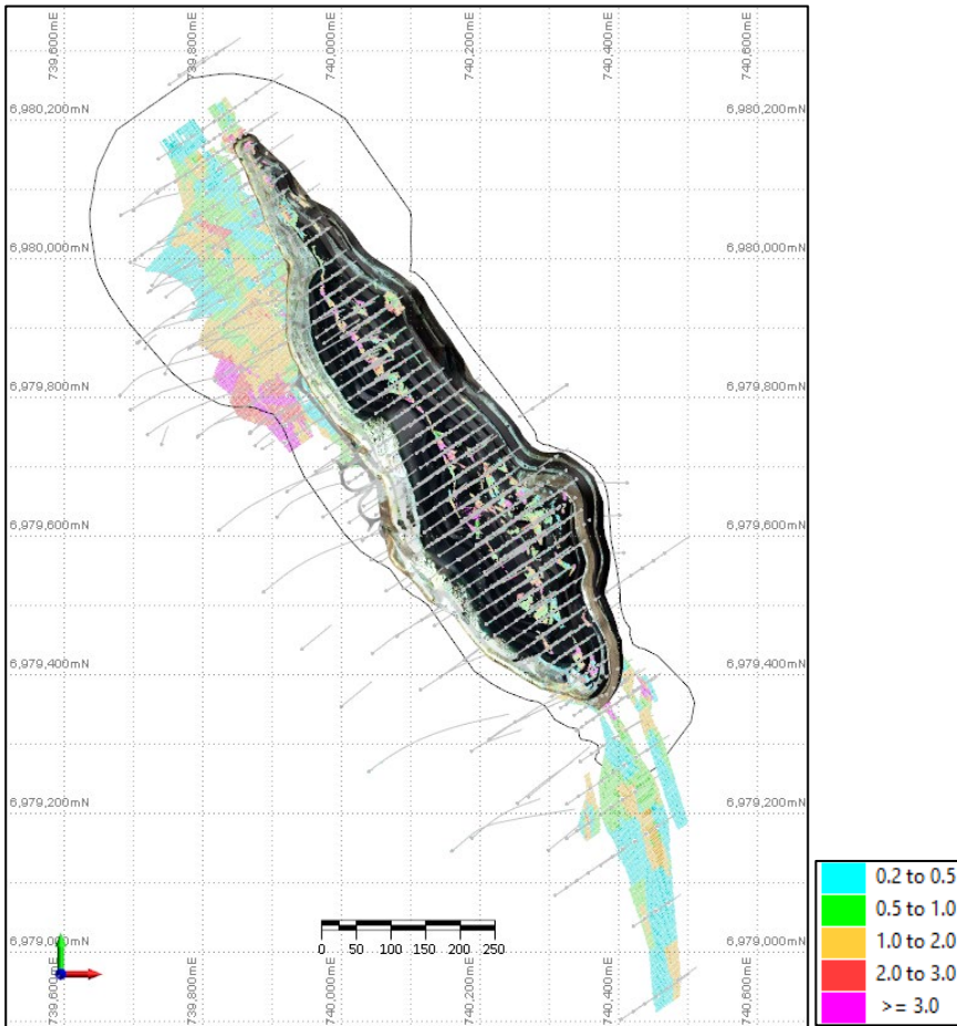
Figure 9: Kingfisher drill hole plan showing mined open pit, OK resource block model coloured by Au (g/t) and A$4,500 optimised pit shell (grey outline)
