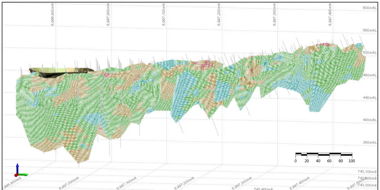
Figure 14: Shiraz 3D view looking down to the west-south-west showing drill holes, mined open pits, and OK block model coloured by Au (g/t)
