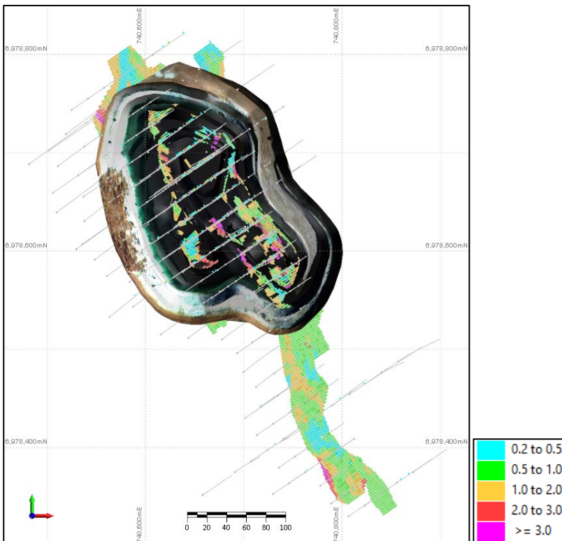
Figure 19: Hawk drill hole plan showing mined open pit and OK resource block model coloured by Au (g/t)
