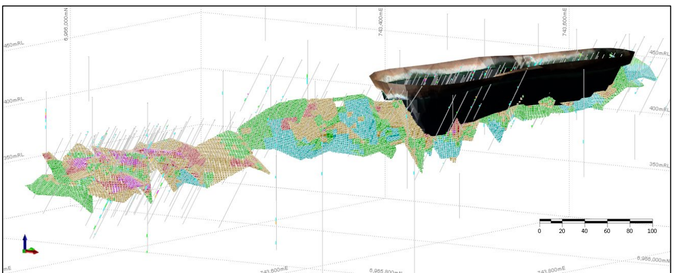
Figure 30: Deep South Reliance 3D view looking down to the north-west showing drill holes, mined open pit and OK block model coloured by Au (g/t)
