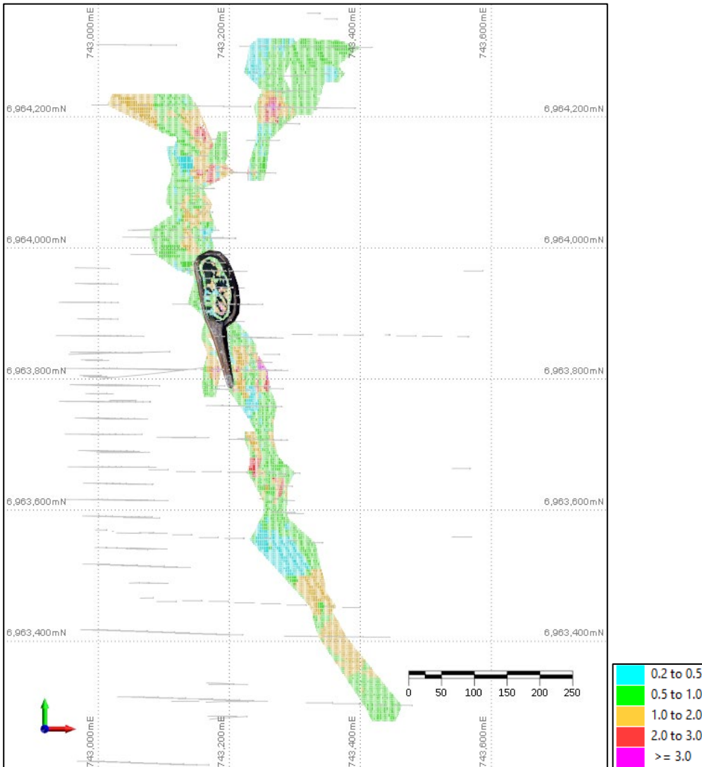
Figure 15: Think Big drill hole plan showing mined open pit and OK resource block model coloured by Au (g/t)
