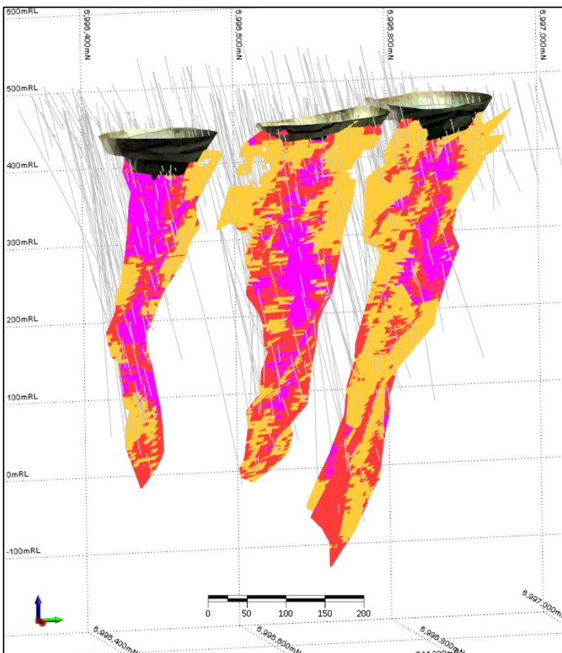
Figure 6: Wilsons 3D view looking down to the west-north-west showing drill holes, mined open pits, and OK block model coloured by Au (g/t)
