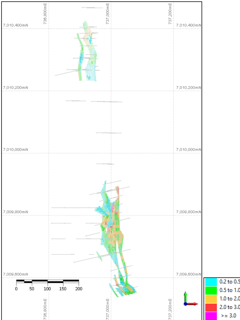
Figure 25: Melbourne Bitter drill hole plan and OK resource block model coloured by Au (g/t)
