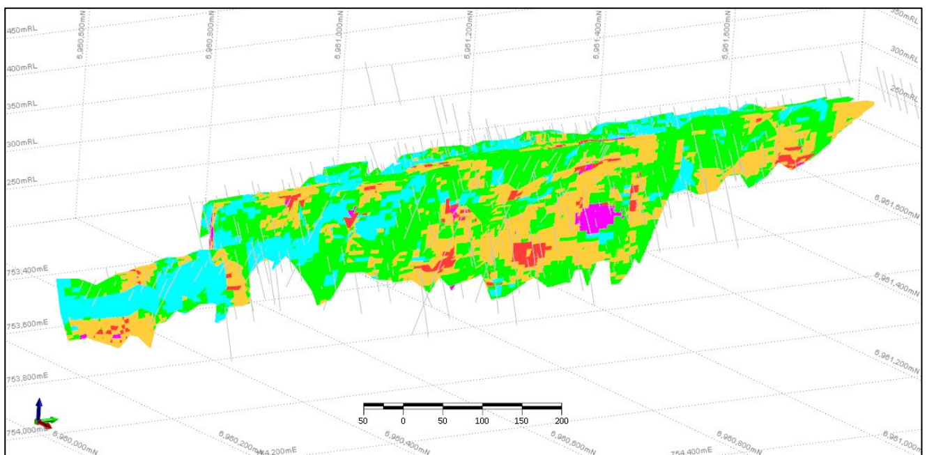
Figure 8: Howards 3D view looking down to the north-west showing drill holes and OK block model coloured by Au (g/t)
