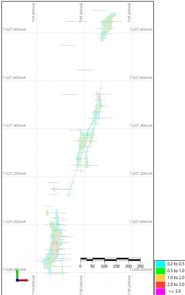
Figure 21: Specimen Well drill hole plan and OK resource block model coloured by Au (g/t)
