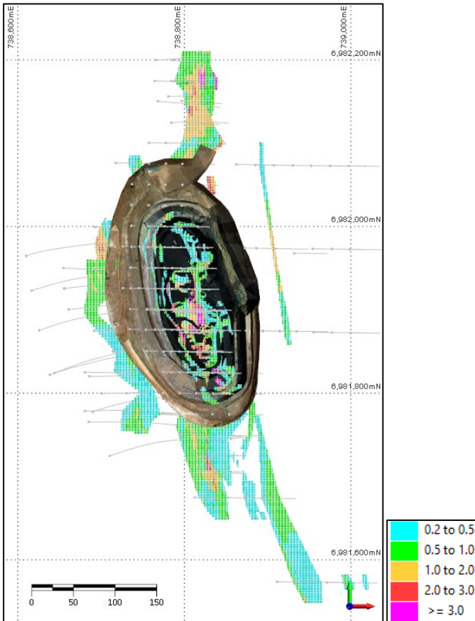
Figure 11: Eagle drill hole plan showing mined open pit and OK resource block model coloured by Au (g/t)
