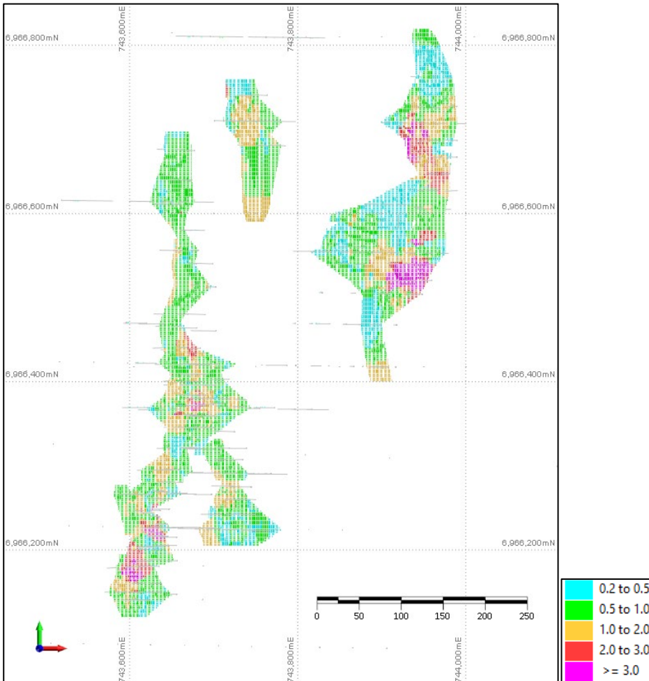
Figure 27: Hyperno-Reliance drill hole plan and OK resource block model coloured by Au (g/t)
