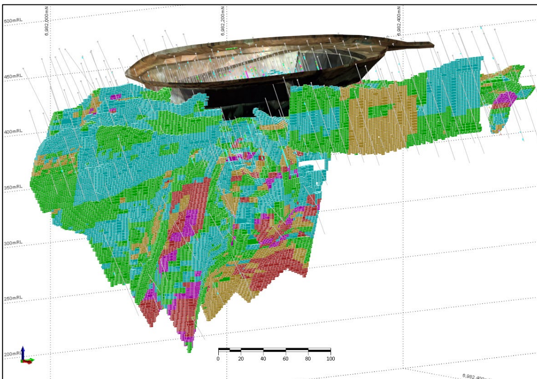
Figure 12: Eagle 3D view looking down to the north-west showing drill holes, mined open pit, and OK block model coloured by Au (g/t)
