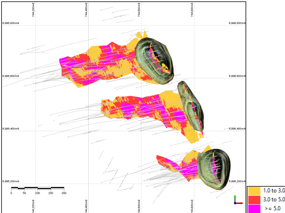
Figure 5: Wilsons drill hole plan showing mined open pits and OK resource block model coloured by Au (g/t)
