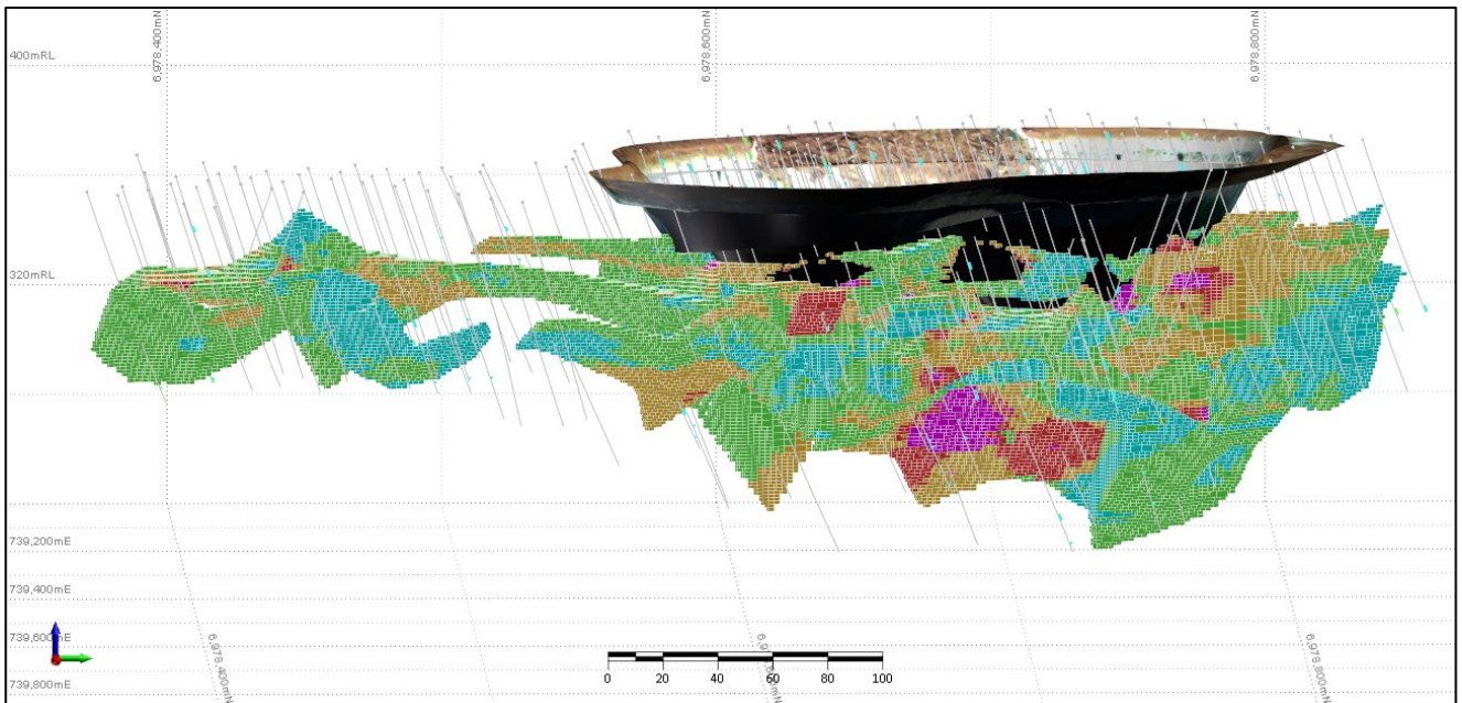
Figure 20: Hawk 3D looking down to the west-north-west showing drill holes and OK block model coloured by Au (g/t)
