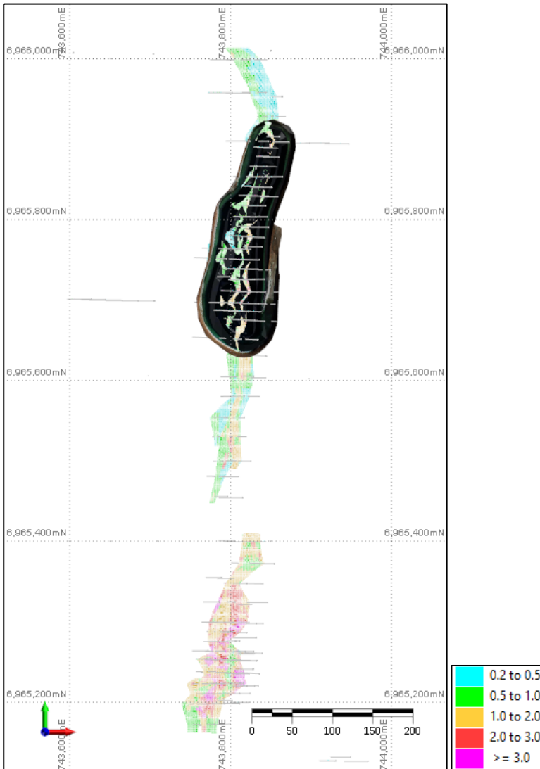
Figure 29: Deep South Reliance drill hole plan showing mined open pit and OK resource block model coloured by Au (g/t)
