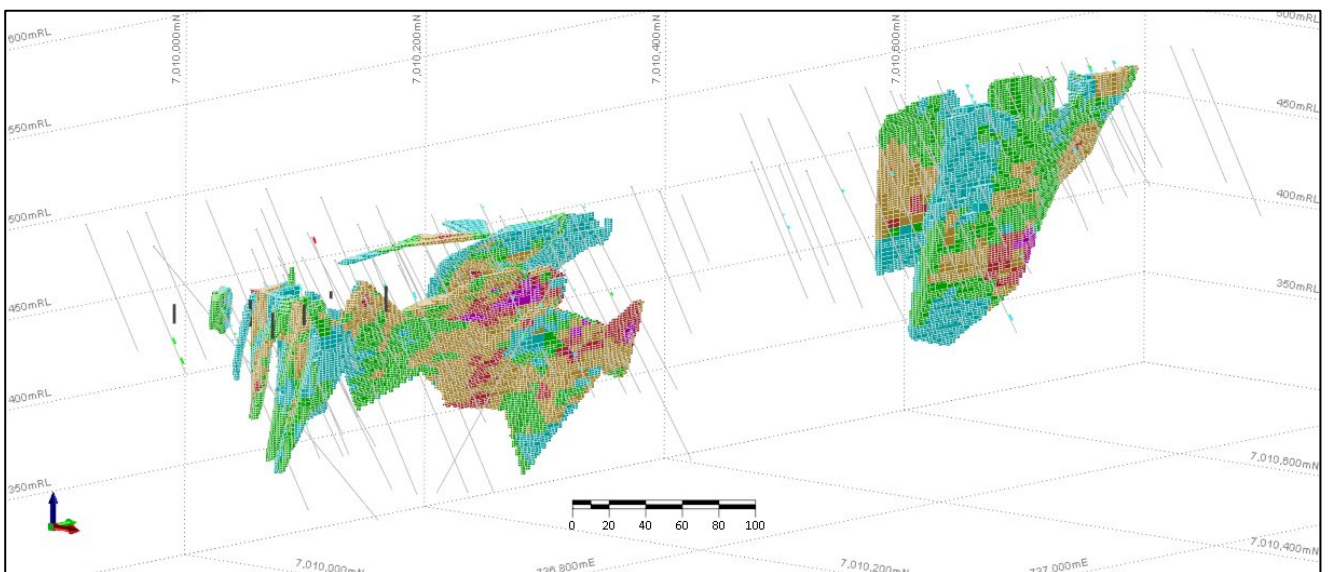
Figure 26: Melbourne Bitter 3D view looking down to the north-west showing drill holes, historic shafts (black), and OK block model coloured by Au (g/t)
