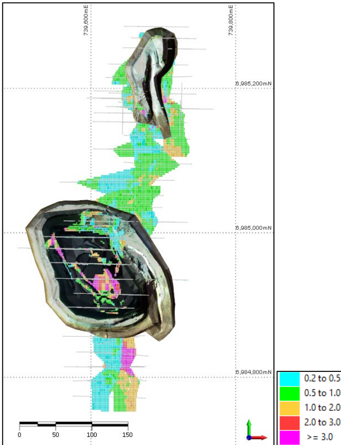
Figure 23: Wedge drill hole plan drill hole plan showing mined open pits and OK resource block model coloured by Au (g/t)
