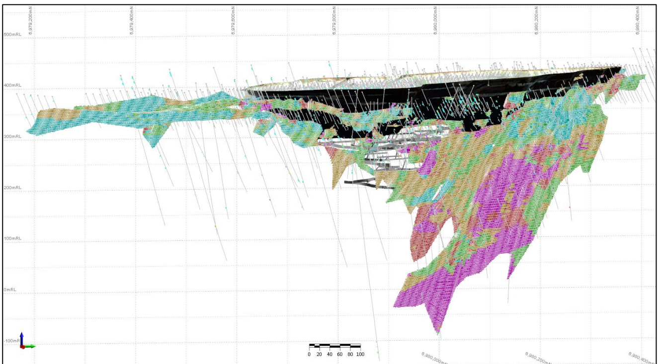
Figure 10: Kingfisher 3D view looking down to the west-north-west showing drill holes, mined open pit, underground workings and OK block model coloured by Au (g/t)
