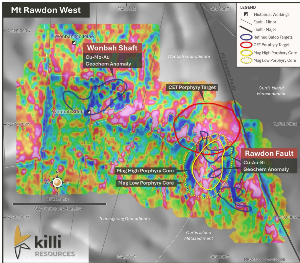
Figure 6: Colour first vertical derivative (IVD) ground magnetic image successfully demarcating the contact between the Wonbah and Tennifering Granodiorites. The significant magnetic high and lows highlight the high degree of fluid flow along the contacts. Also the interpreted indicative characteristics of a porphyry system associated with the contacts of the Wonbah/Tennifering Granodiorites and the older Curtis Island Metasediments proximal to the Mt Rawdon Fault and geochemical target area - Rawdon Fault.
