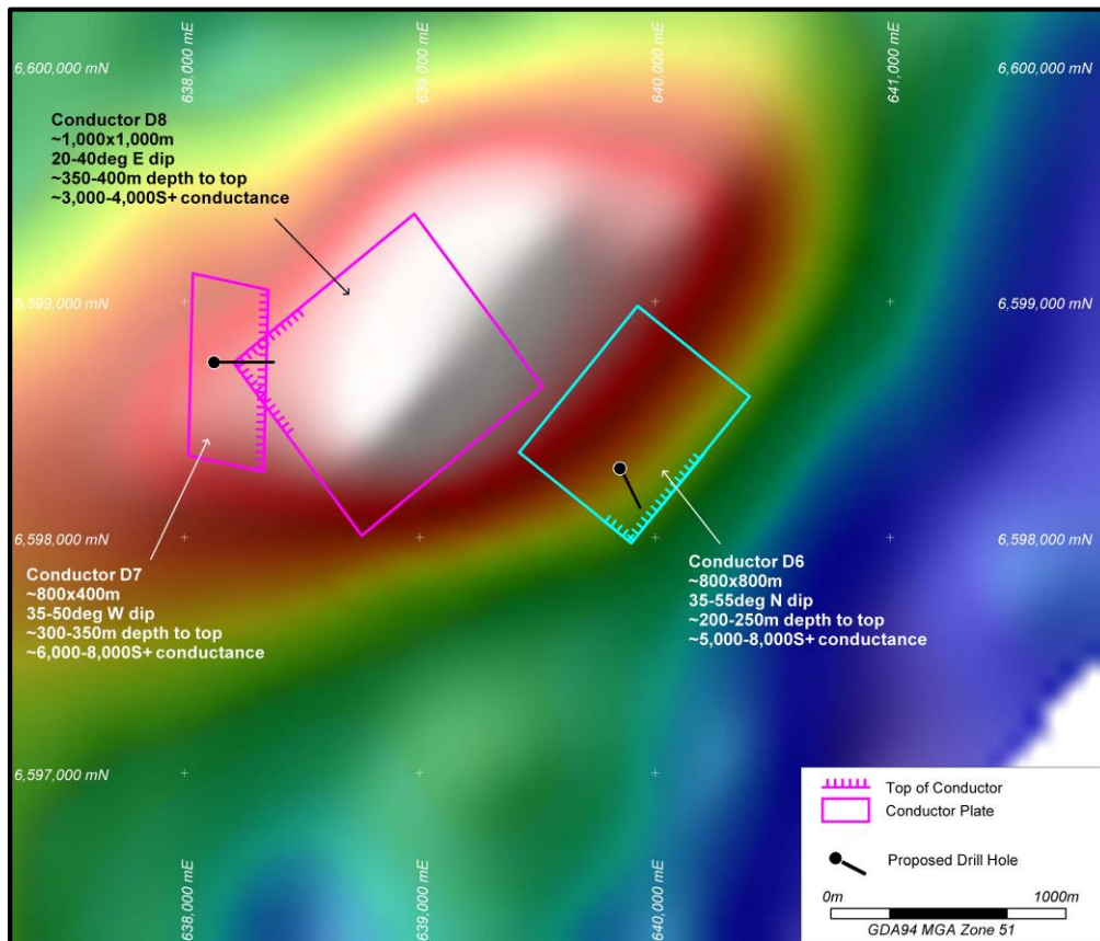
Figure 1: Proposed Drillholes on FLTEM Conductor Plates (Residual Gravity)
