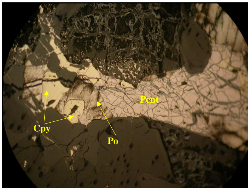
Photo 1: Gabbronorite containing pentlandite (Pent), chalcopyrite (Cpy) and pyrrhotite (Po). BOH sample from RKAC183 (Field of view = 1.8 mm)
