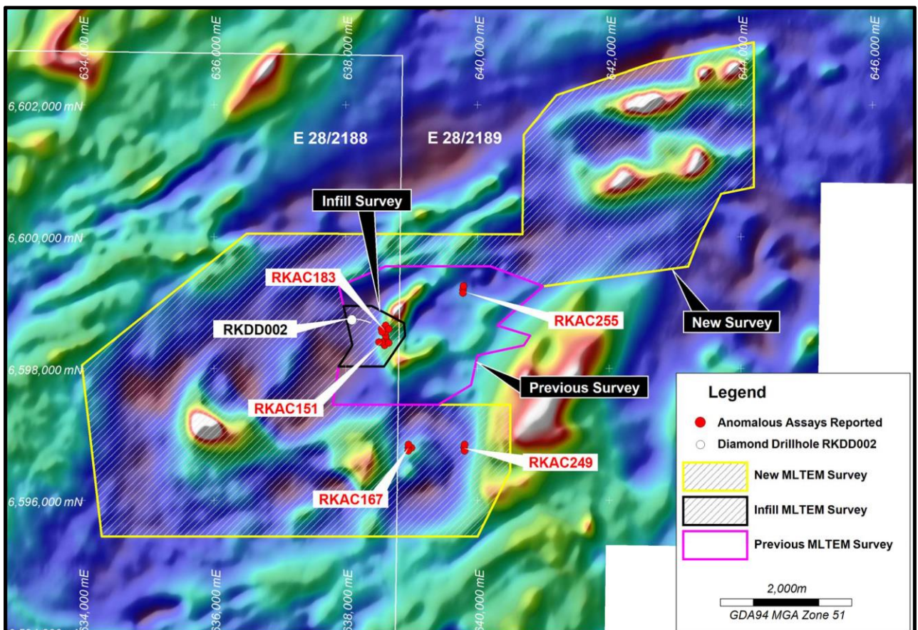
Figure 1: New MLTEM Survey – Area D
