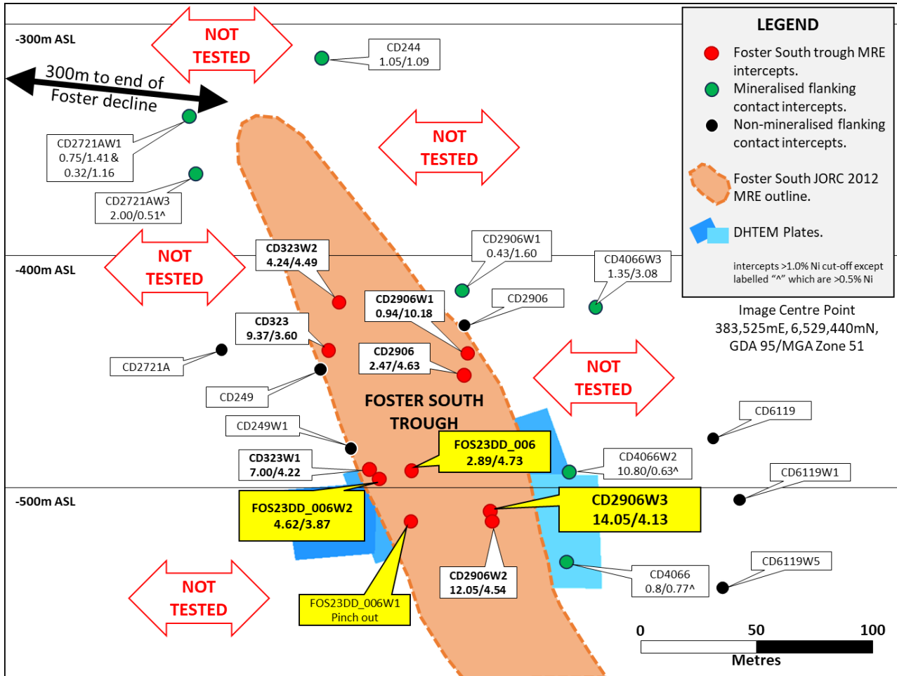
Figure 2: Long projection (looking northeast) of the Foster South deposit with latest Lunnon Metal metallurgical DD hole CD 2906W3 result and previous Lunnon Metal and WMC historical pierce points at the komatiite-basalt contact (see ASX announcement dated 9 October 2023 for full details of other drillholes shown).
