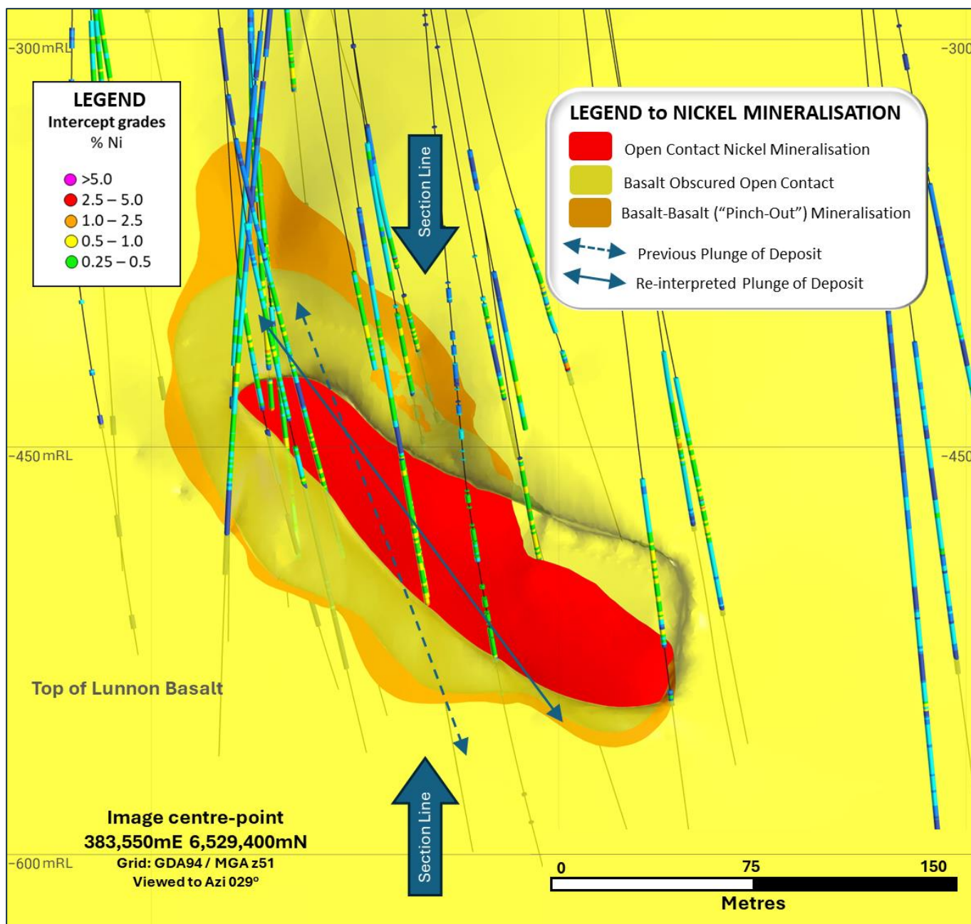
Figure 3: Isometric View (looking NNE) illustrating current and revised plunge orientation and geological interpretation of nickel sulphide mineralisation host position at Foster South (see Figure 4 for cross section indicated).
