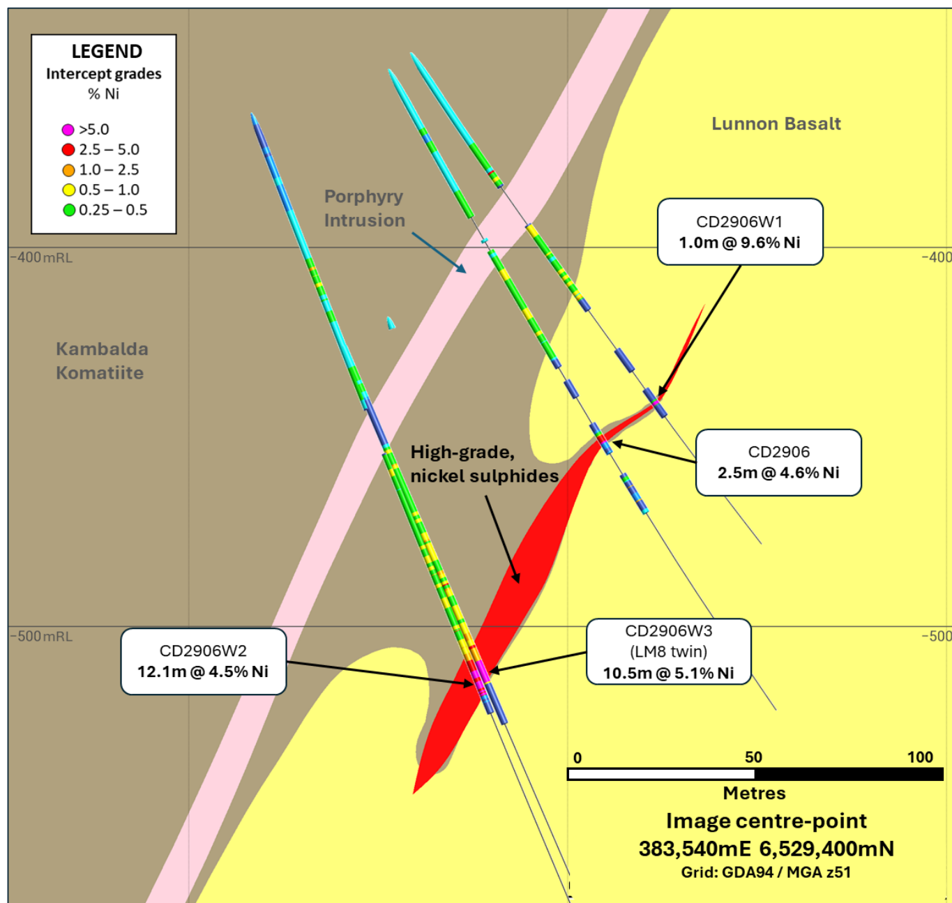
Figure 4: Geological cross section view through Foster South MRE looking north-west.
