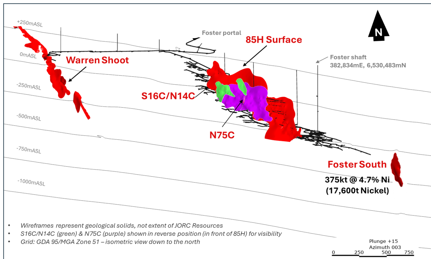
Figure 2: Isometric View of Foster Mine decline illustrating relative location of the unmined Foster South MRE 7 , to both the workings and the surface.
