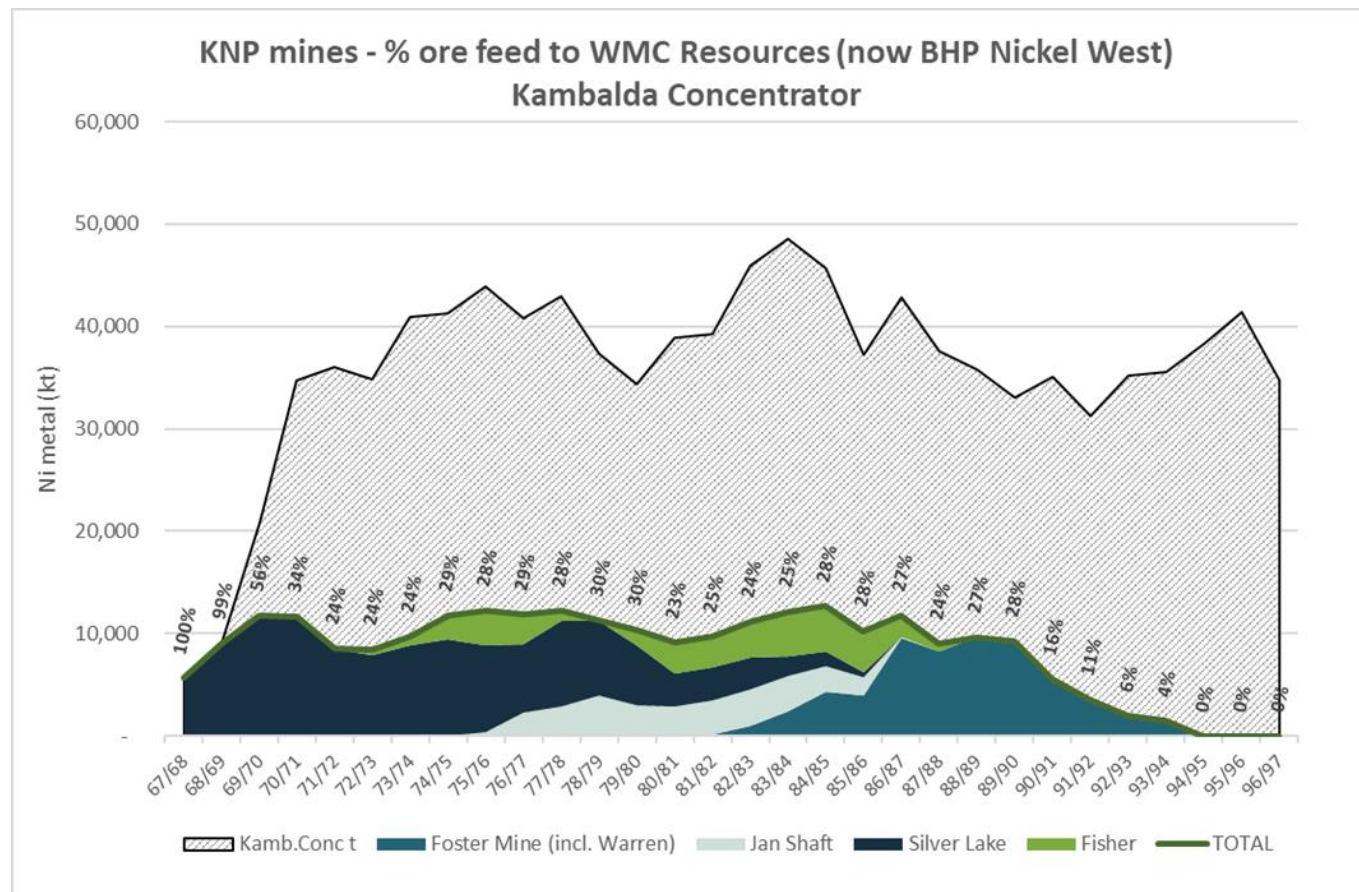
Figure 5: Historical nickel metal in ore fed to the Kambalda Concentrator (1967-1997), highlighting the contribution from nickel mines now in Lunnon Metals' portfolio 10 .
