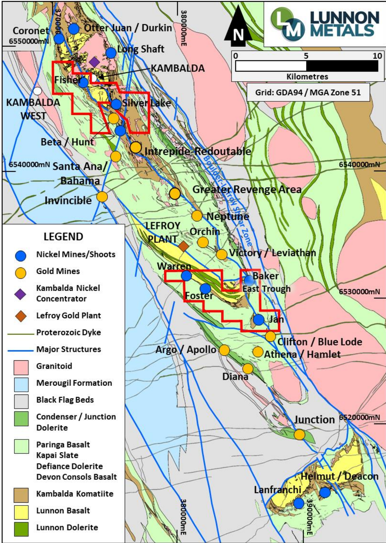
Figure 5: The KNP (red outlines) with Kambalda regional geology and location of key nickel and gold mines/infrastructure.
