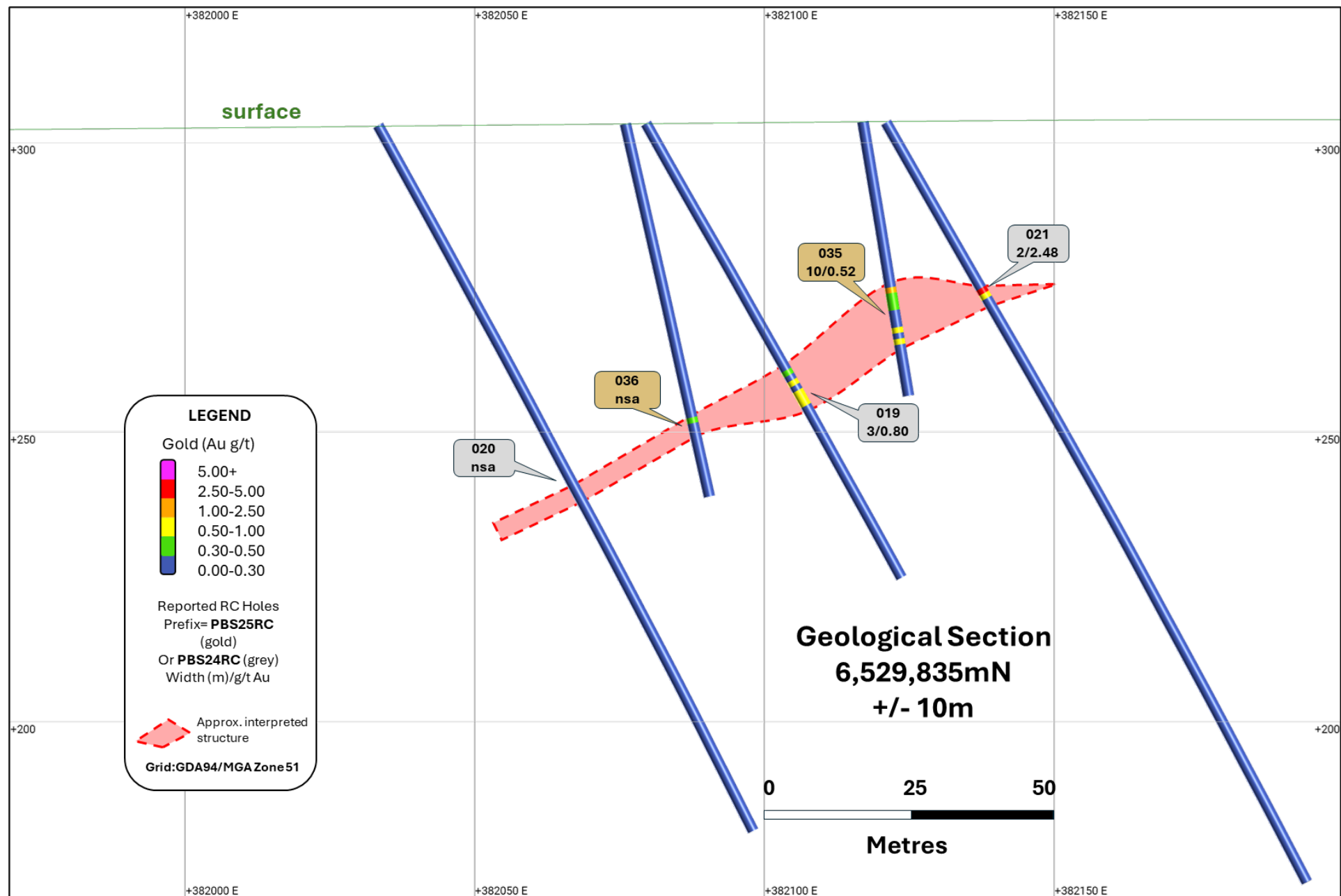
Figure 6: Section 6,529,835mN (looking north +/- 10m) illustrating the results reported today (gold call-outs) and prior reported results (grey call-outs).
