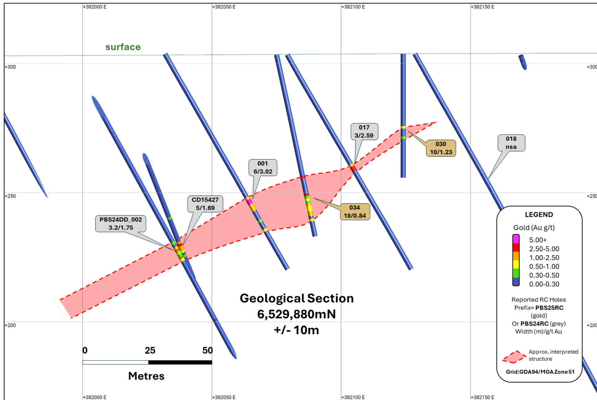
Figure 4: Section 6,529,880mN (looking north +/- 10m) illustrating the results reported today (gold call-outs) and prior reported results (grey call-outs).
