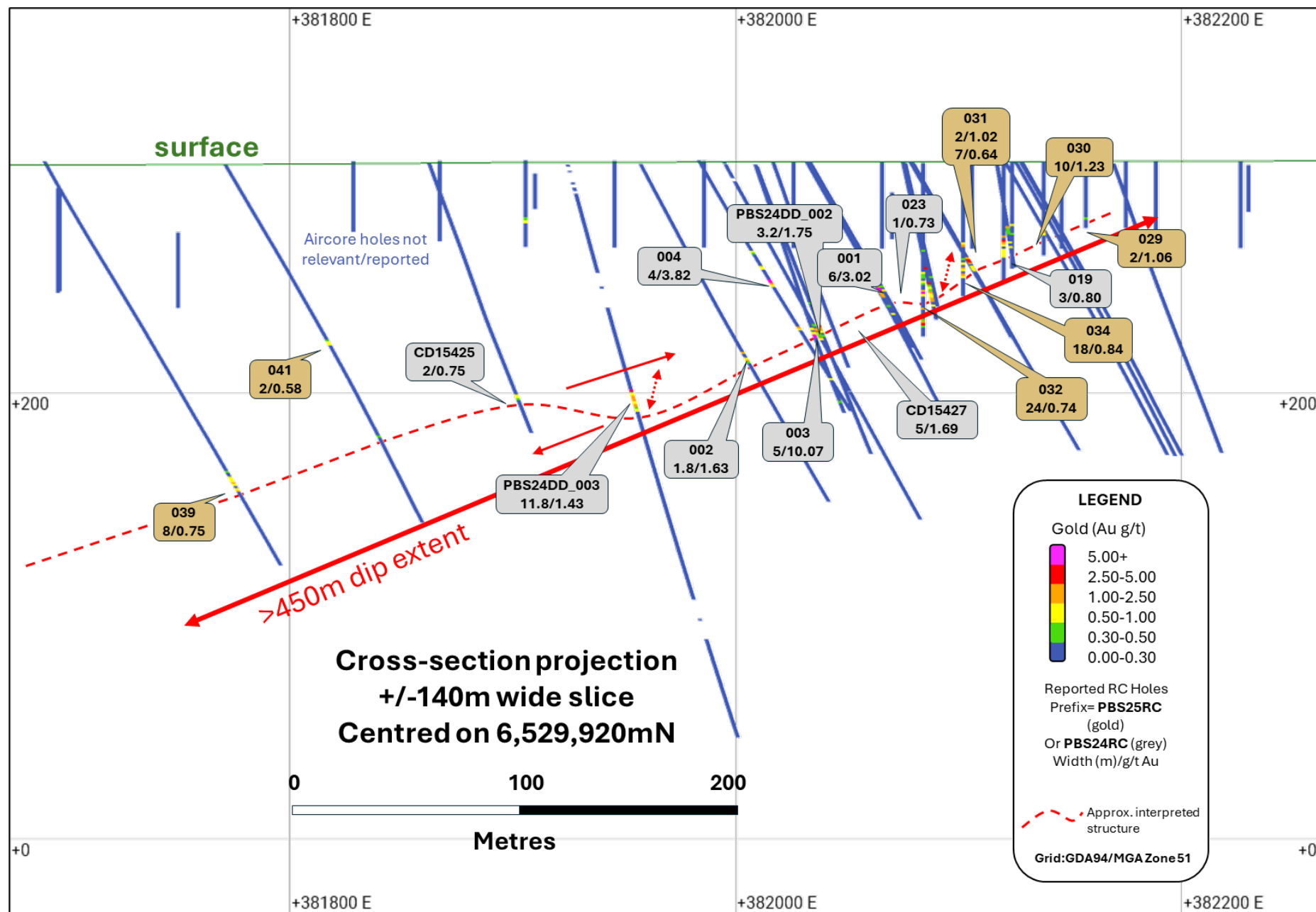
Figure 3: Cross-section centred on 6,529,920mN (looking north +/- 140m) illustrating the results reported today (gold call-outs) and prior reported results (grey call-outs).
