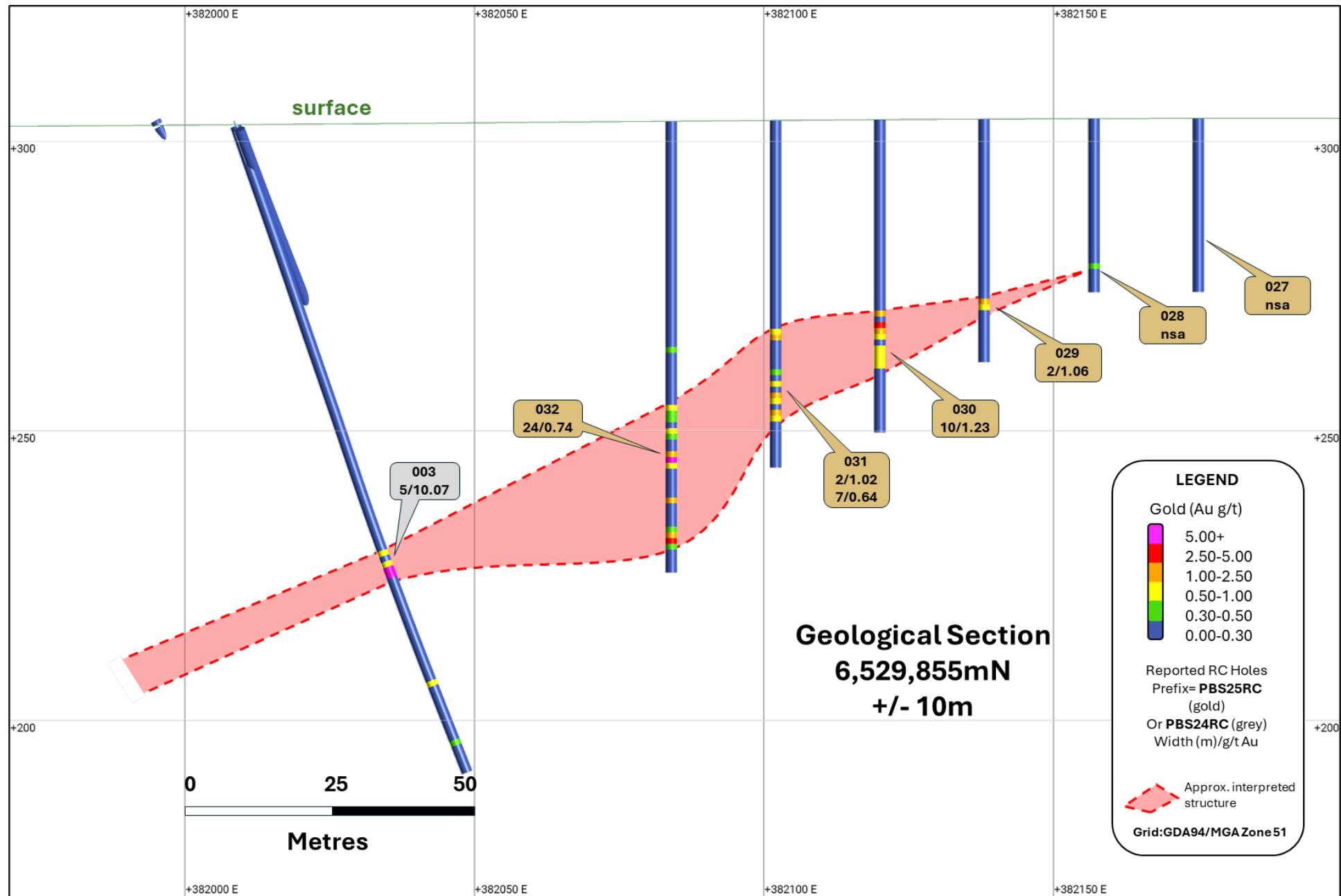
Figure 5: Section 6,529,855mN (looking north +/- 10m) illustrating the results reported today (gold call-outs) and prior reported results (grey call-outs).
