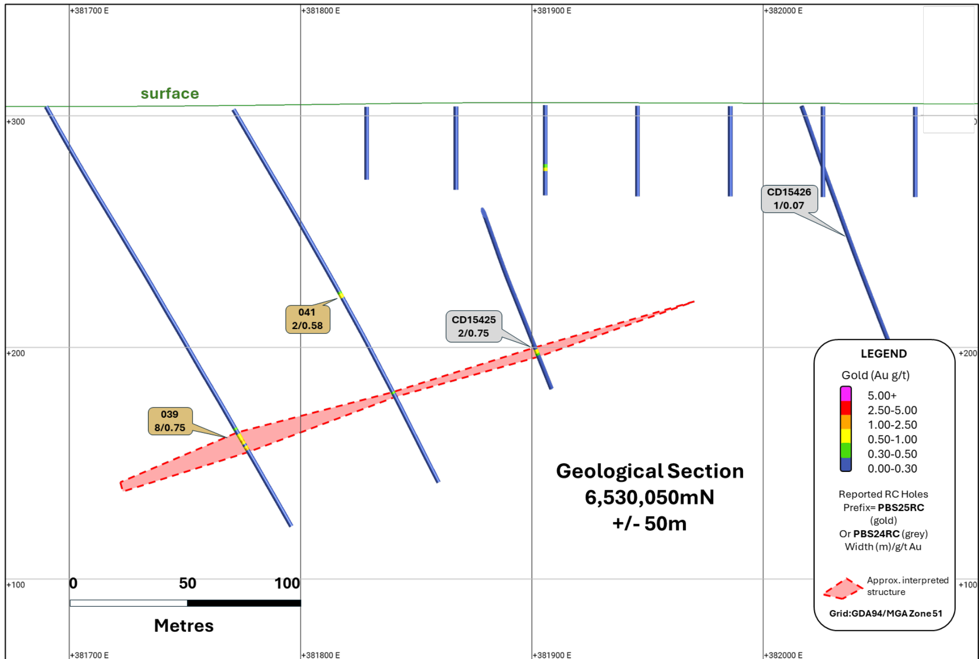
Figure 7: Section 6,530,050mN (looking north +/- 50m) illustrating the results reported today (gold call-outs) and prior reported results (grey call-outs).
