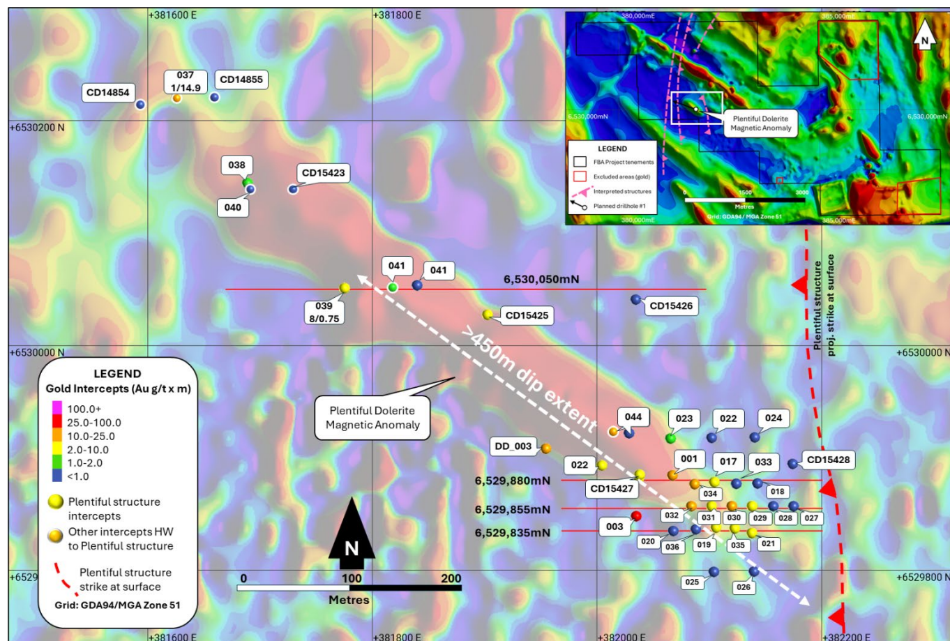
Figure 2: Plan view of the Plentiful dolerite and gold prospect area, showing drill hole IDs and section lines of Figures 4 to 7 , over ground magnetic image (reduced to pole – 1 st vertical derivative) with insert displaying location at the project scale and the first planned Plentiful EIS hole.
