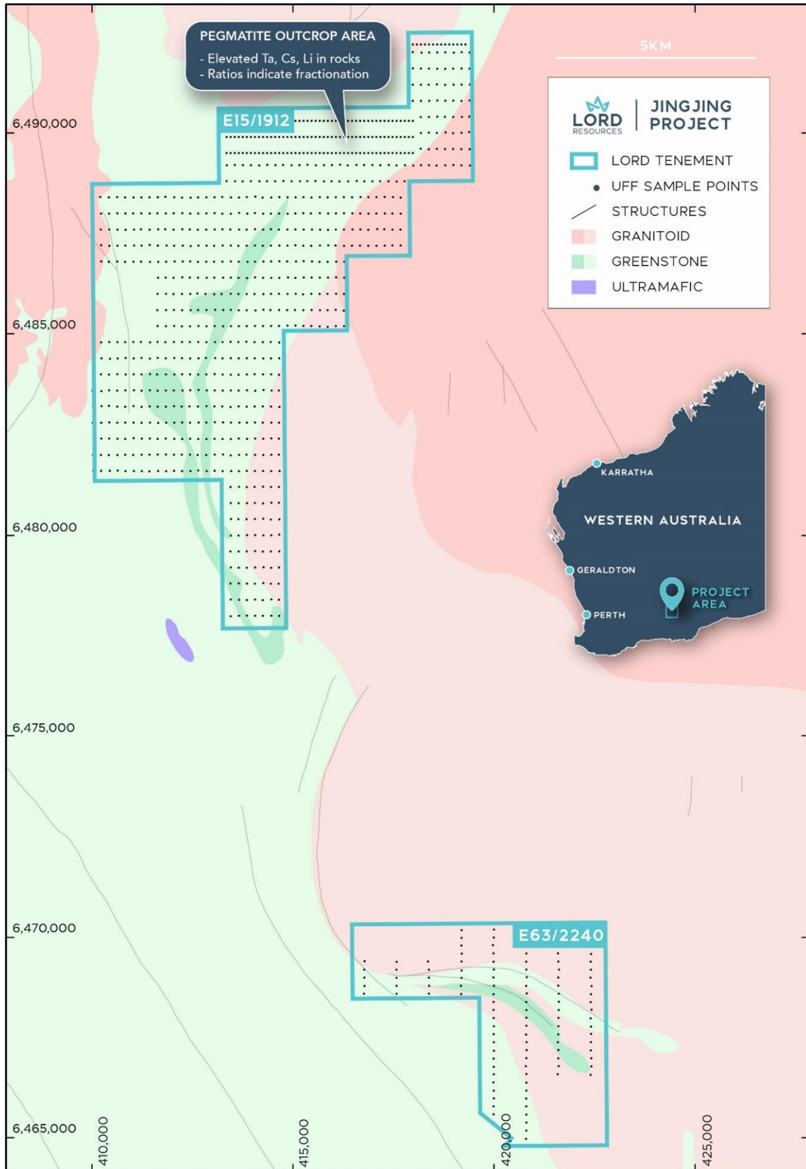
Figure 3 - Jingjing Project area showing sample locations over simplified geology.
