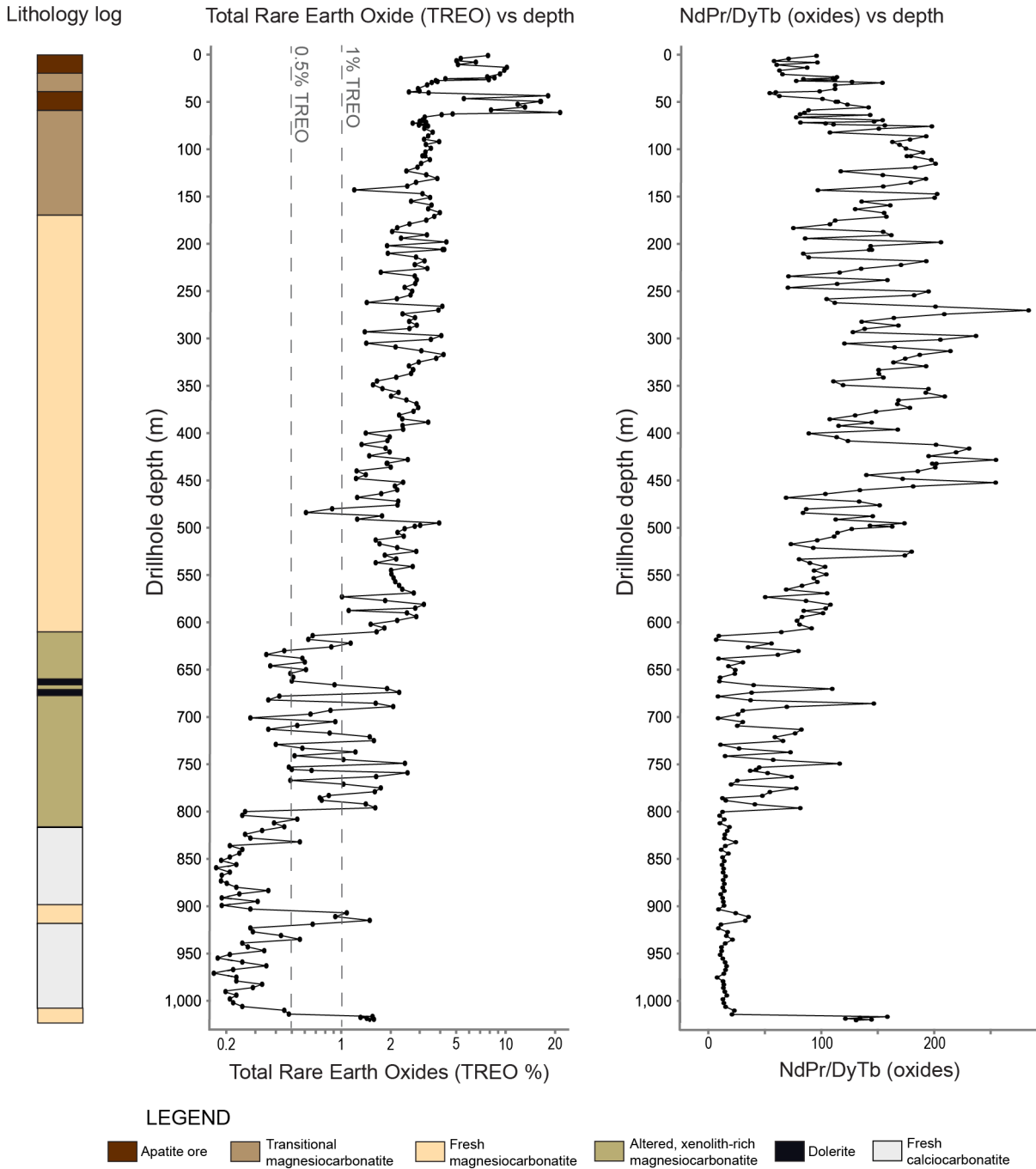
Figure 9 Downhole lithology correlated to total REO% and ratio between Light Rare Earth Elements Nd, Pr and Heavy Rare Earth Elements Dy and Tb. NdPr/DyTb oxide ratio of less than 40 implies relative enrichment of HREE
