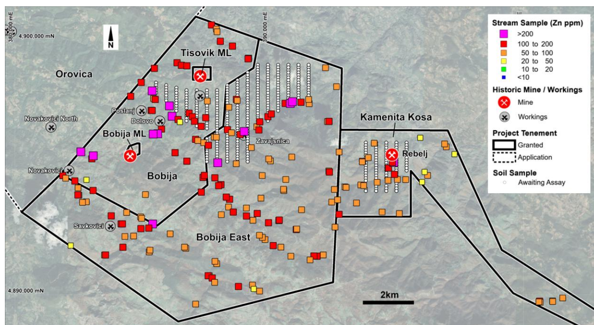
Figure 3: Stream sediment sample results across the Bobija Project area (showing Zn ppm) and location of current soil sampling programs.
