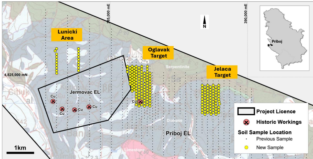
Figure 1: Central Priboj area showing location of new soil sample results.
