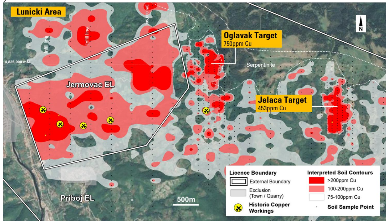
Figure 5: Central Priboj Project area showing priority target areas and copper-in-soil anomalism (anomaly values shown in ppm Cu represent average of soil sample results within +200ppm Cu contour).
