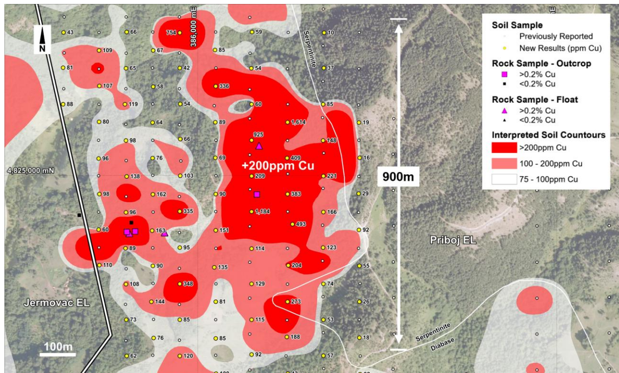
Figure 4: Oglavak Target – Soil sample results and location of rock chip samples.
