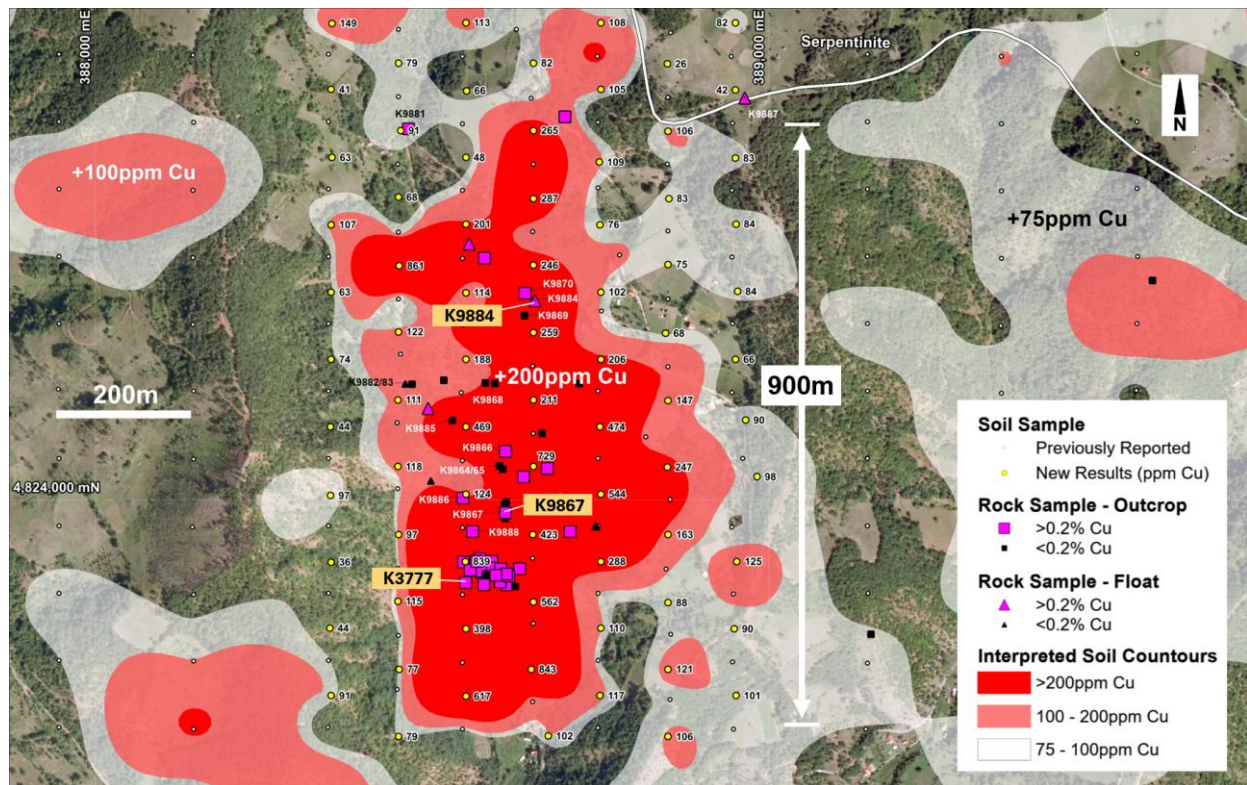
Figure 2: Jelaca Target - Soil sample results and location of rock chip samples.
