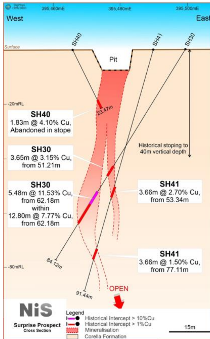
Figure 4: Cross section through the Surprise mine based on historical VAM drilling
