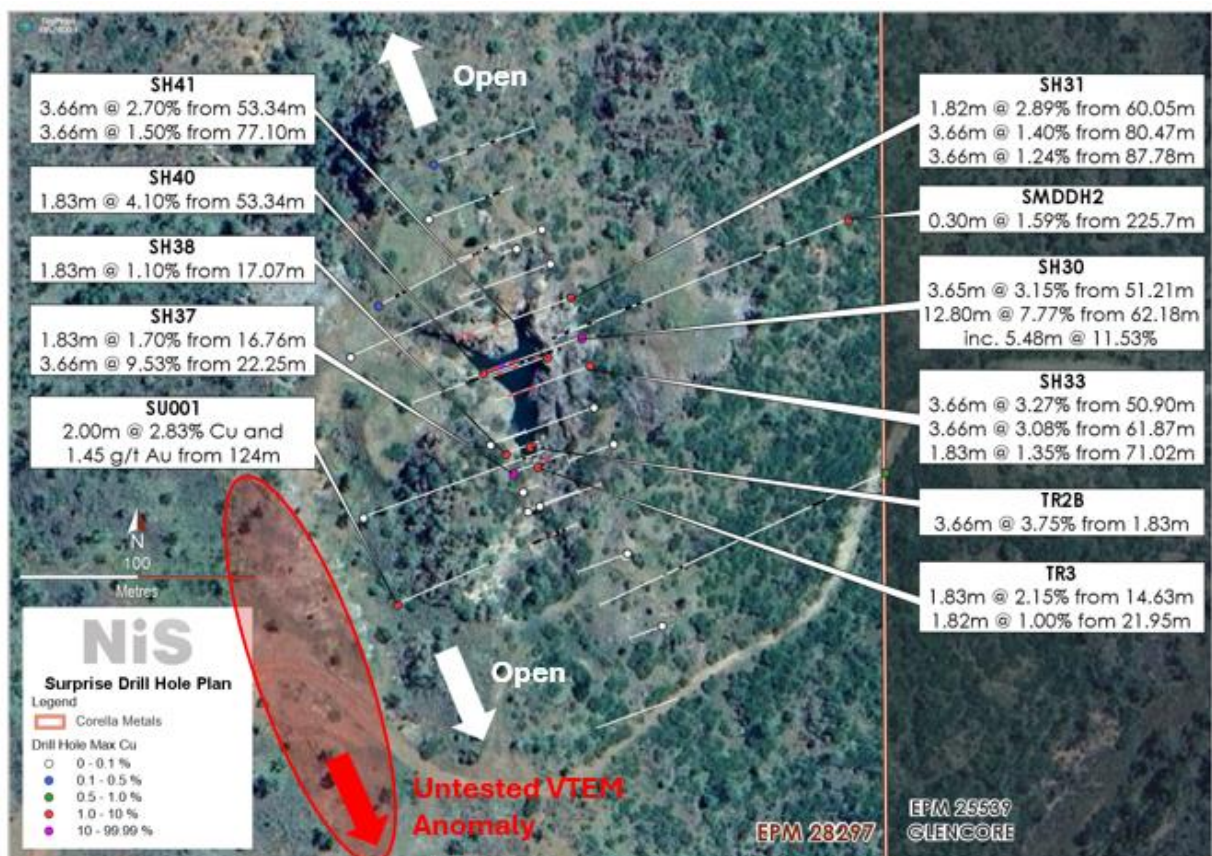
Figure 3: Surprise Mine Plan View outlining historical VAM drilling
