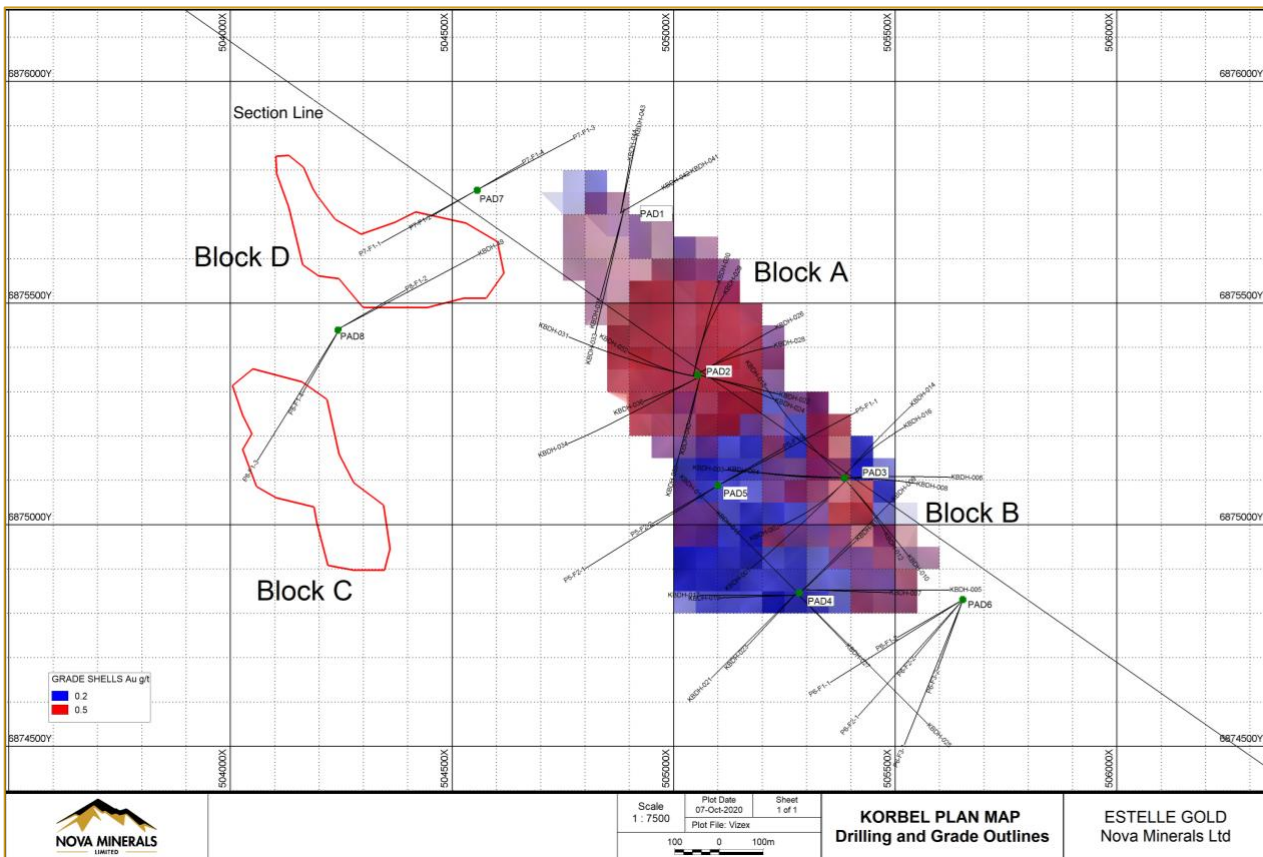
Figure 1. Plan view map of the Korbelt gold deposit illustrating the R/C and Diamond drill hole locations of Block A, B, C and D with a grade contours and IP Chargeability ( n=2 ).
