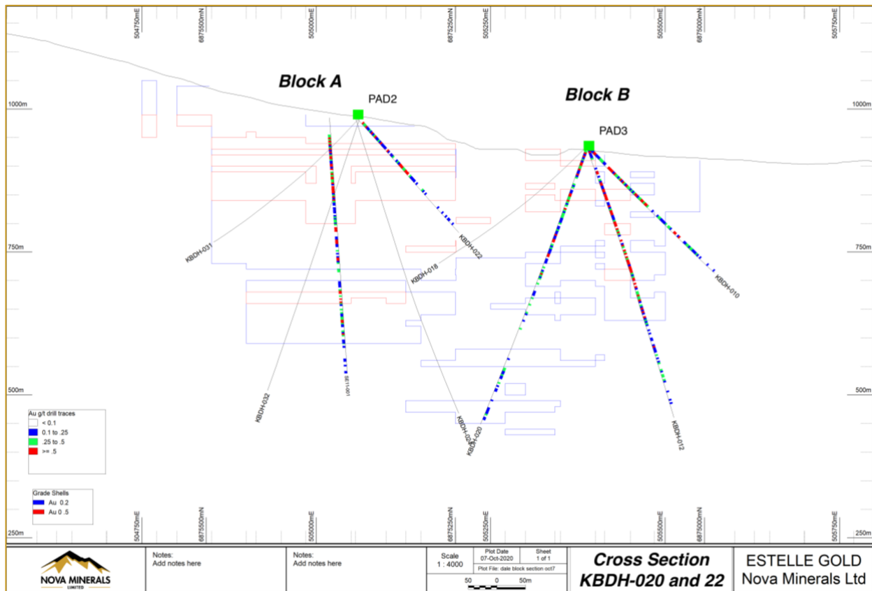
Figure 2. Cross Section KBDH-20 and 22
