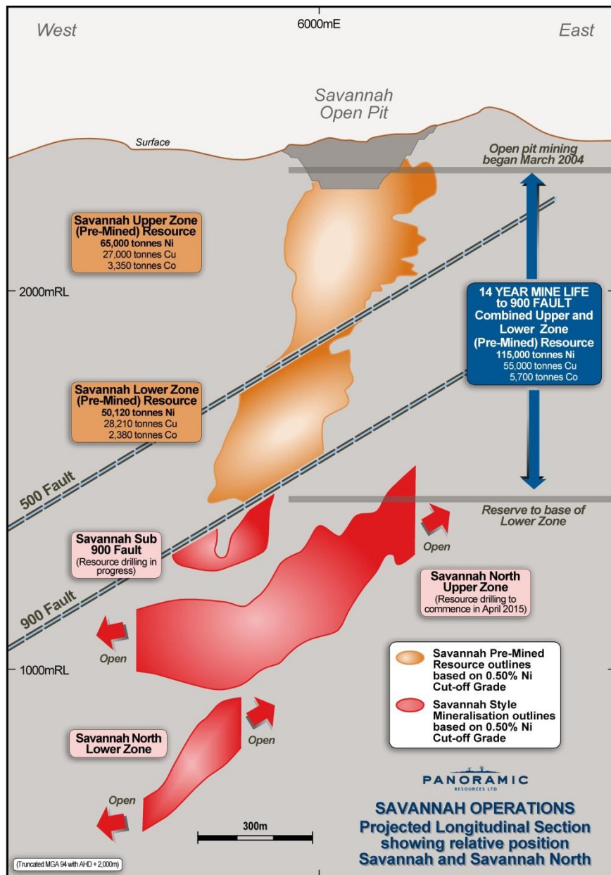
Long section looking North
