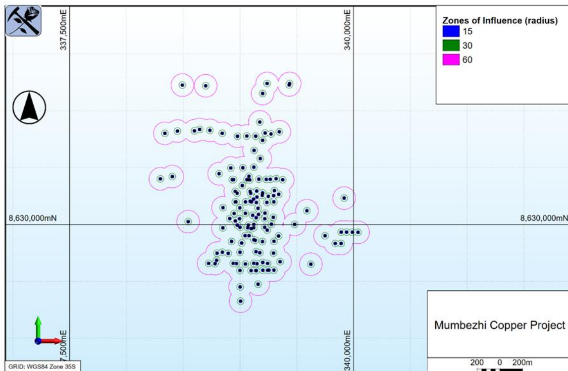
Figure 6: Plan showing zones of influence for Nyungu Central drilling – circles coloured by radius from drill collar
