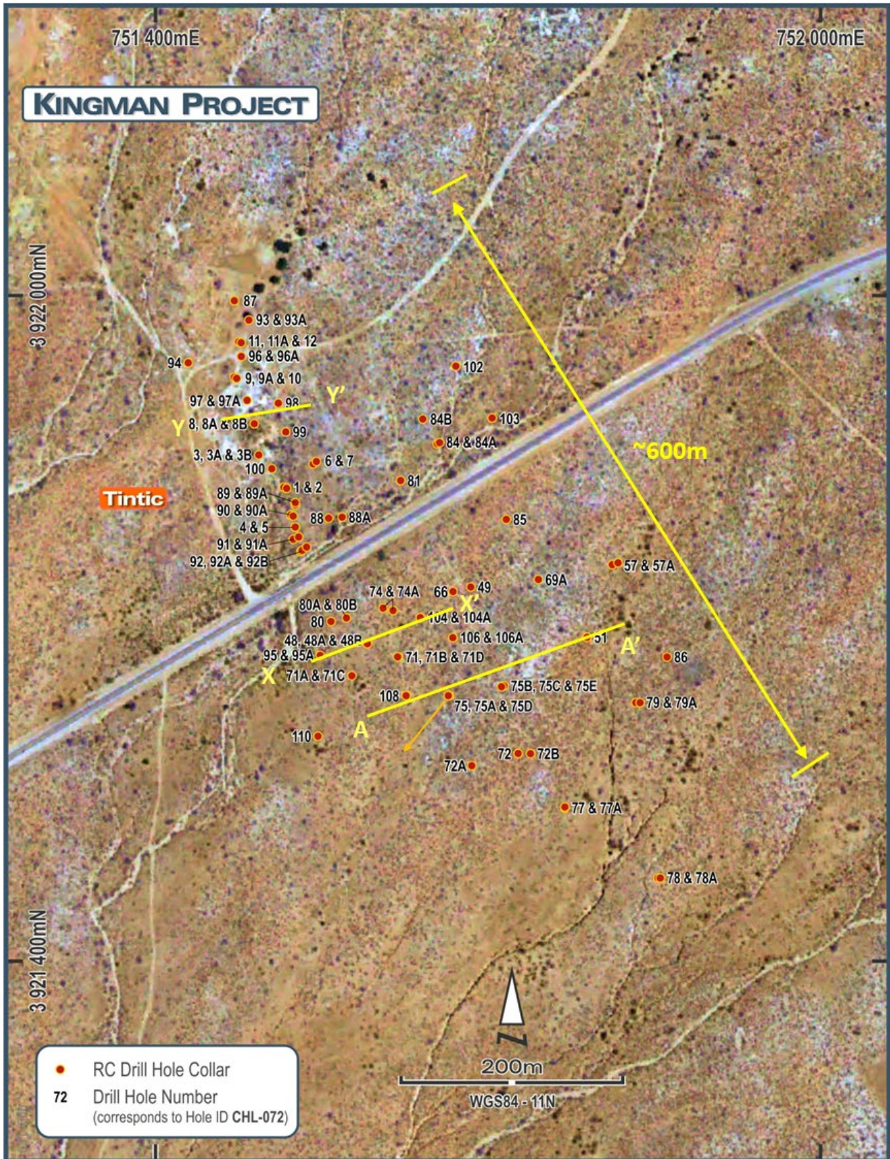
Figure 4 – RC hole collar locations over the Tintic area showing section lines & drill trace of hole CHL-075D which intersected 3.8m (downhole width) grading 18.1 g/t Au & 201 g/t Ag from 85.3m (approx. 60m below surface)
