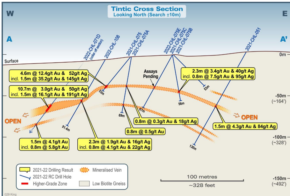
Figure 2 – Tintic RC Interpreted Drill Cross Section A-A' over ~250m width
