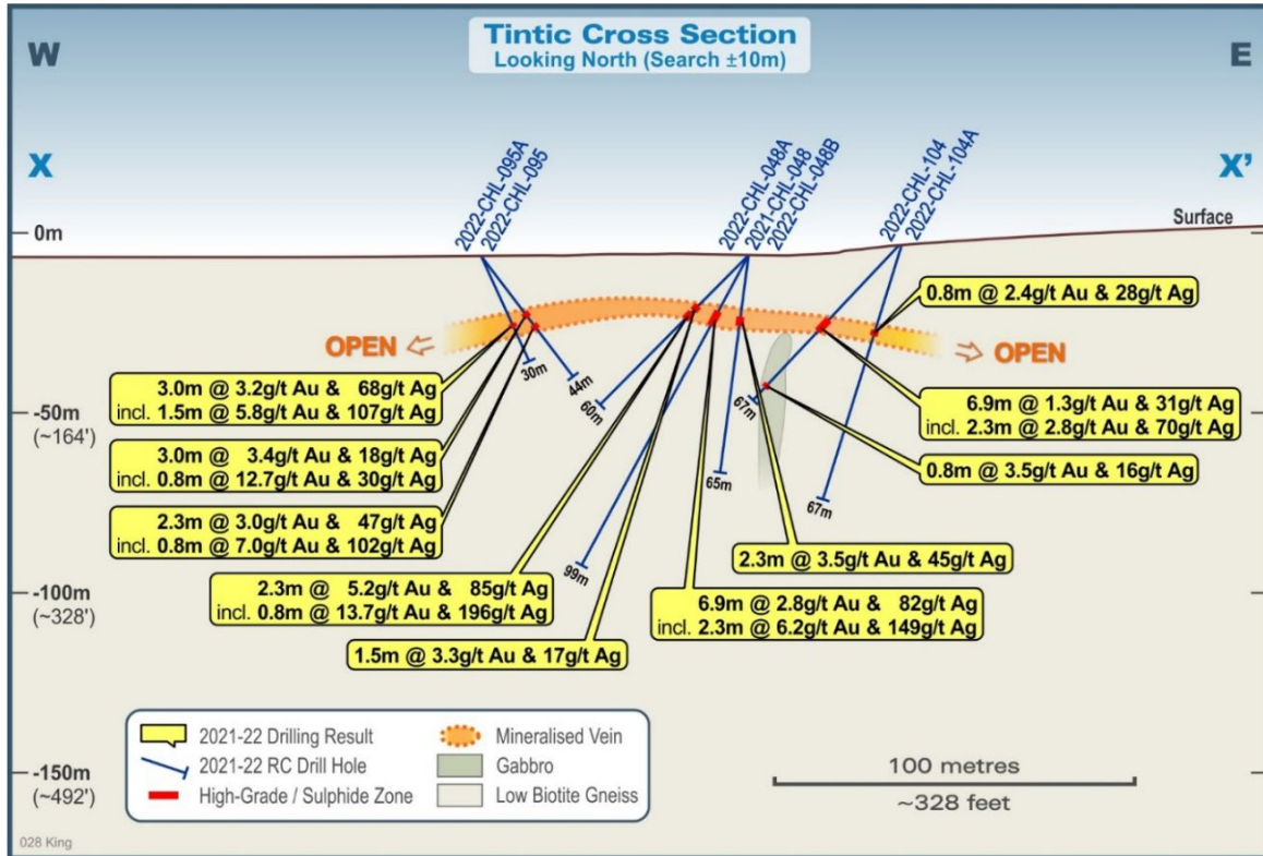
Figure 1 – Tintic RC Interpreted Drill Cross Section X-X' over ~100m width
