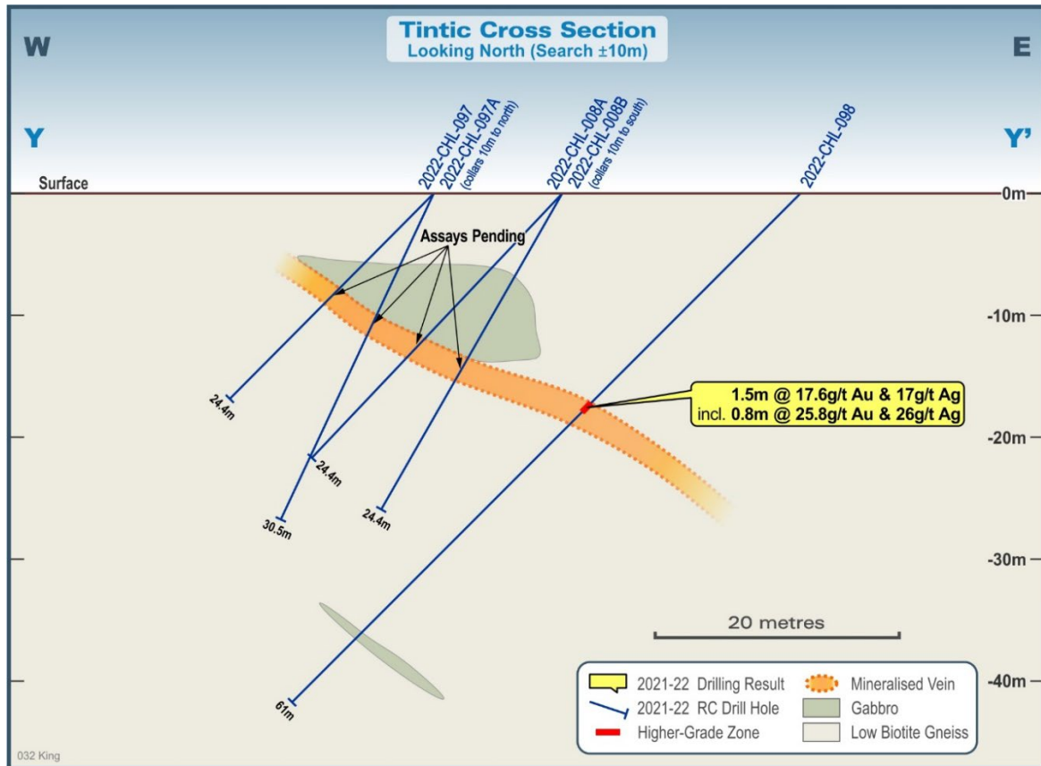
Figure 3 – Tintic RC Interpreted Drill Cross Section Y-Y'
