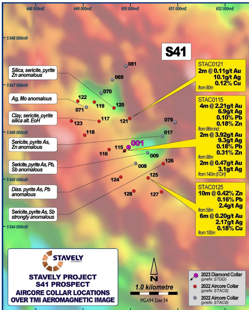
Figure 2. S41 gold prospect collar location map.
