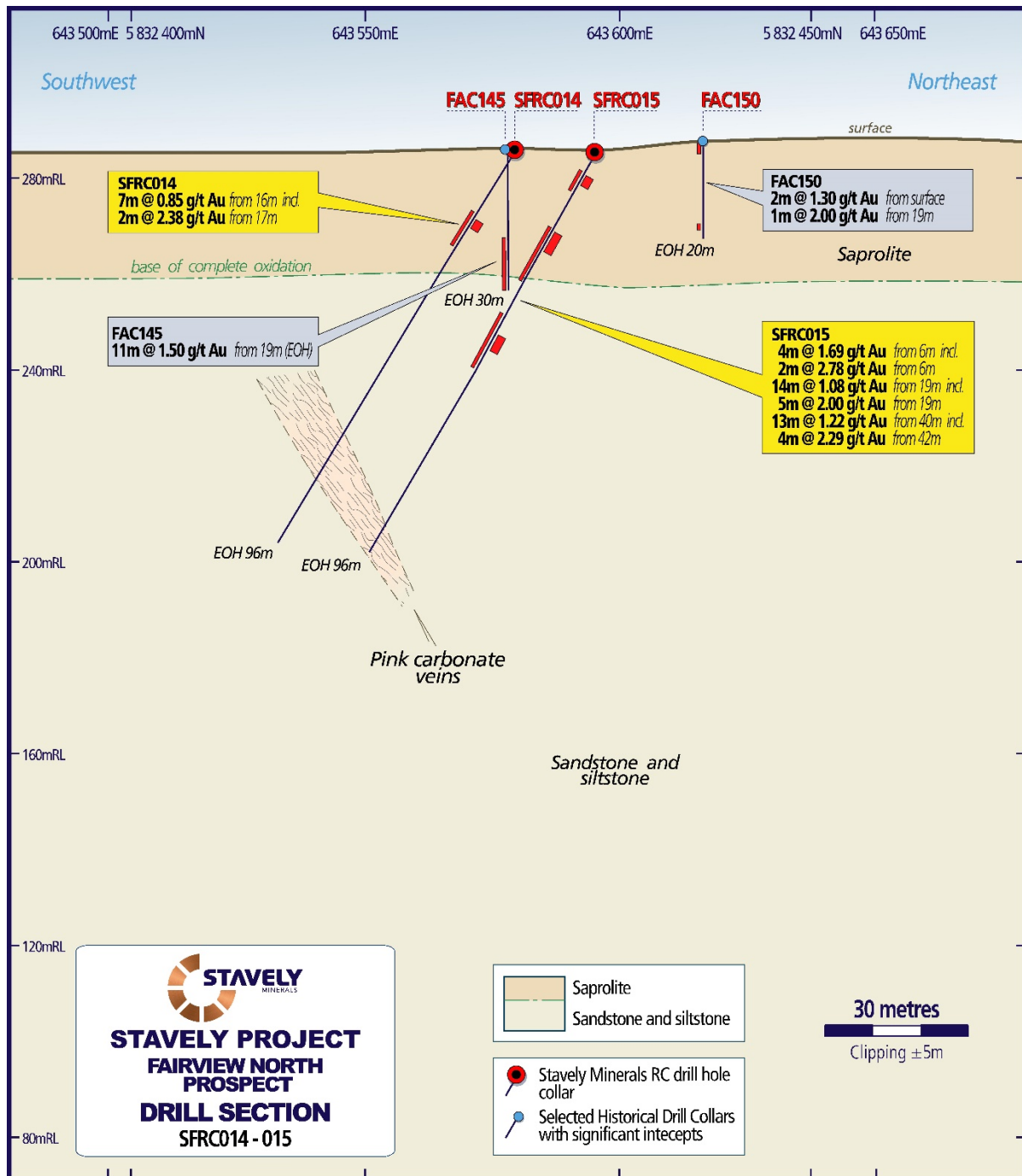
Figure 6. SFRC014 and SFRC015 drill hole cross section.
