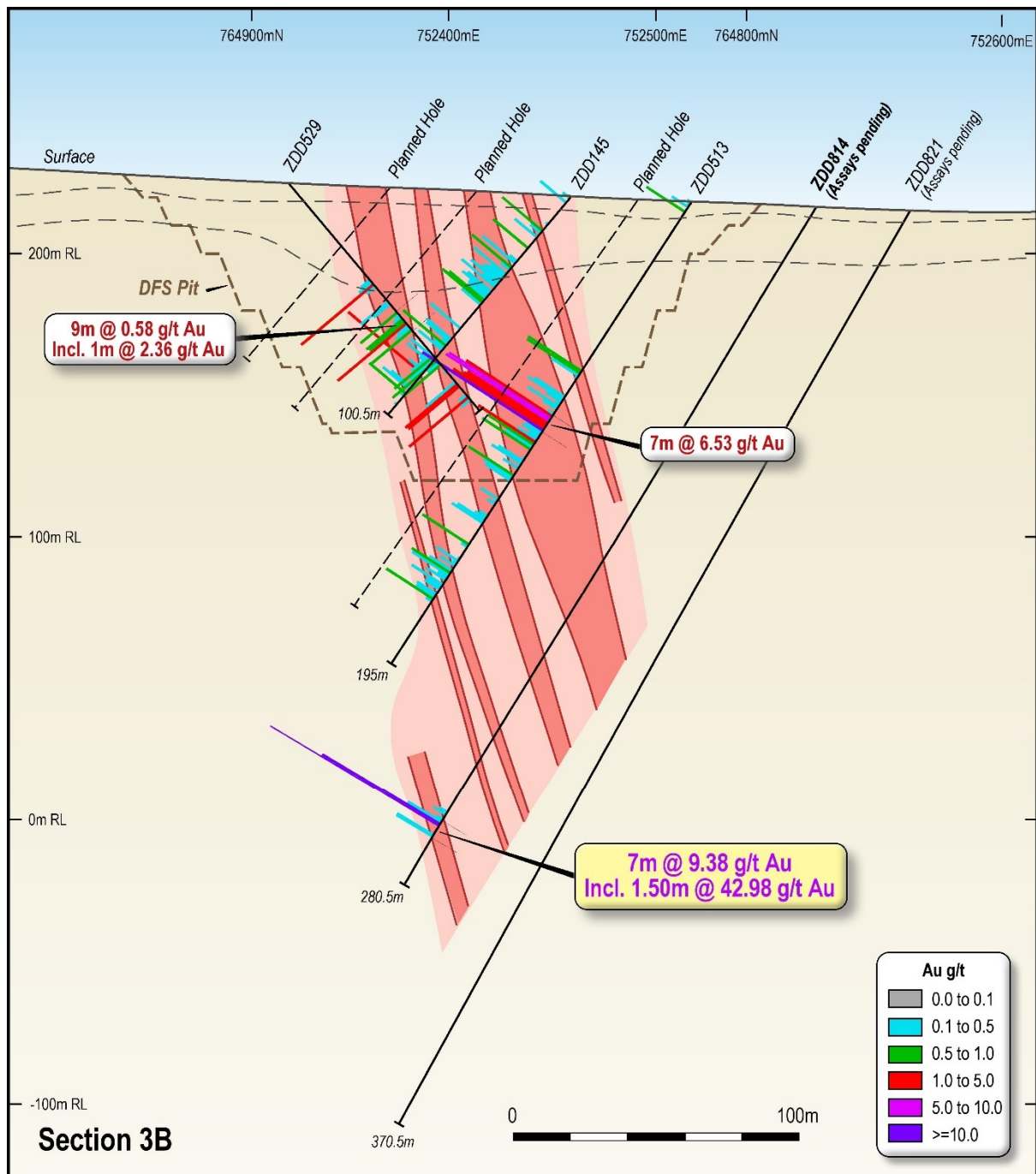
Figure 6: Oblique cross section showing latest drill results at AG (section 3B +/-25m)
