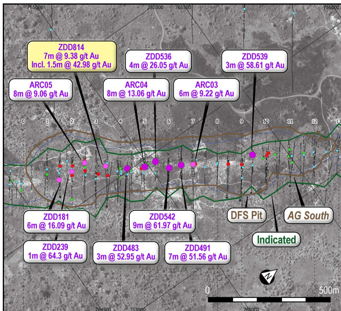
Figure 4: Plan view showing latest drill results at AG South
