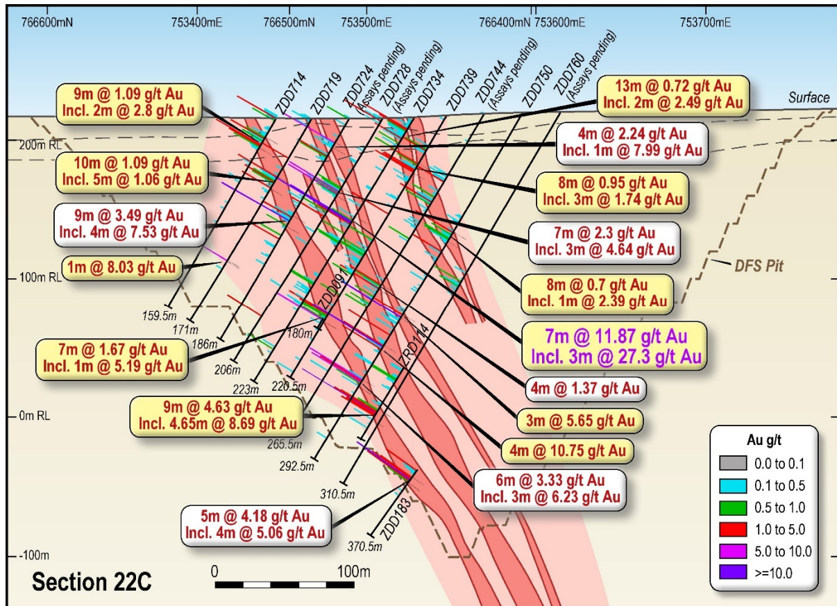
Figure 5: Oblique cross section showing latest drill results at AG (section 22C +/-12.5m)
