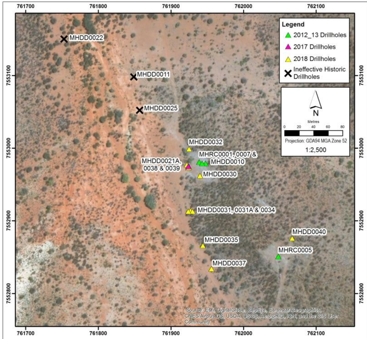
Figure 3 Drill hole location plan for the EM1 Prospect at Mt Hardy.
