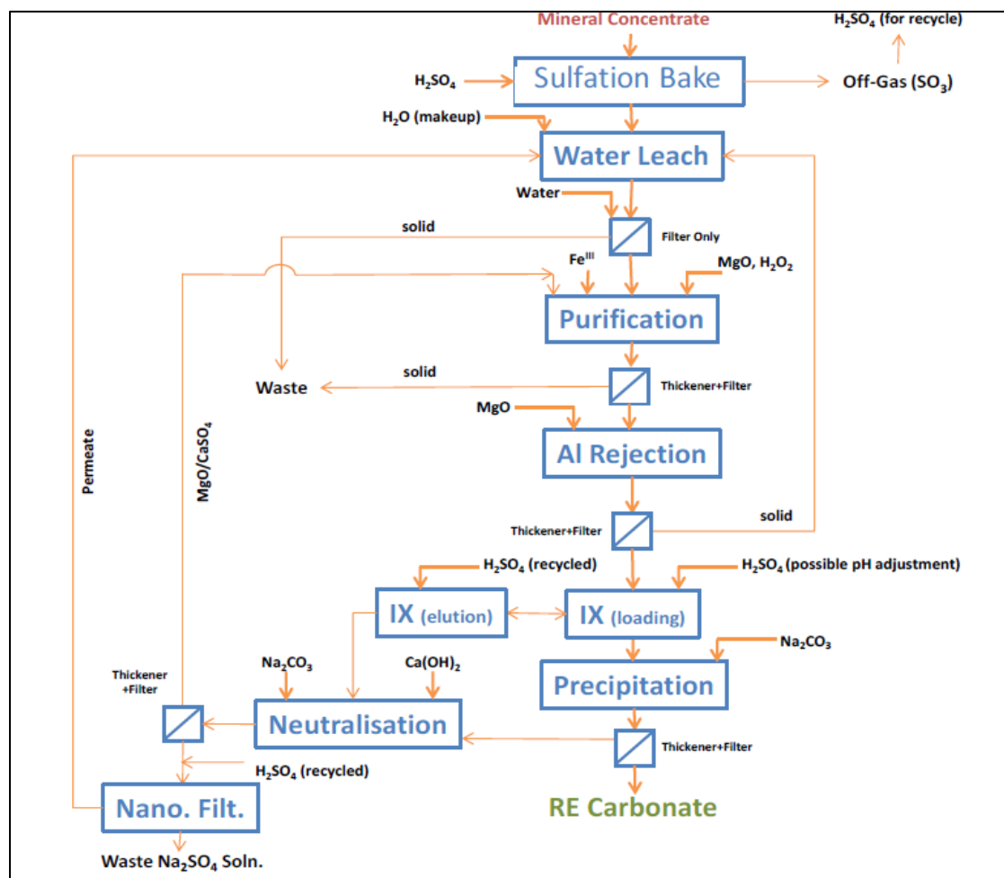
Figure 10: ANSTO pilot flowsheet
