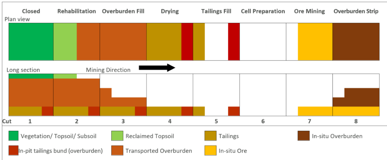
Figure 7: Schematic illustration of mining sequence including progressive backfill and rehabilitation.
